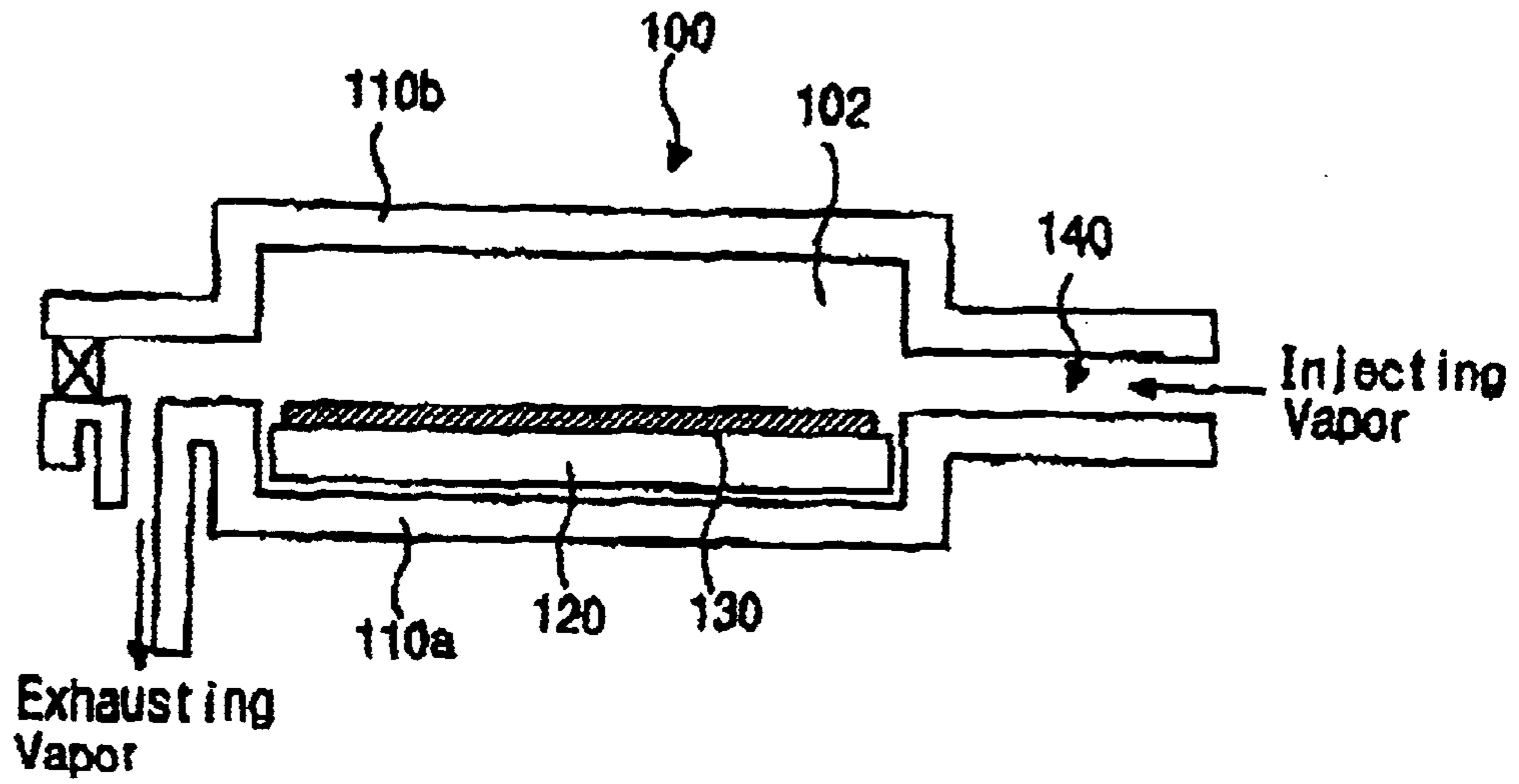
(related art) FIG. 1
