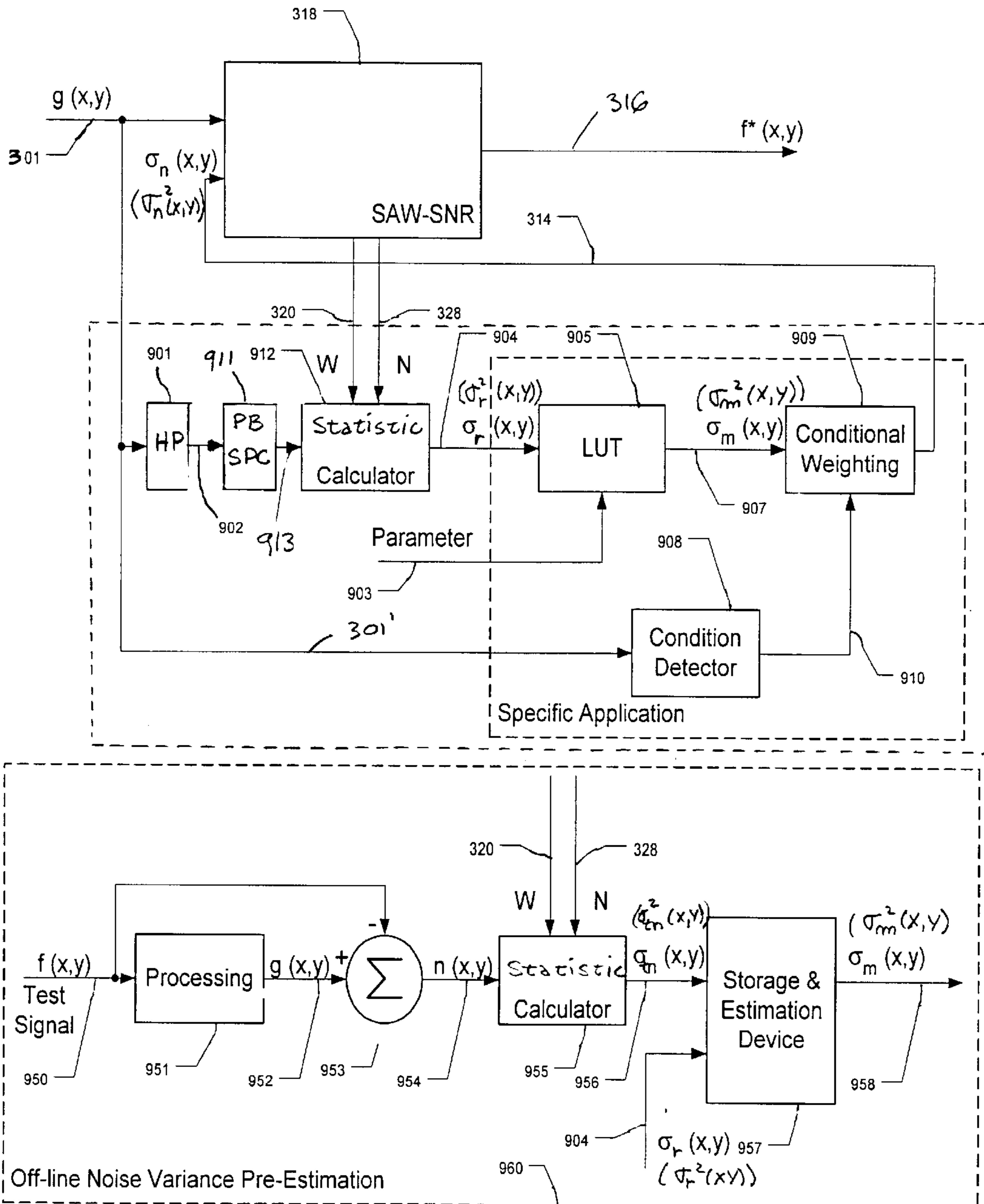
Fig.9 Proposed SAW-SNR with Controllable Noise statistic Estimator Block Diagram (Third Preferred Embodiment)
