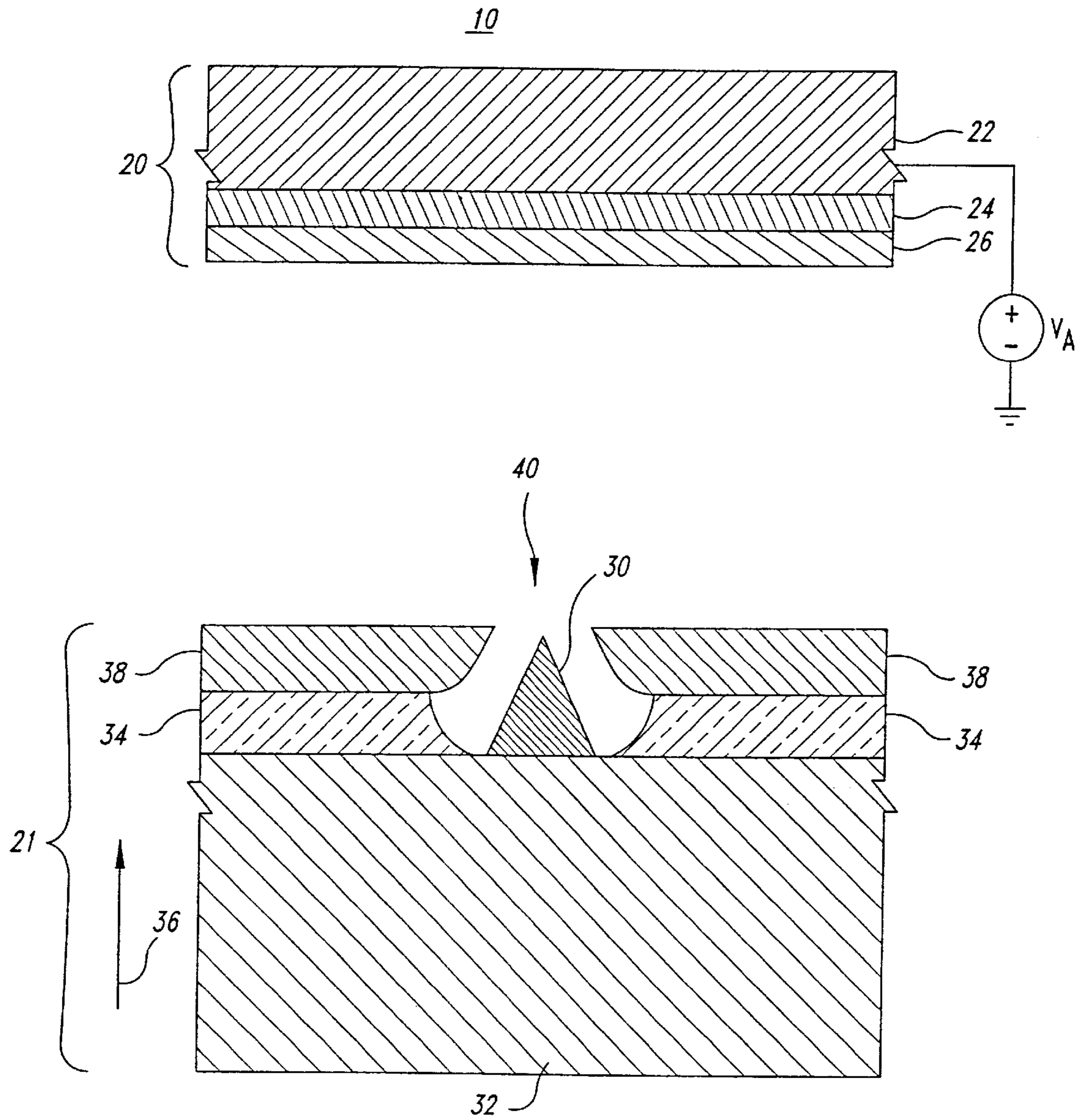
Fig. 1 (PRIOR ART)
