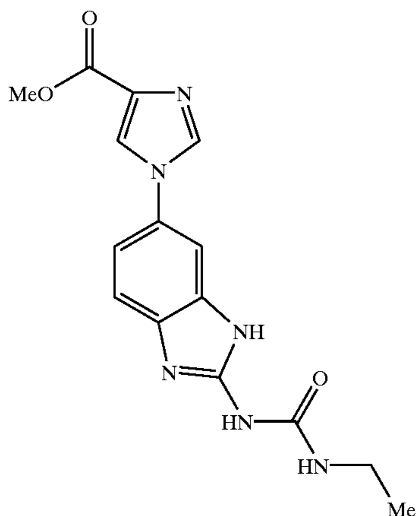
Example 8
