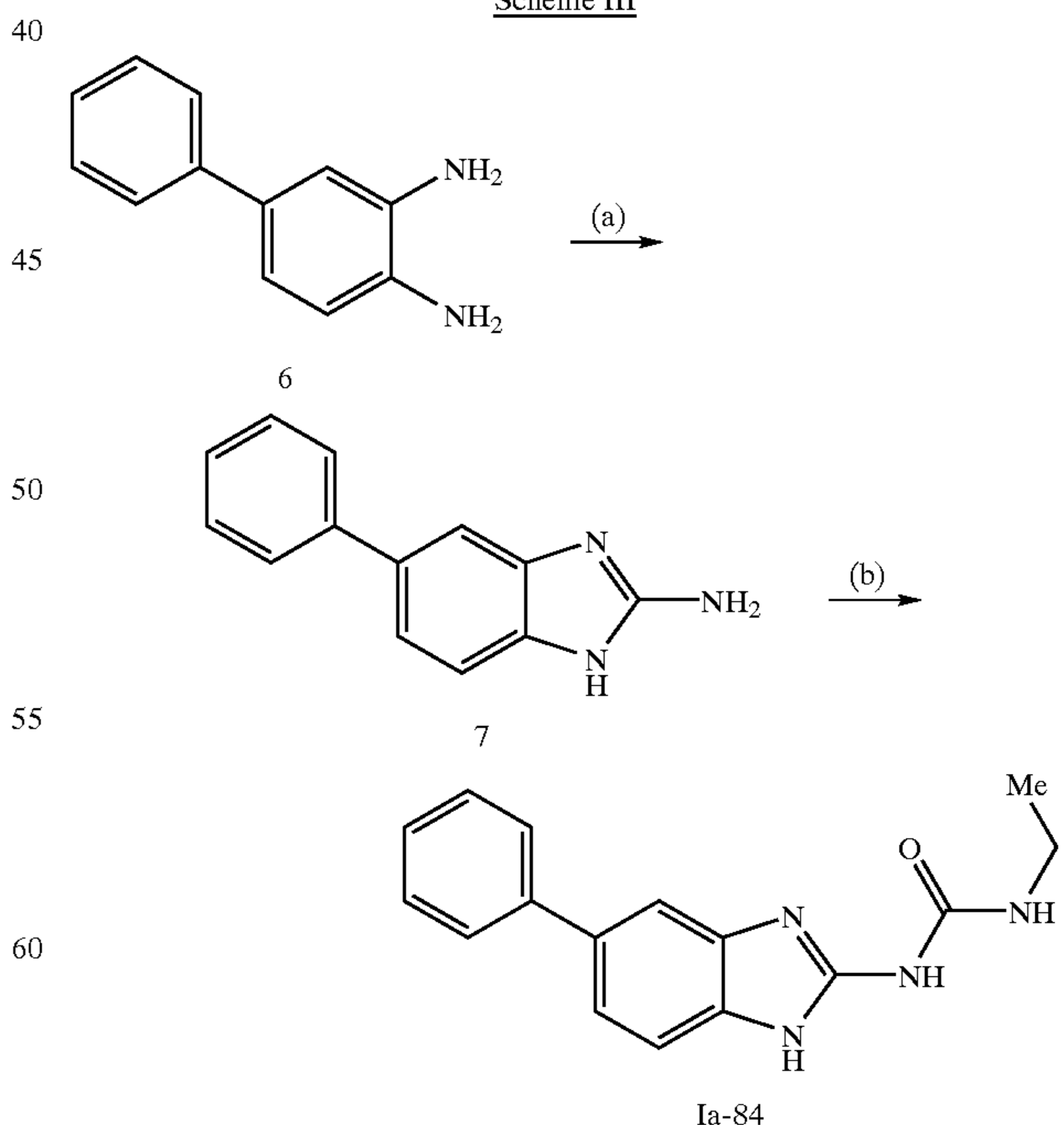
Scheme III
