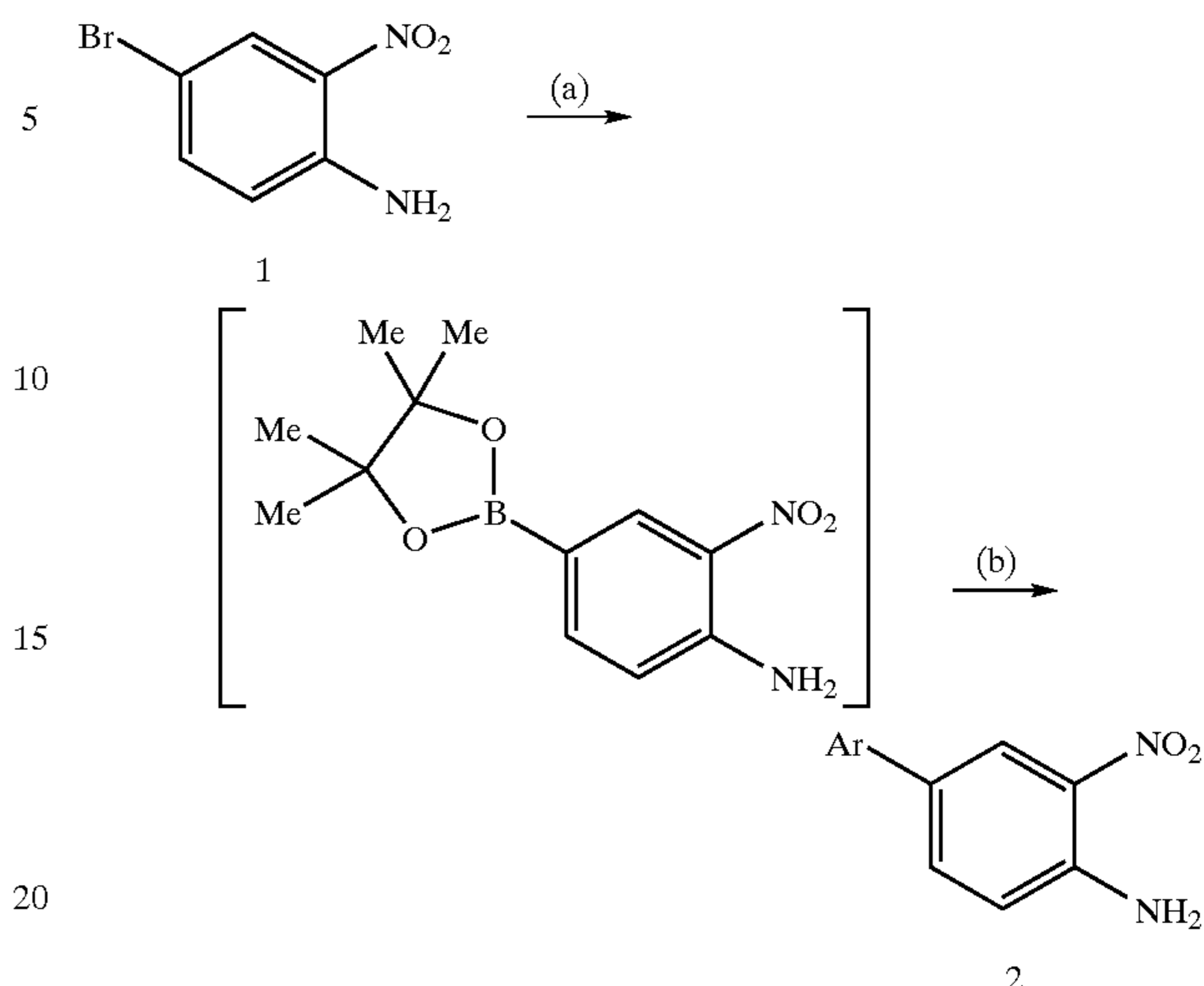
Scheme II
