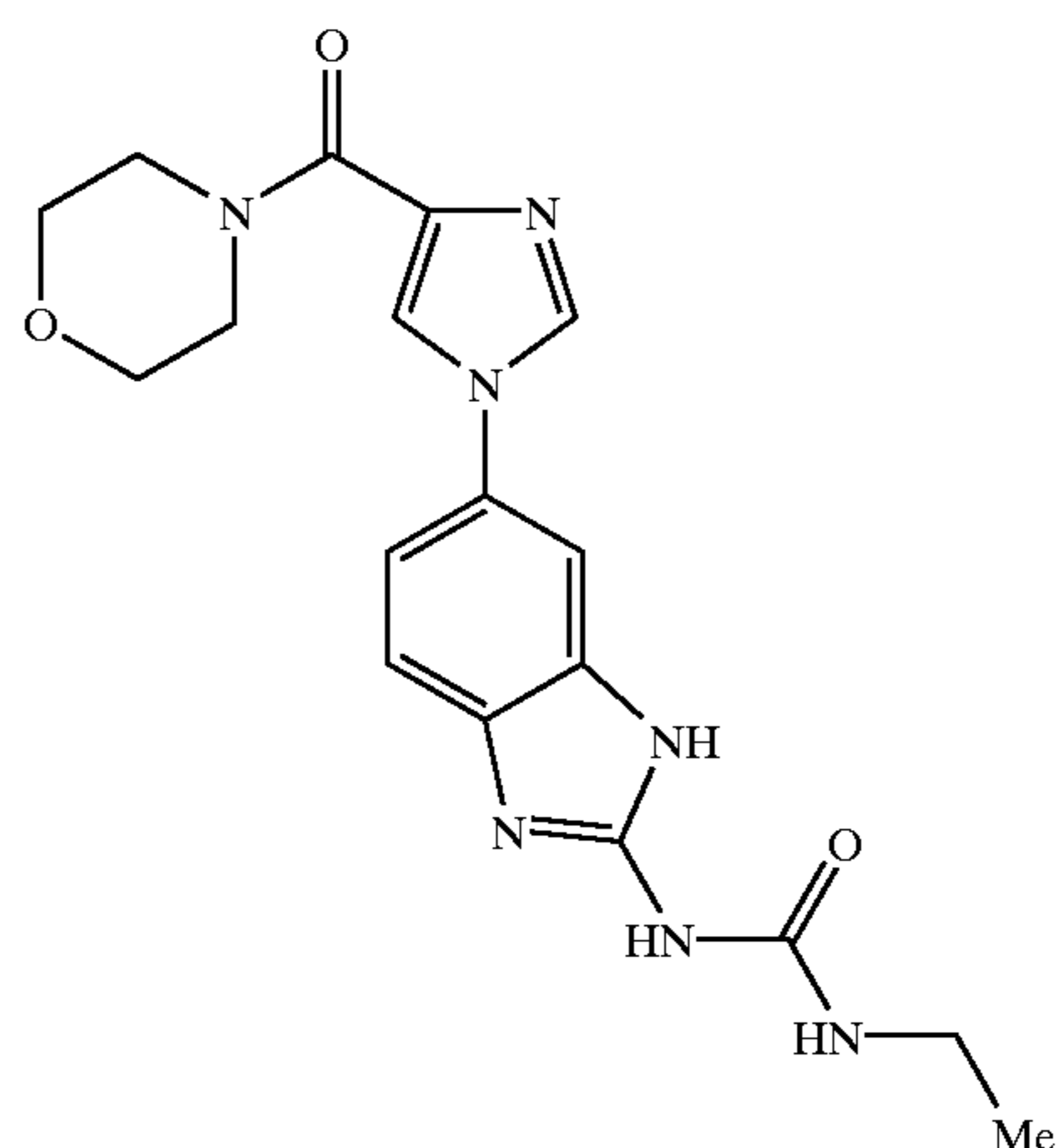
Example 10
