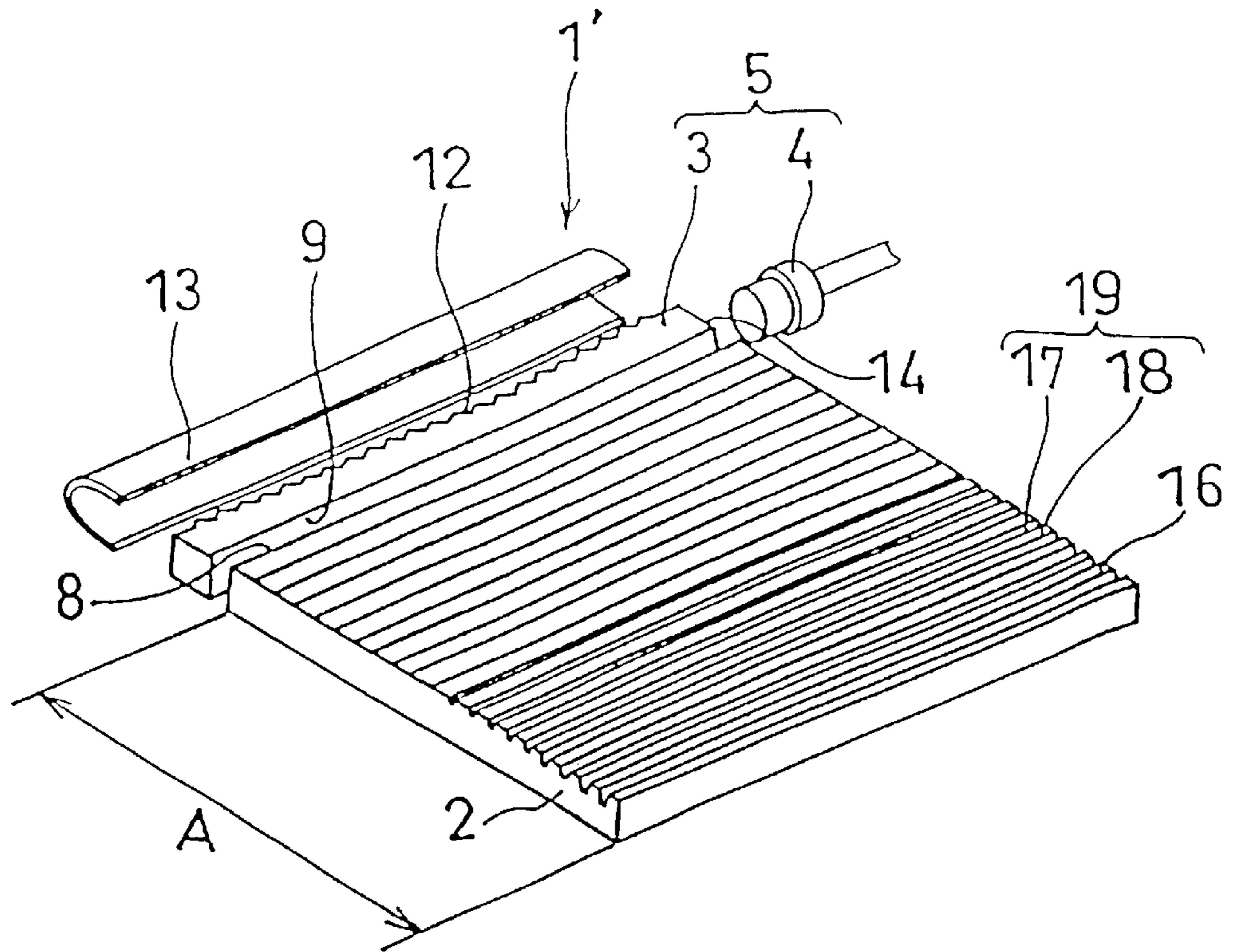
Fig. 7 PRIOR ART
