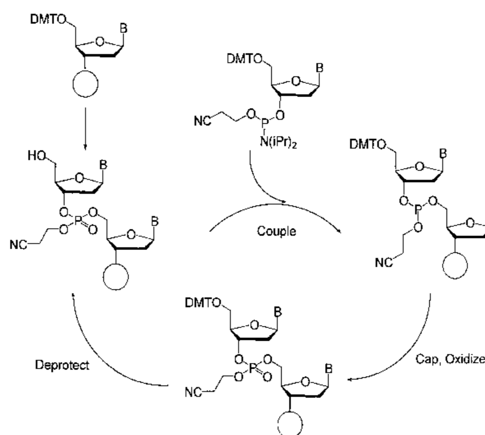
3'-5' Synthesis With DMT Protection
