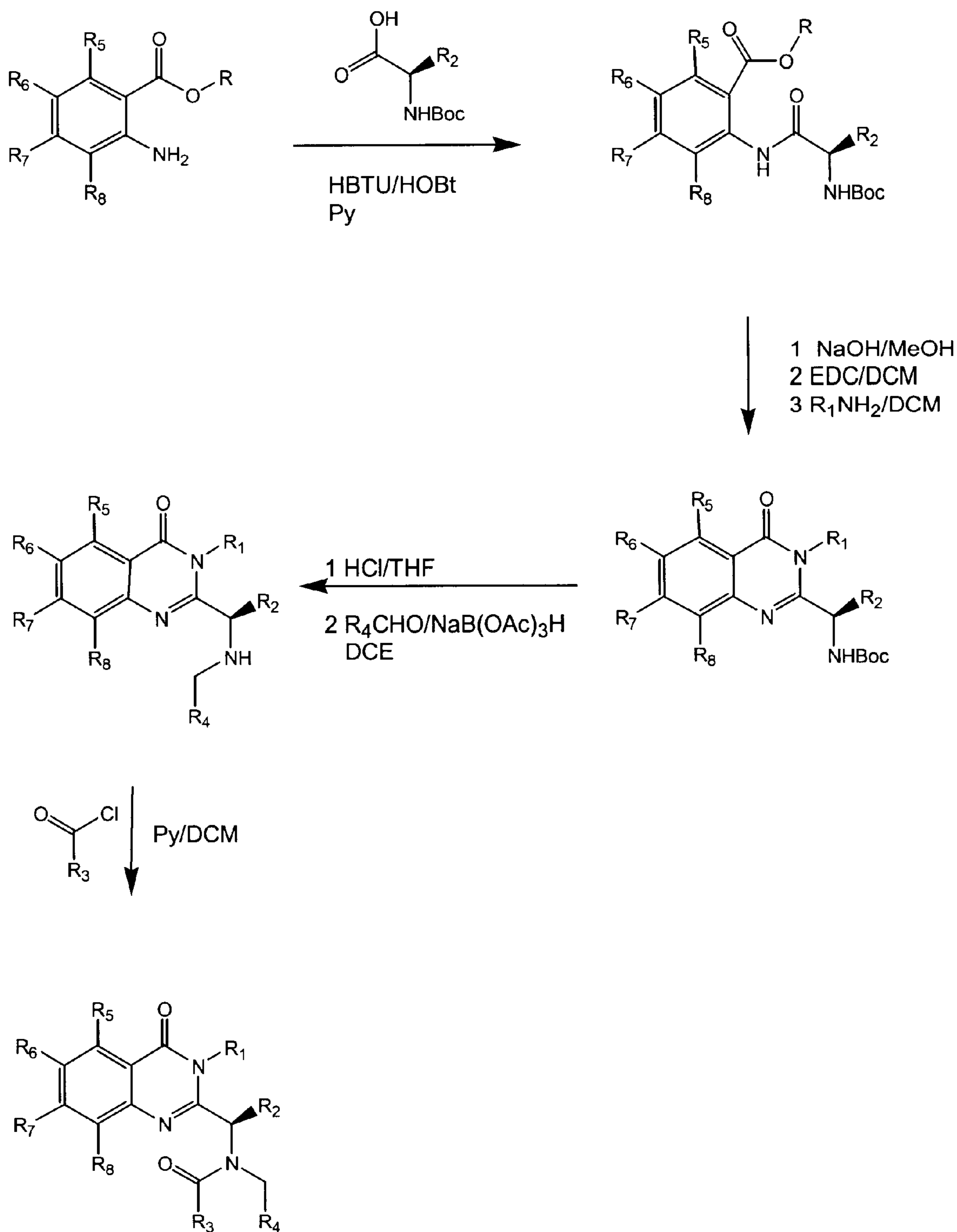
Figure 4: Asymmetric Synthesis
