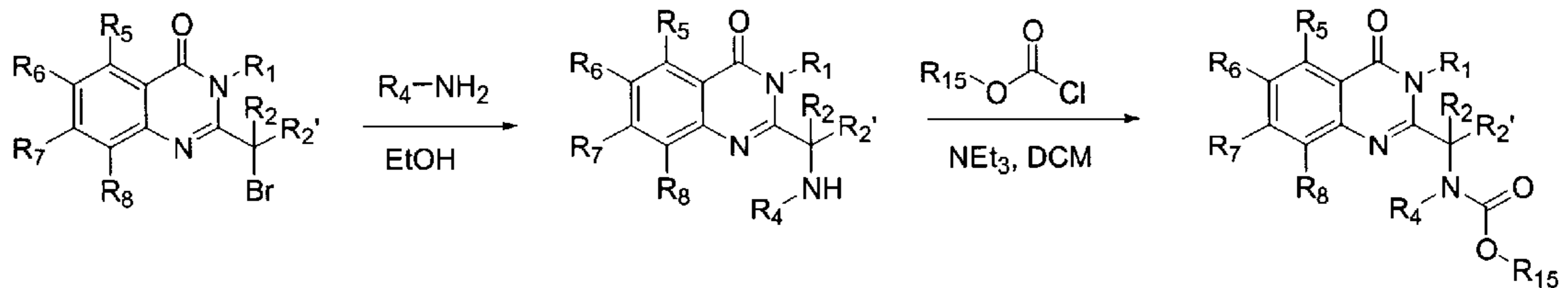
Figure 5c: Urea Synthesis
