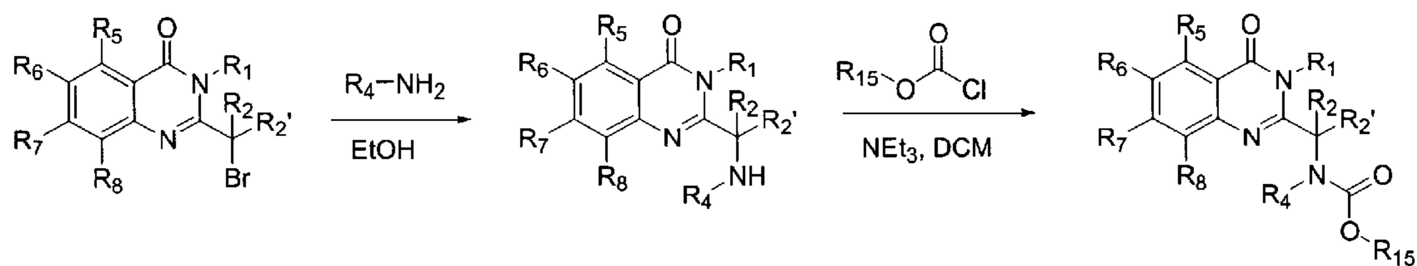
Figure 5c: Urea Synthesis
