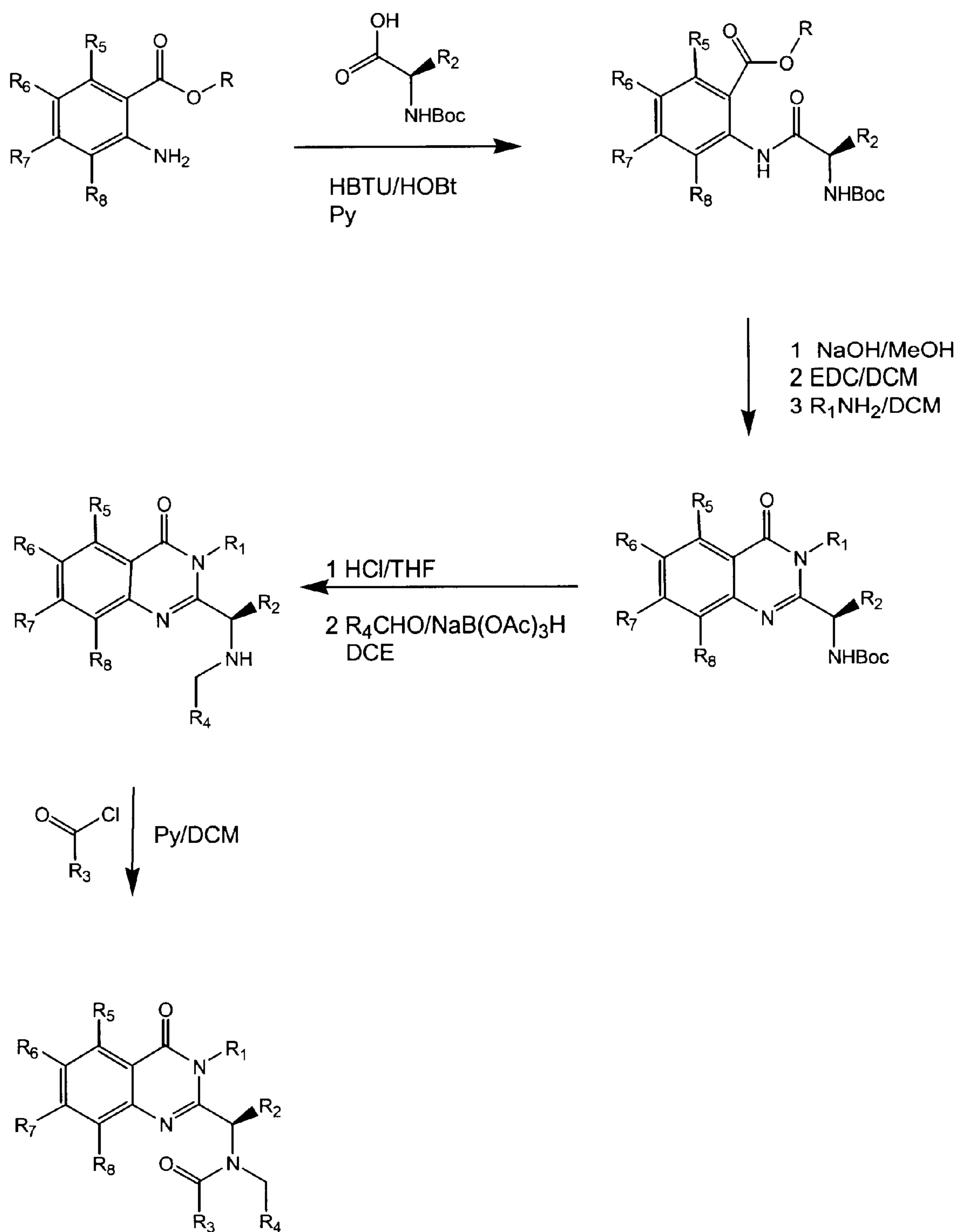
Figure 4: Asymmetric Synthesis
