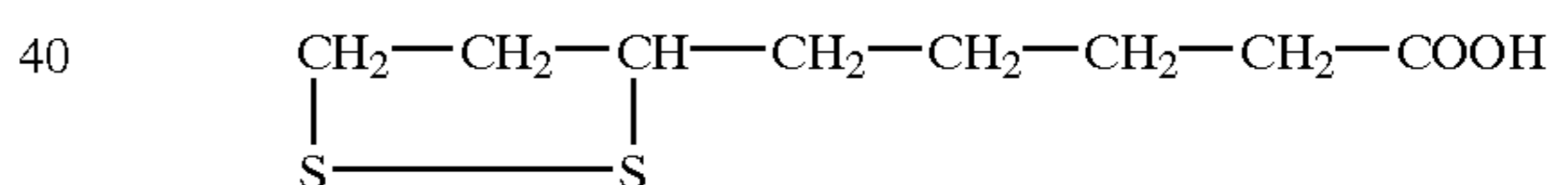
Thioctic acid or α-lipoic acid (TA)
