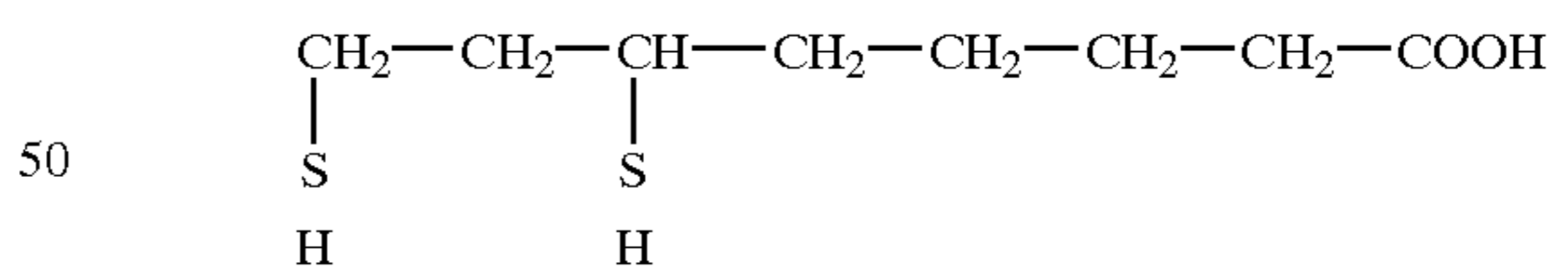
Dihydrolipoic acid (DHL)
