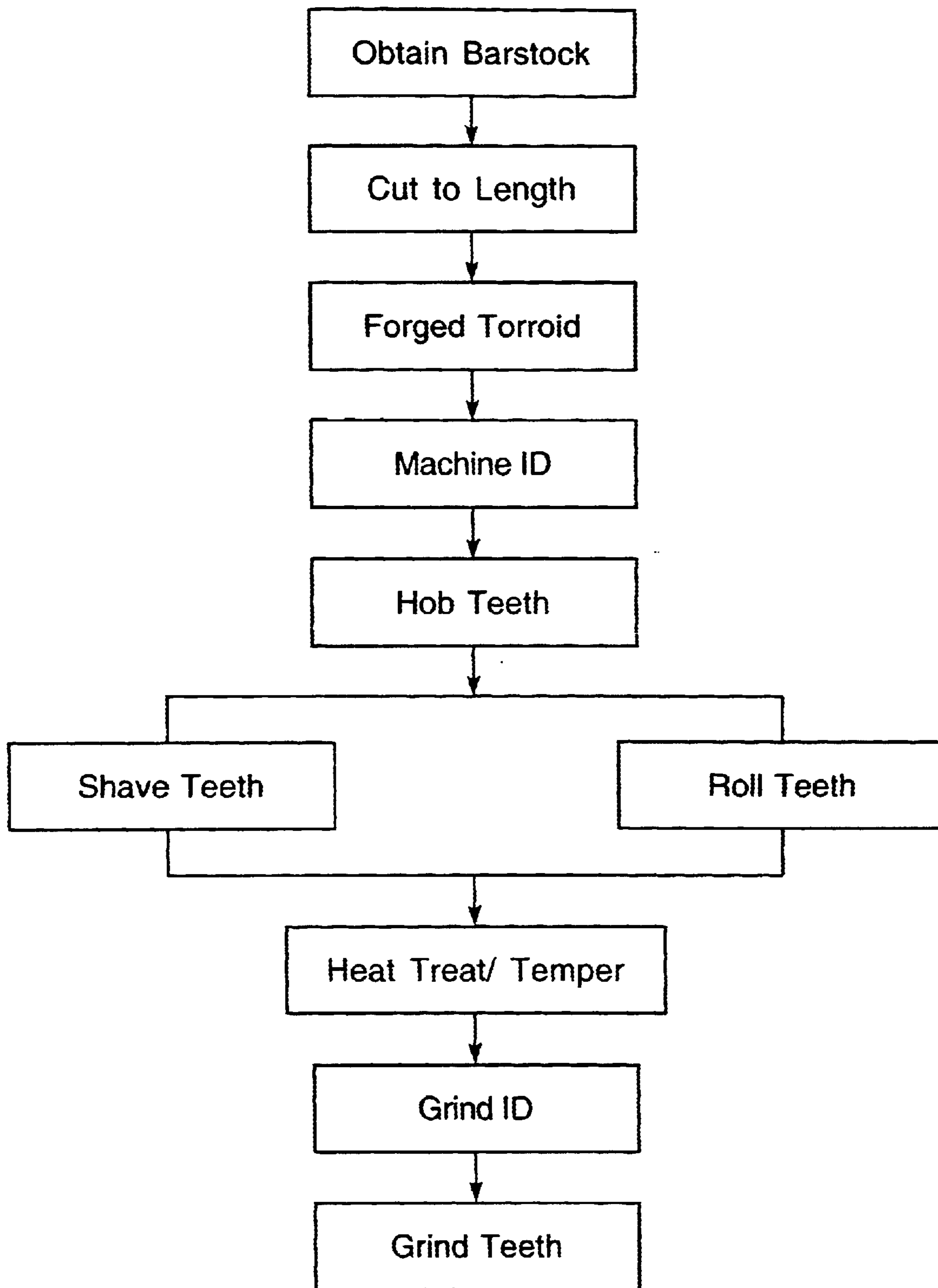
FIG. 1 Prior Art
