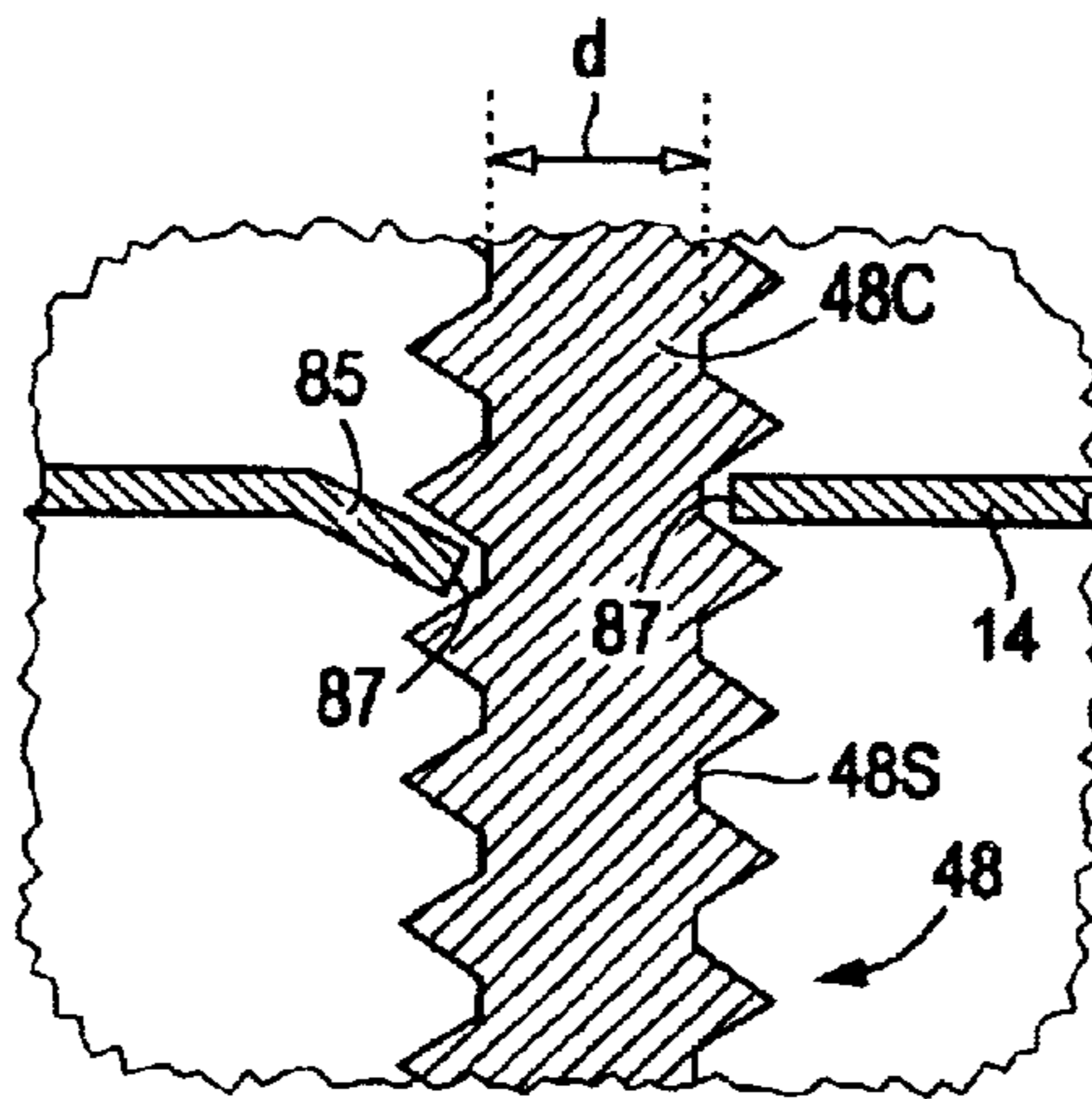
FIG. 18 PRIOR ART
