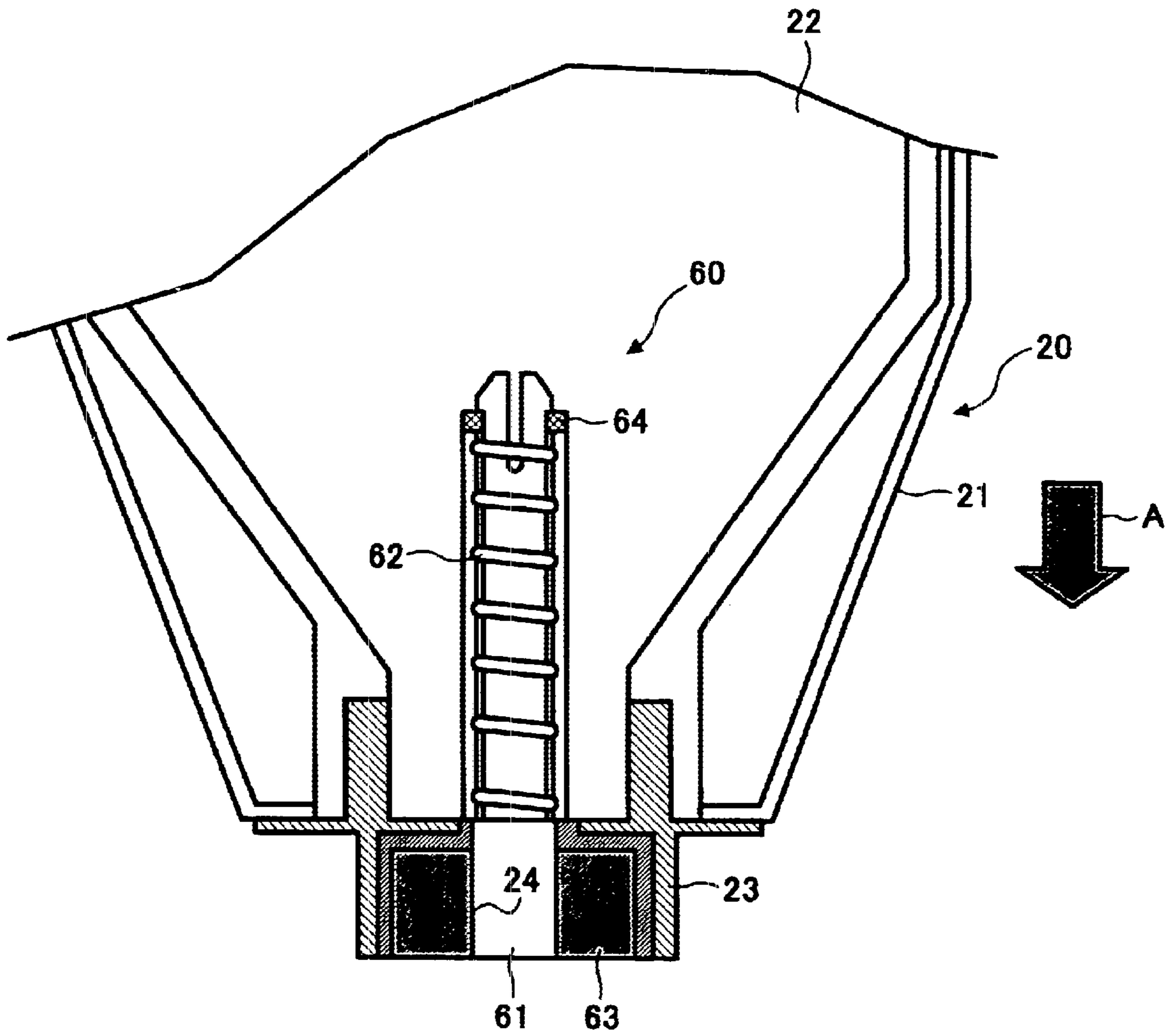
FIG. 5 PRIOR ART
