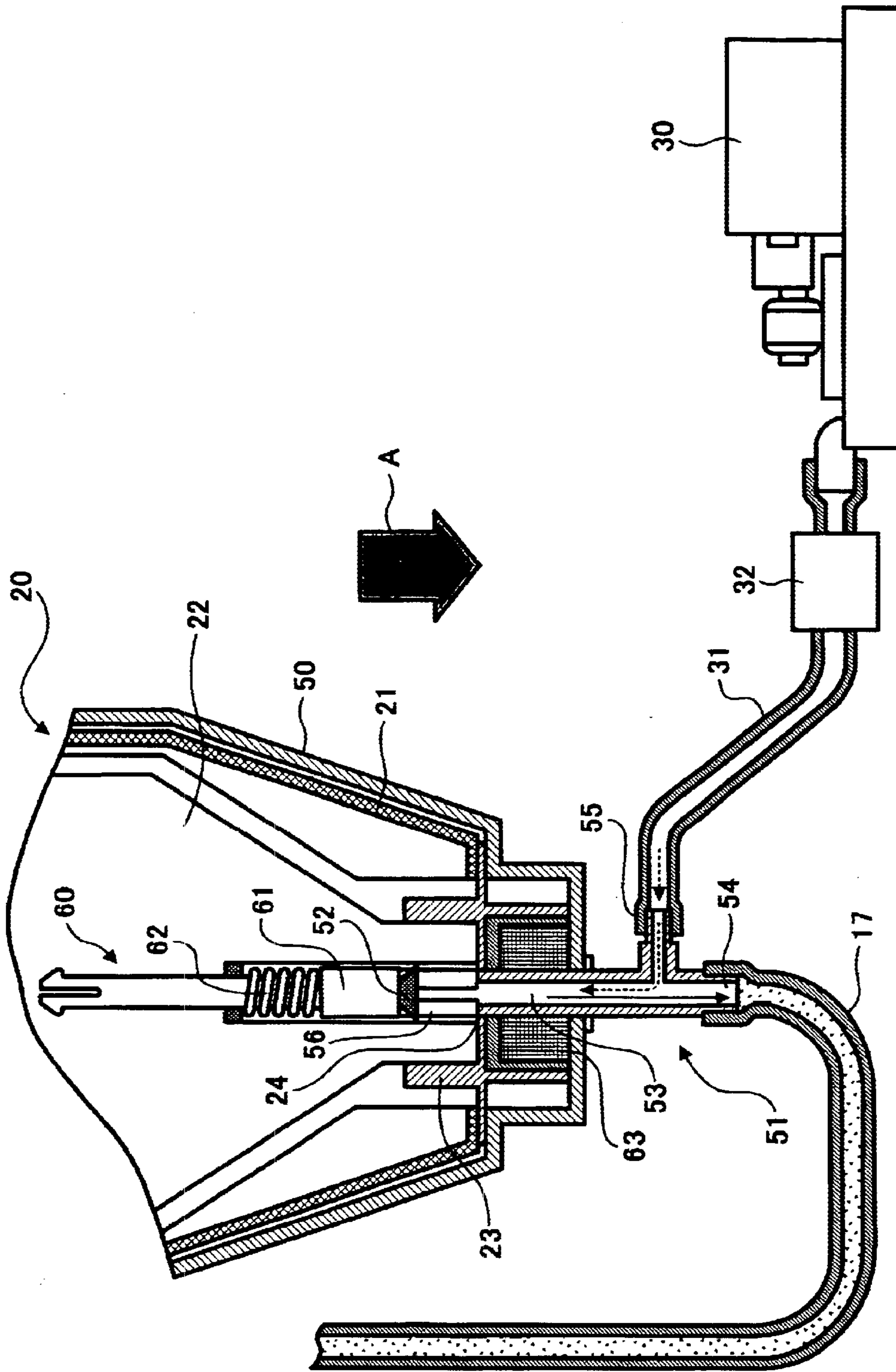
FIG. 6 PRIOR ART
