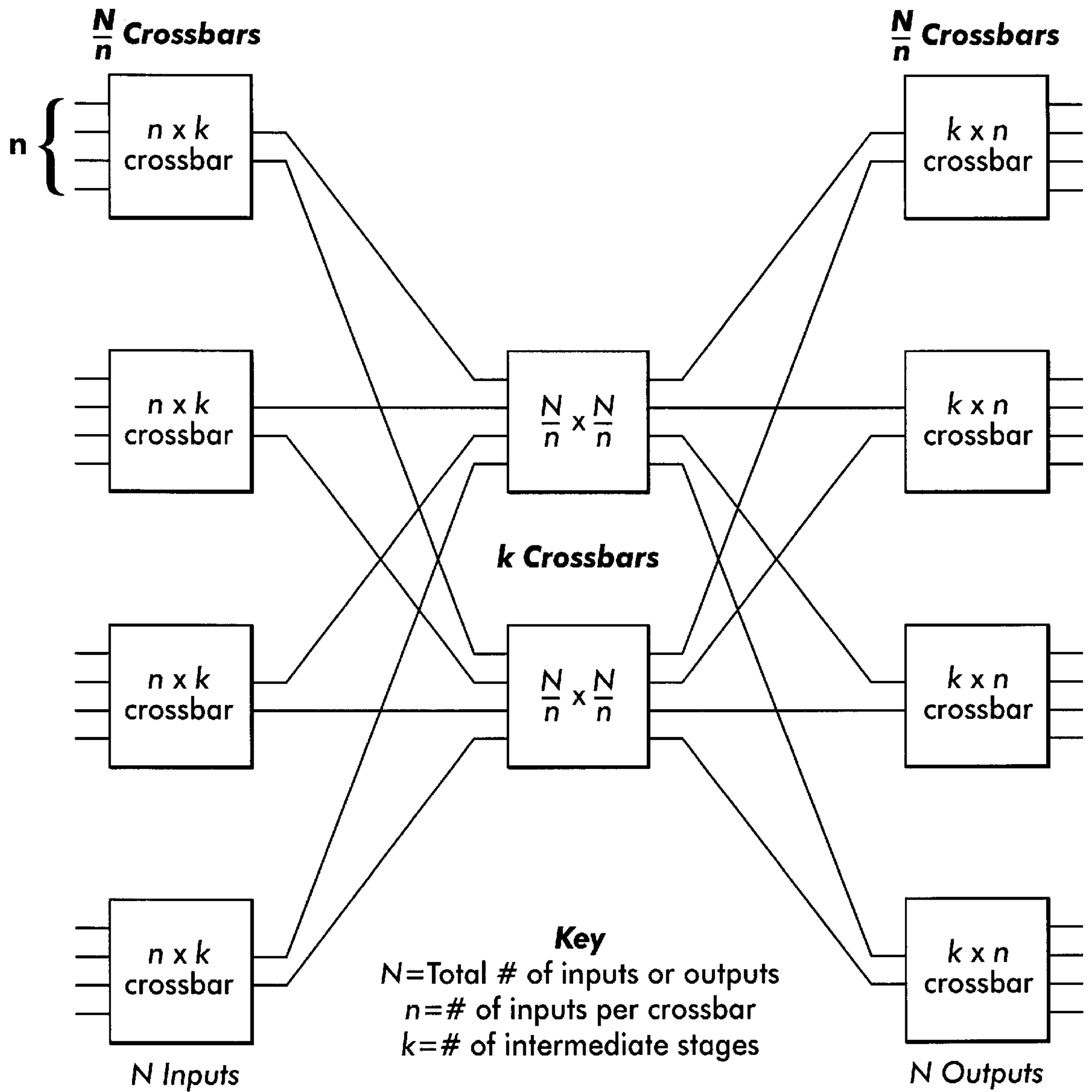
FIG. 10 PRIOR ART
