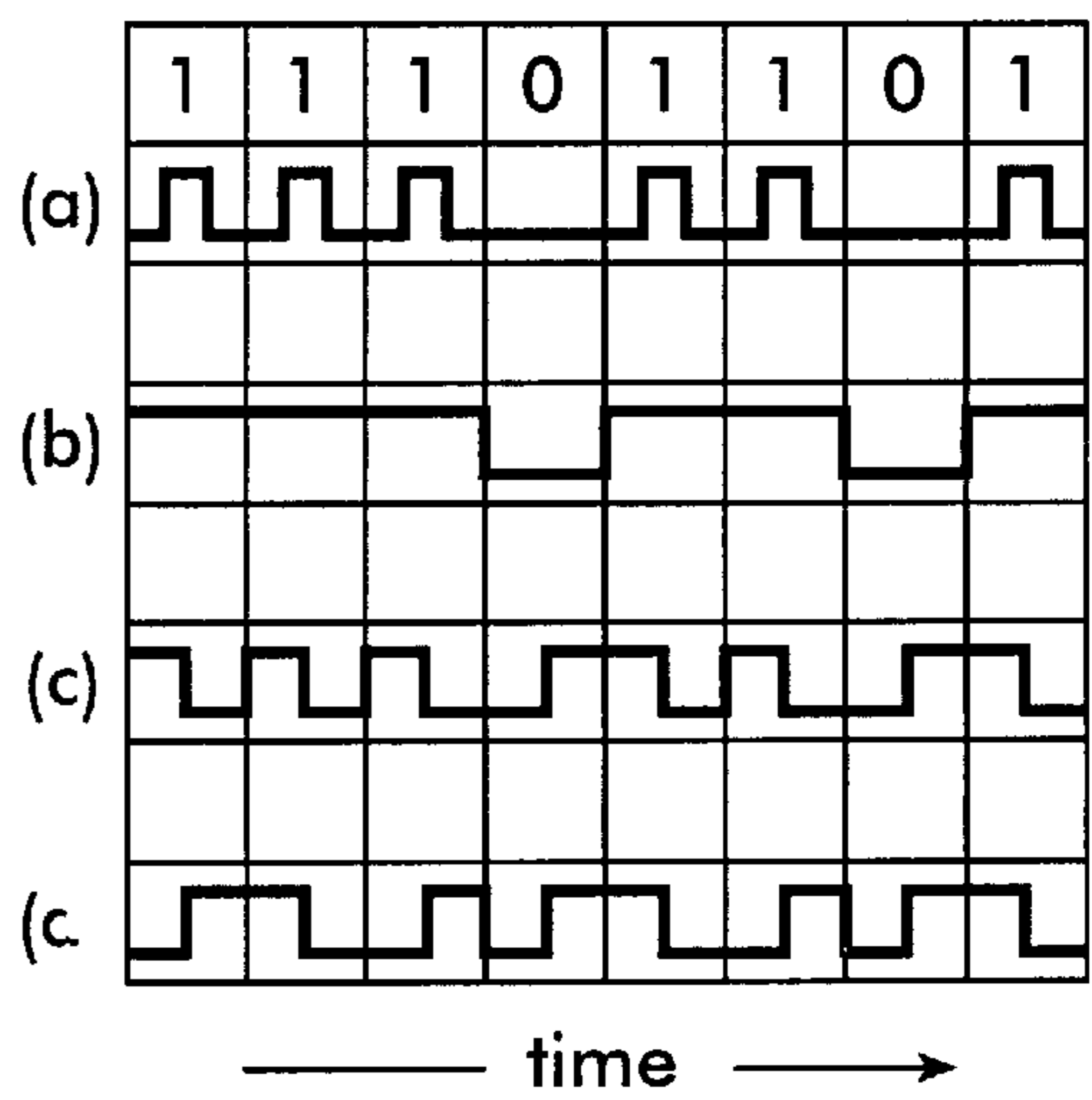
FIG. 3 PRIOR ART
