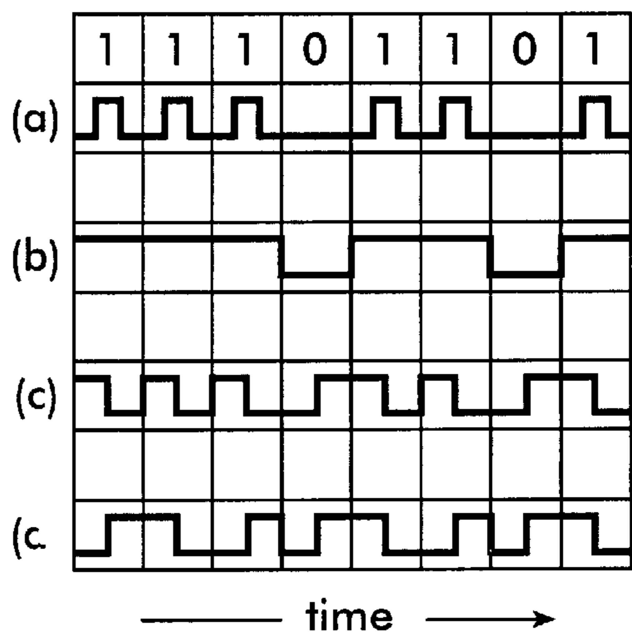
FIG. 3 PRIOR ART
