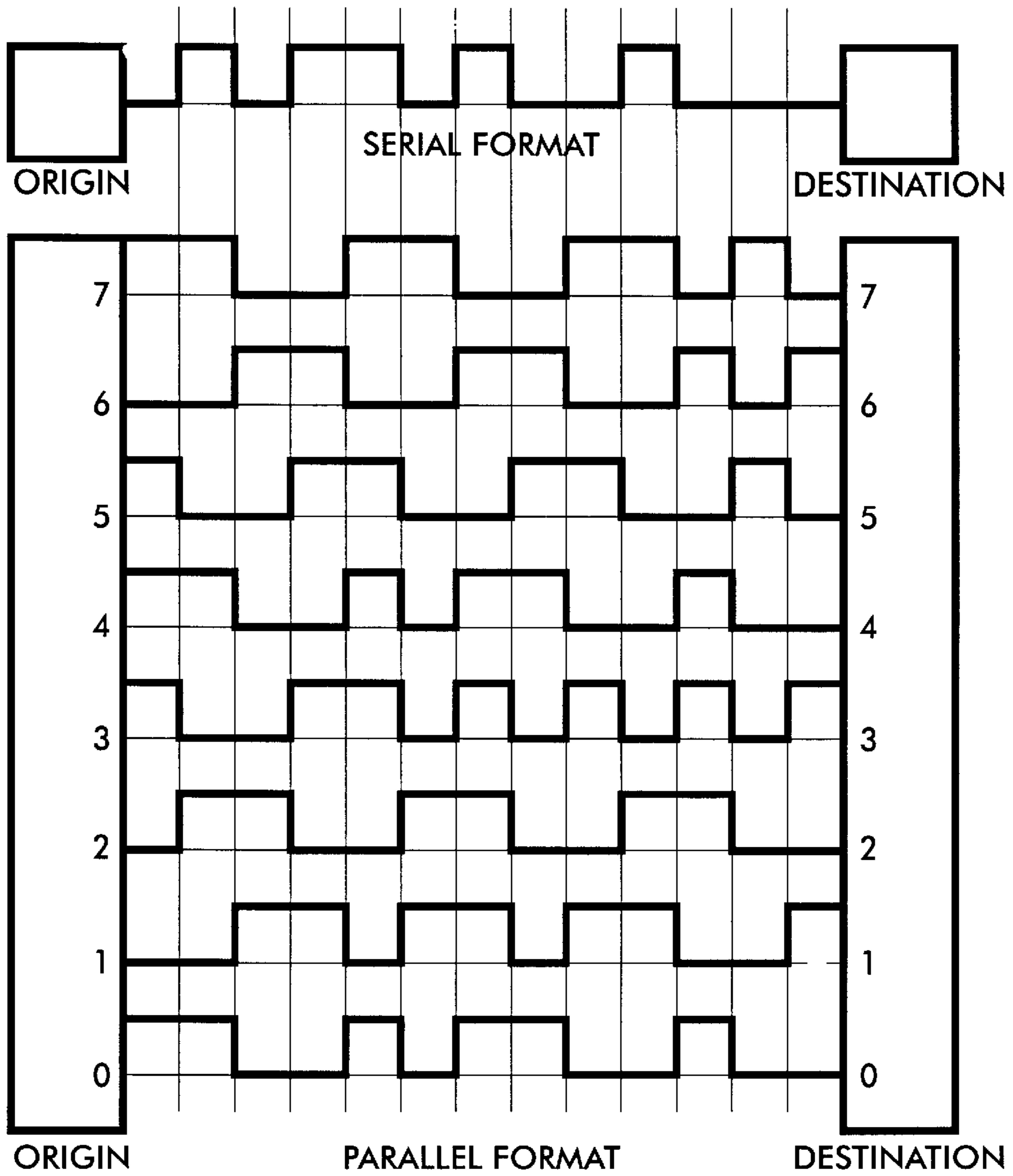
FIG. 4 PRIOR ART
