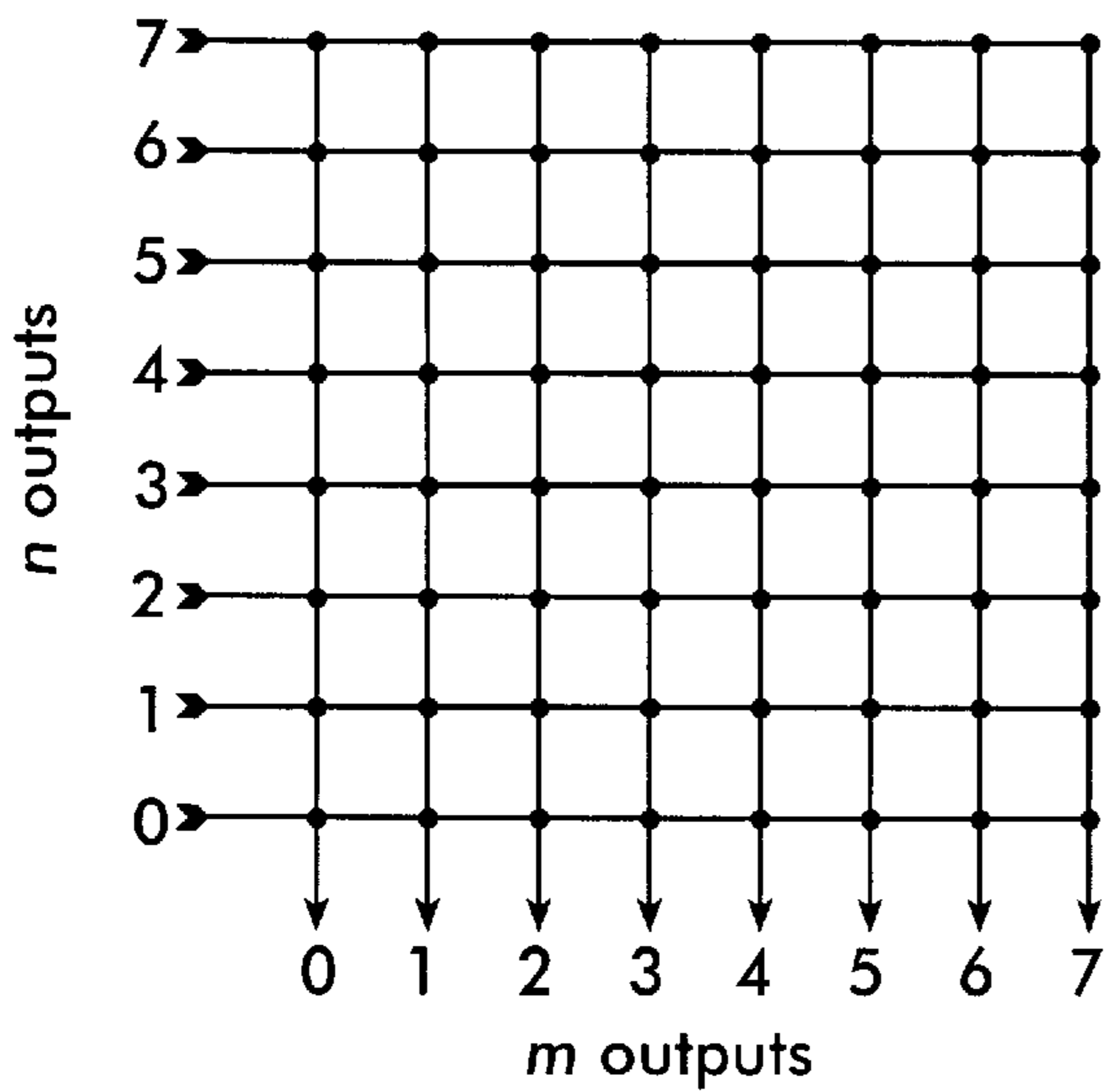
FIG. 7 PRIOR ART
