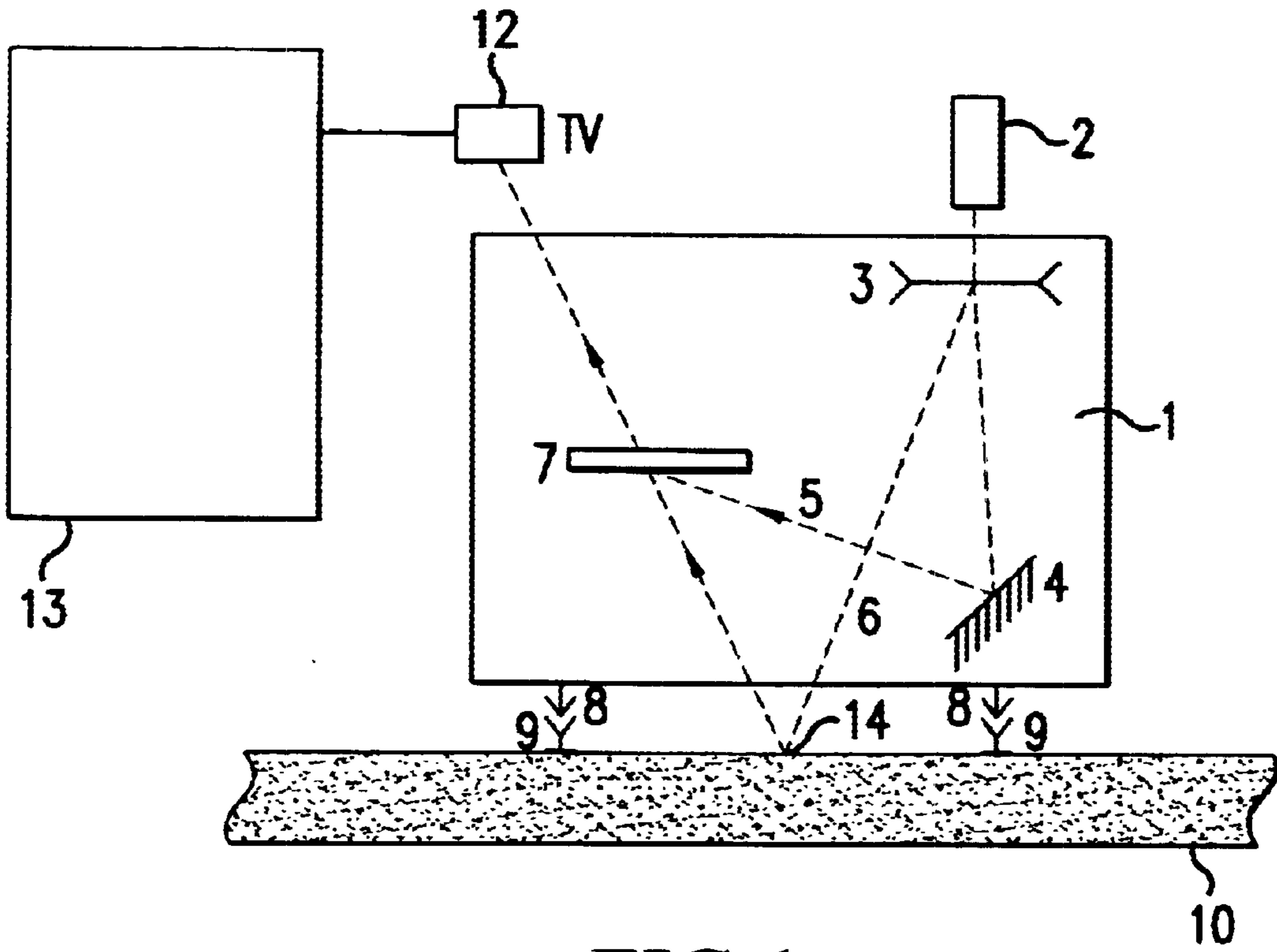
FIG. 1 BACKGROUND ART
