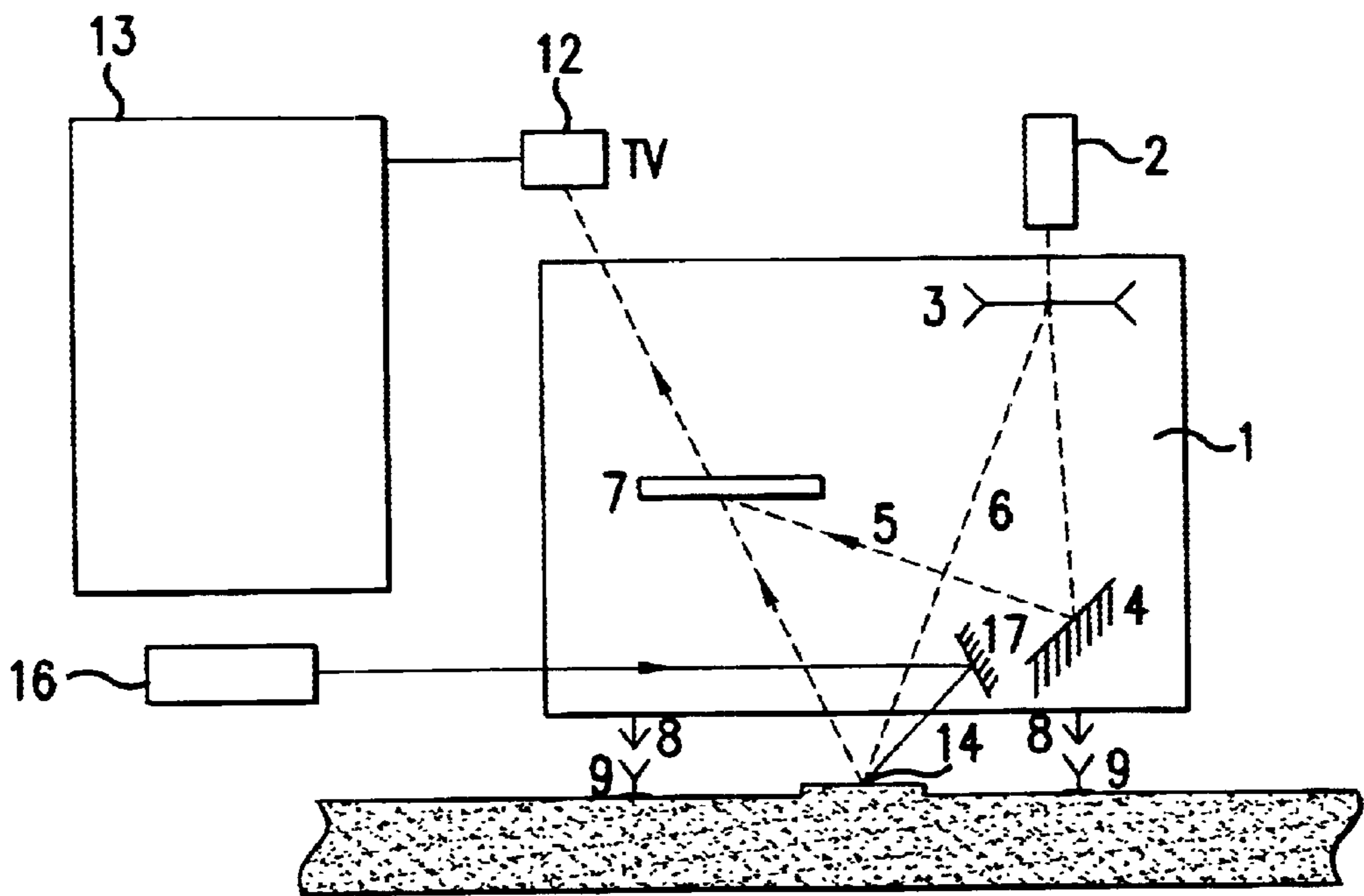
FIG. 5 BACKGROUND ART
