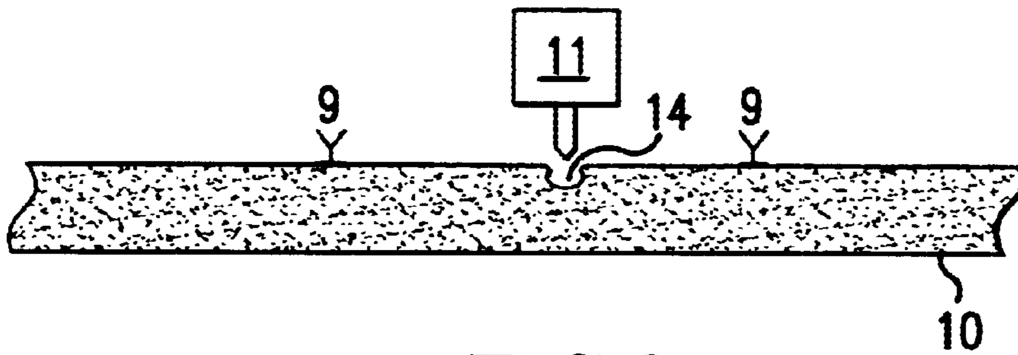
FIG. 2 BACKGROUND ART
