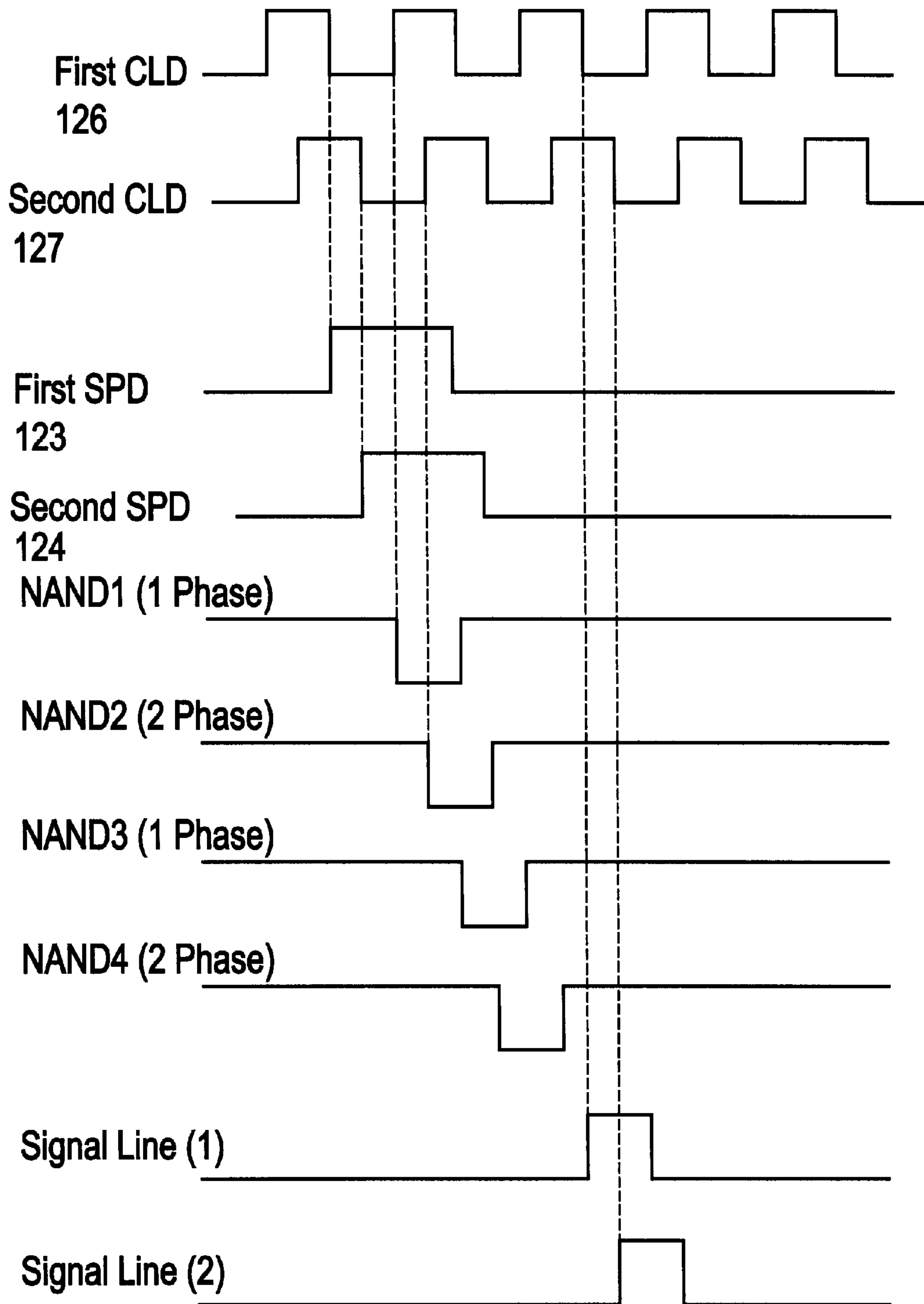
Timing Chart of Source Driver Circuit
