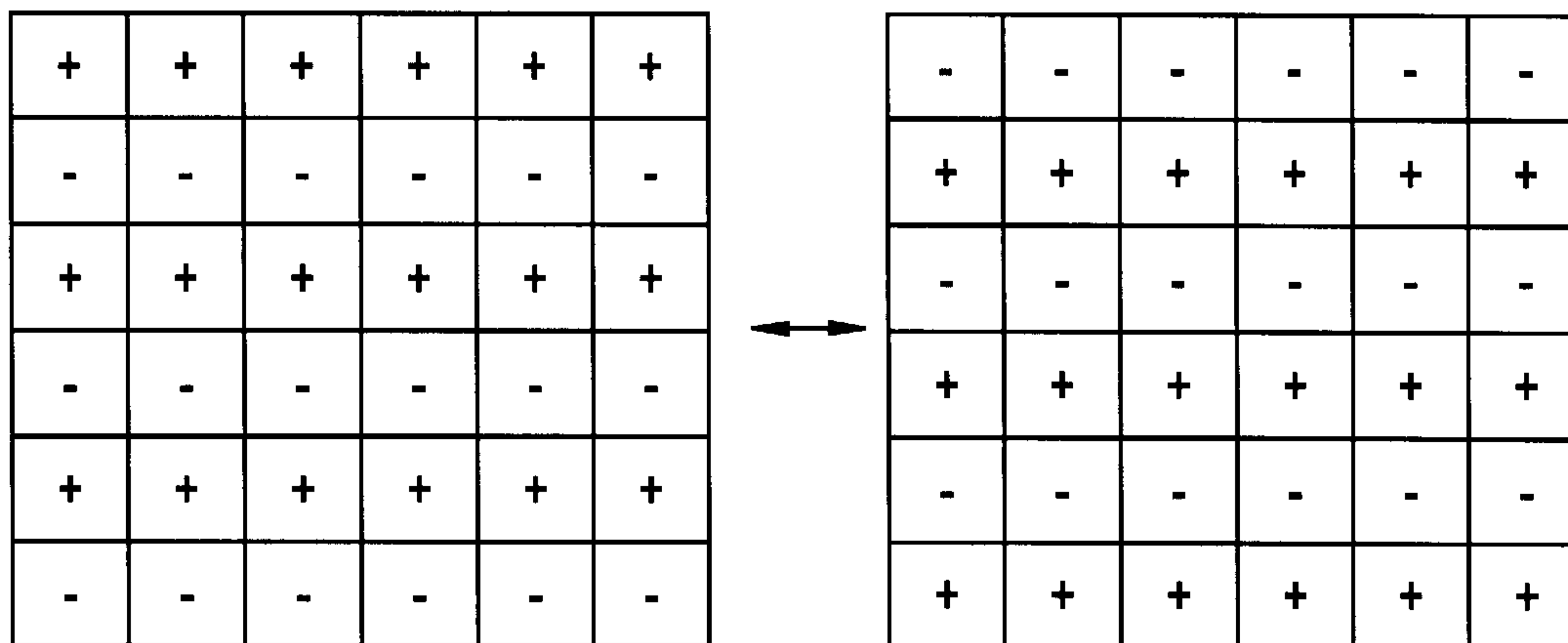
Gate Line Inversion
