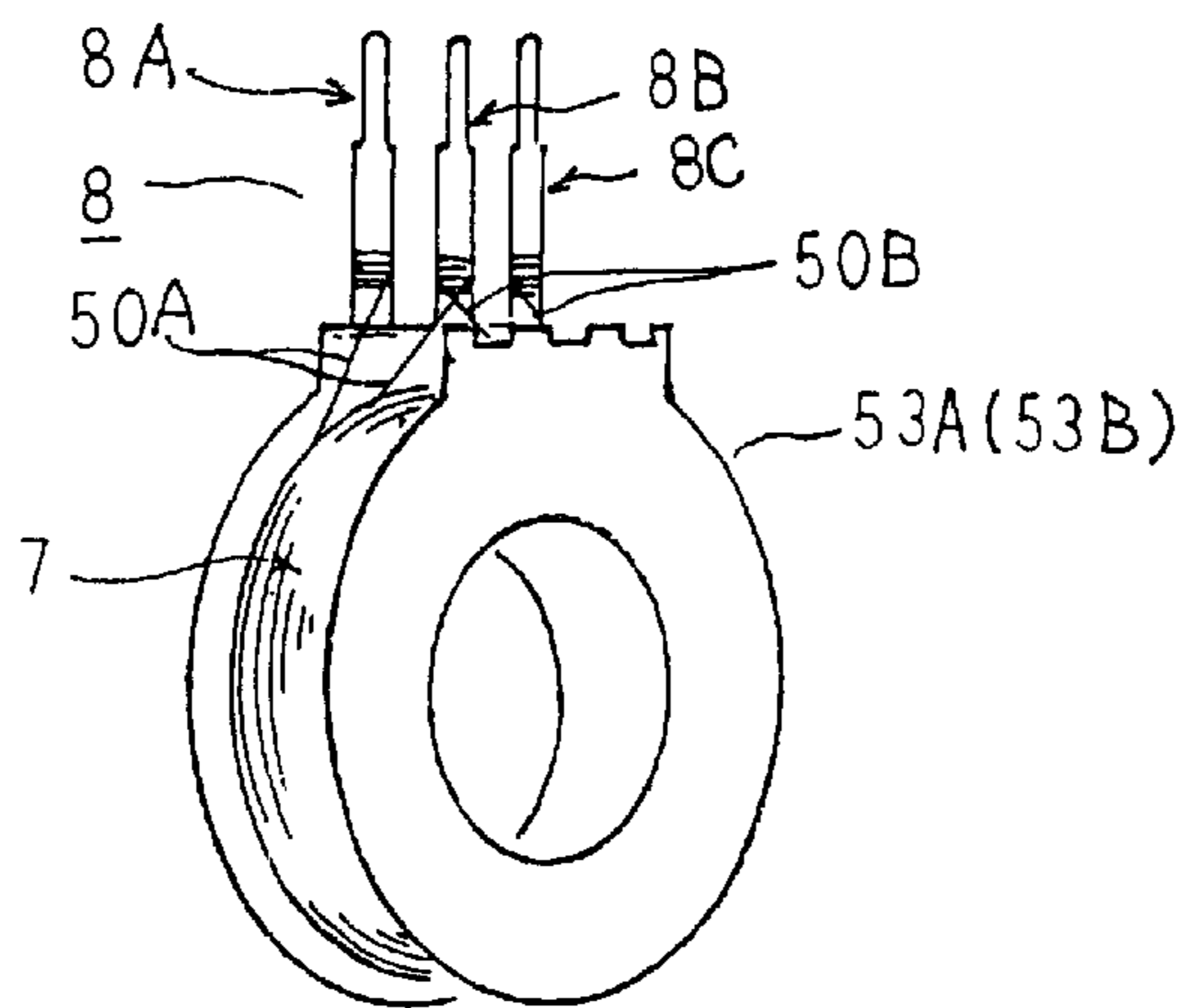
FIG. 14 PRIOR ART
