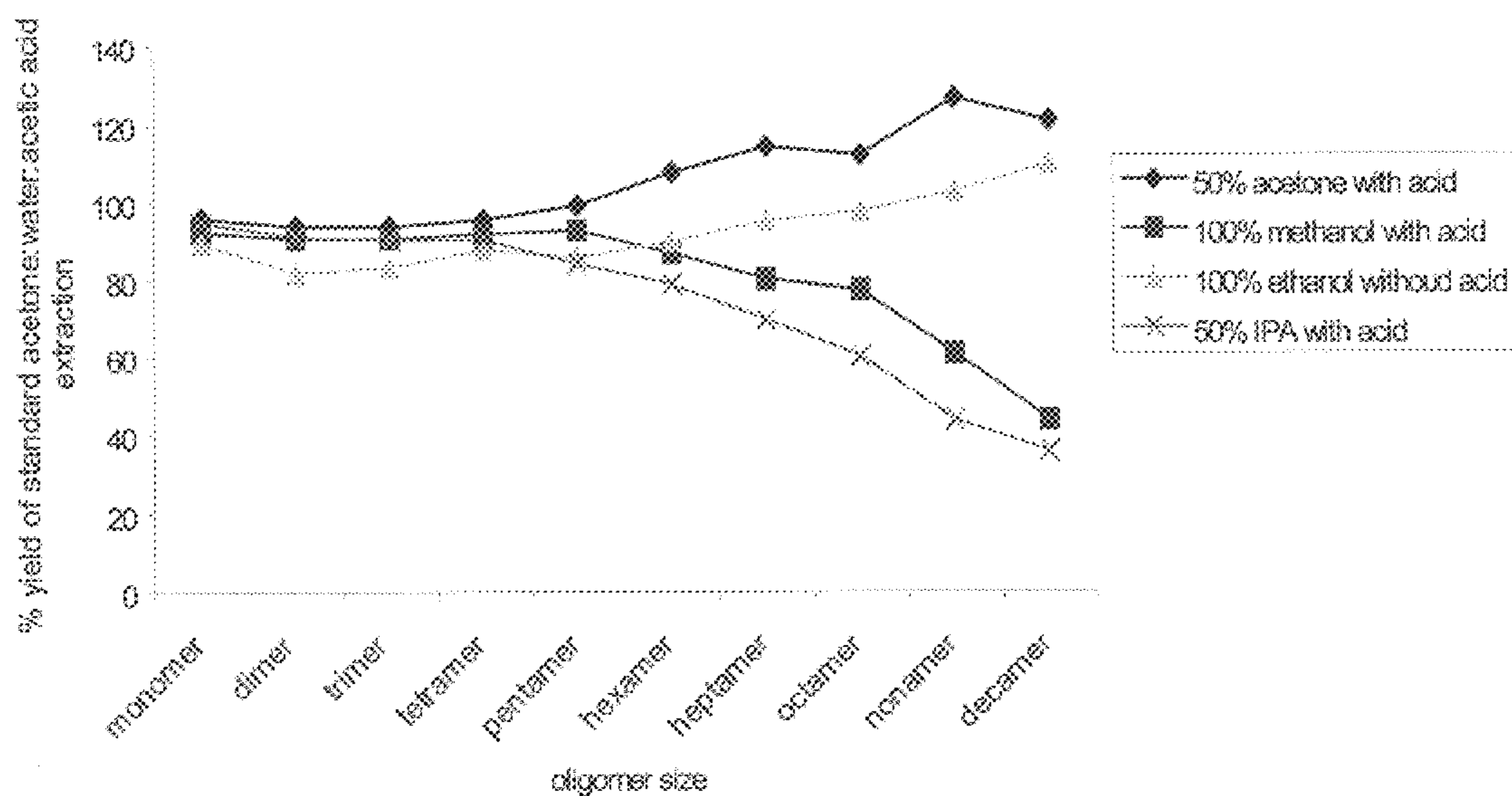
Figure 2 Graph showing that acetone and ethanol are most effective for extracting the higher oligomers at 50°C
