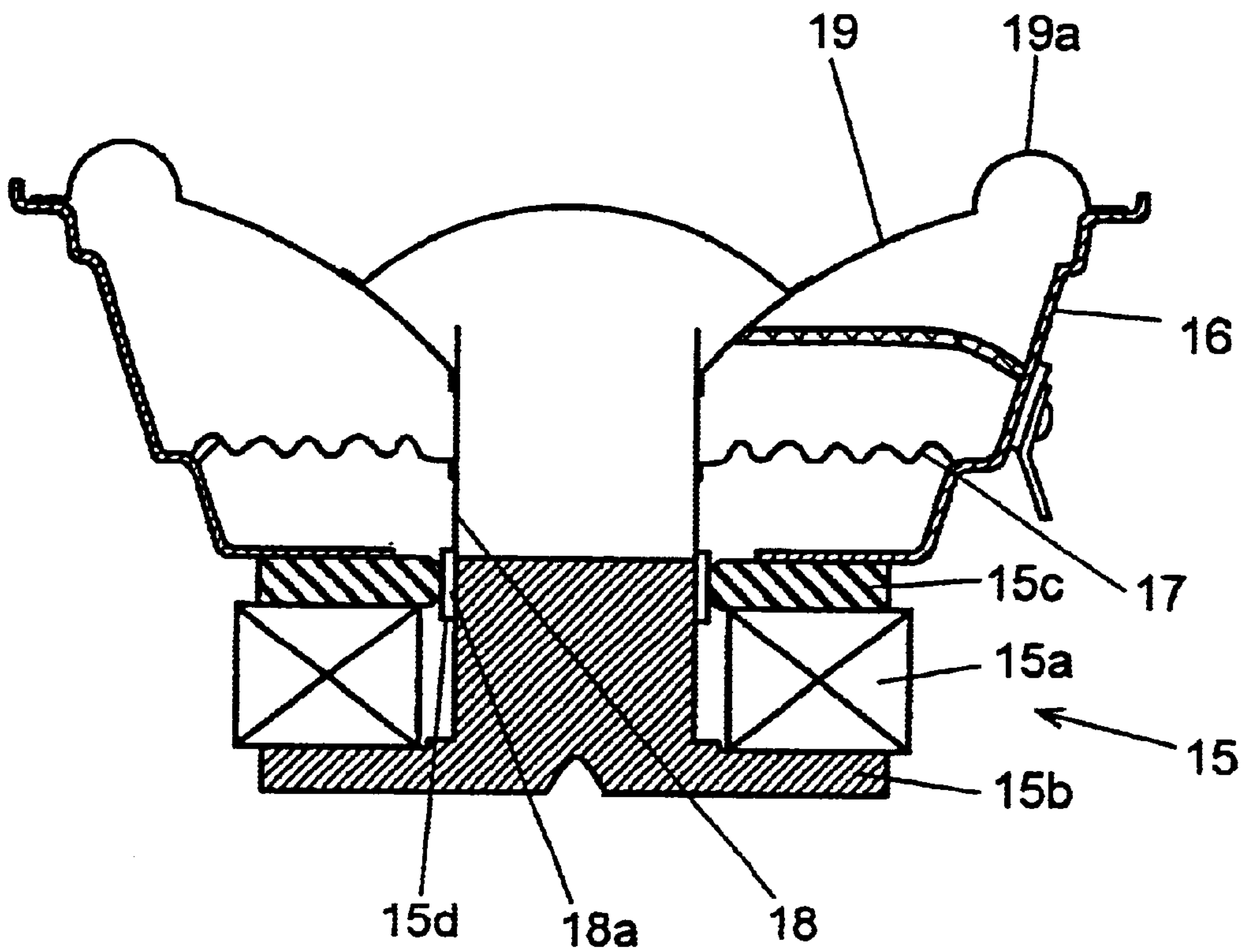
FIG. 7 PRIOR ART
