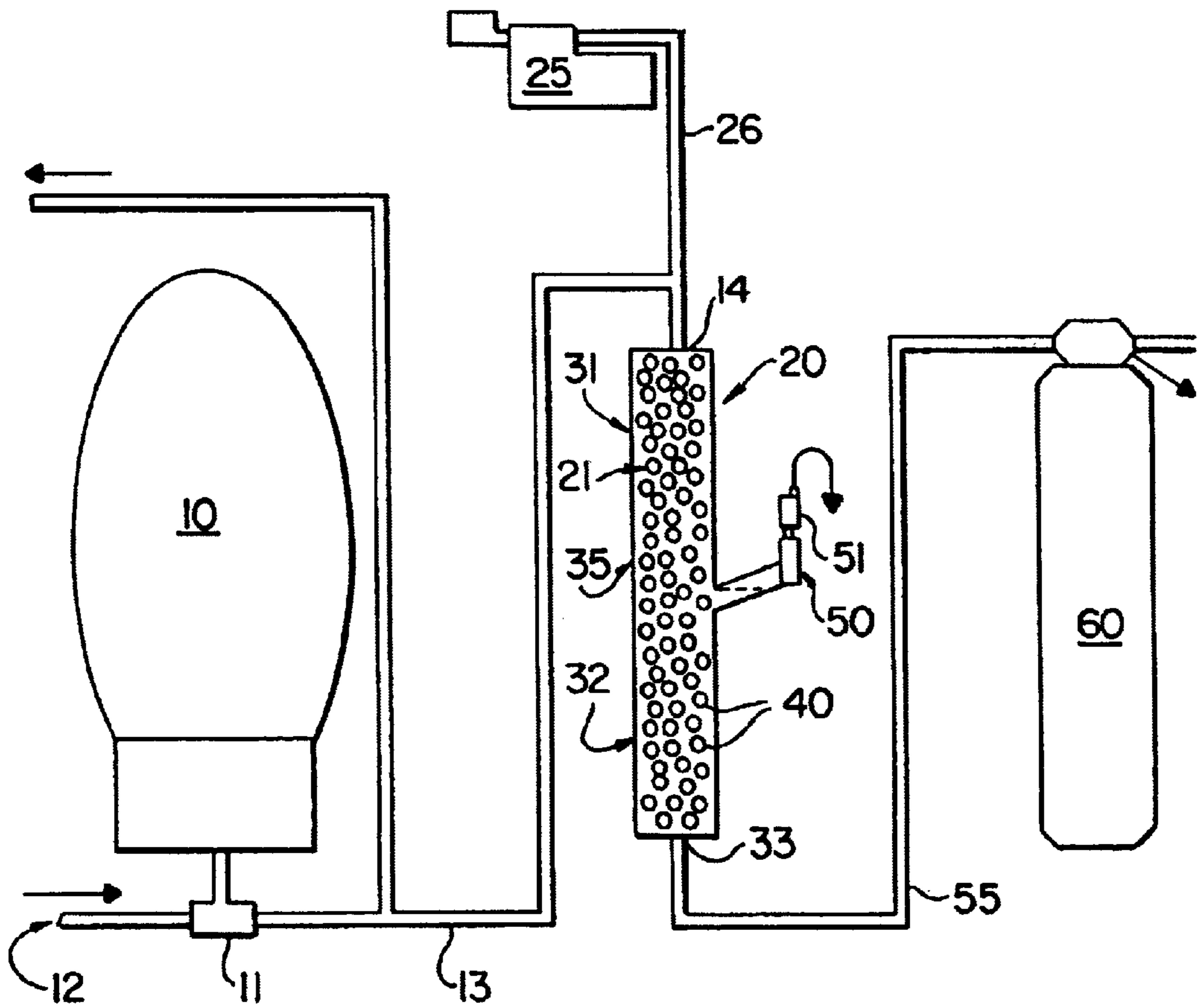
FIG. 1 (PRIOR ART)
