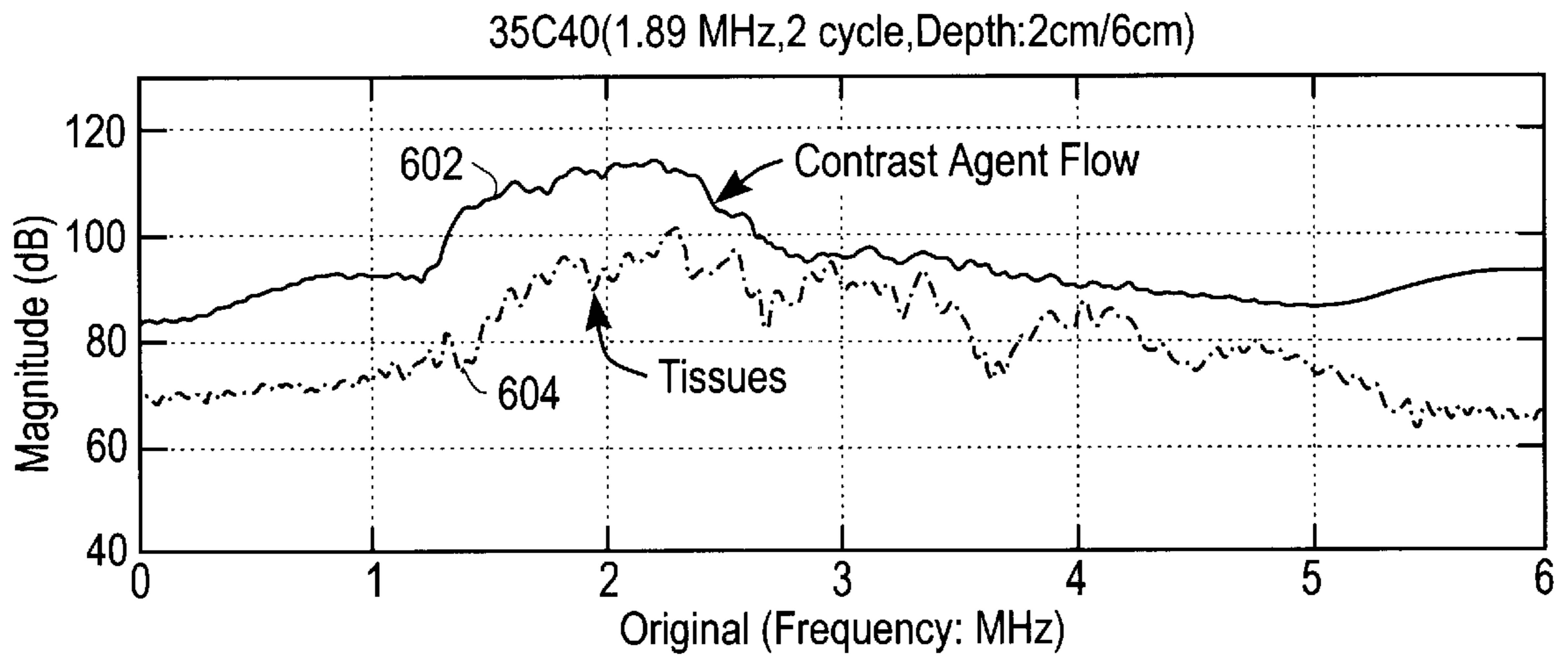
FIG. 6 The Spectra of Echoes from Single Transmit.
