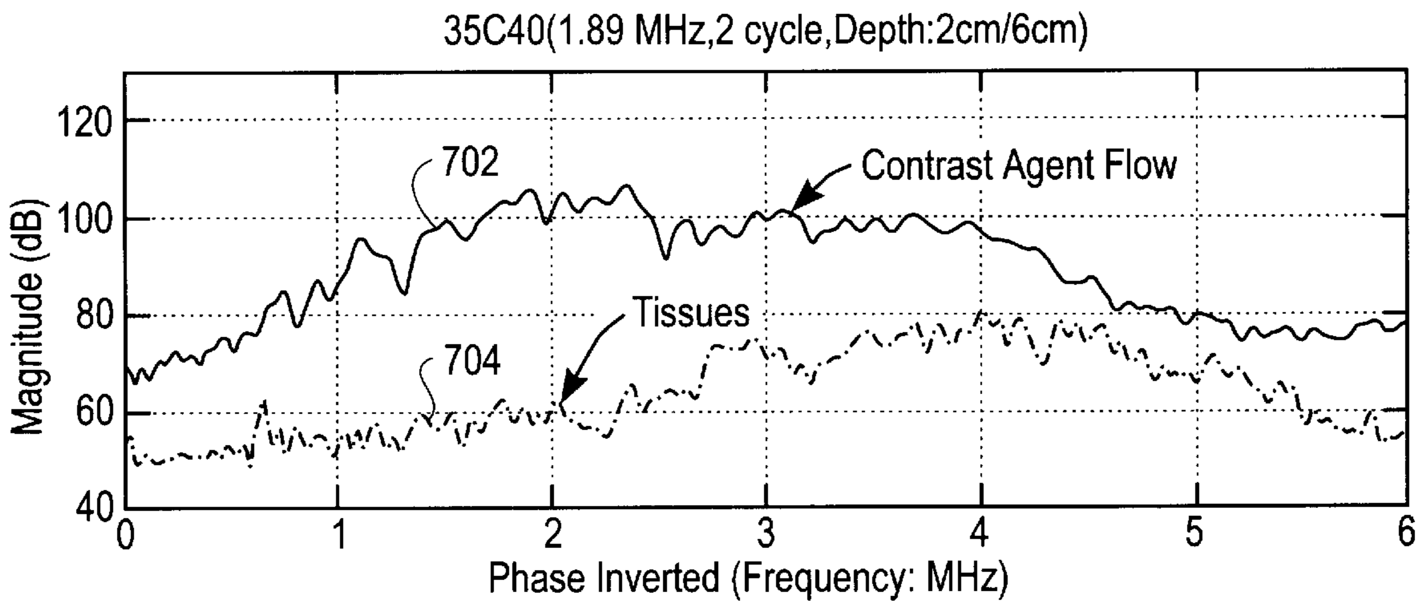
FIG. 7 The Spectrum of Echoes with PI Summation
