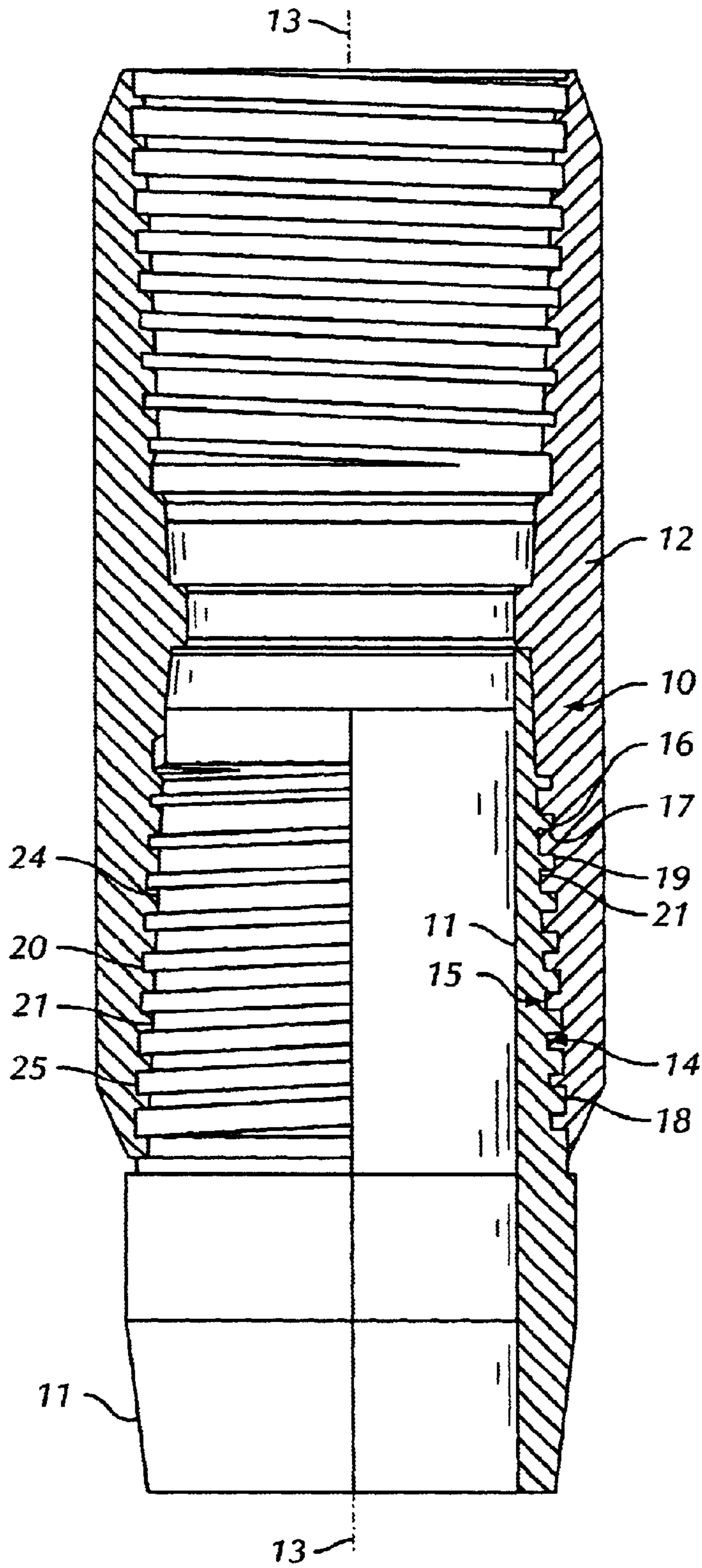
FIG. 1 (Prior Art)
