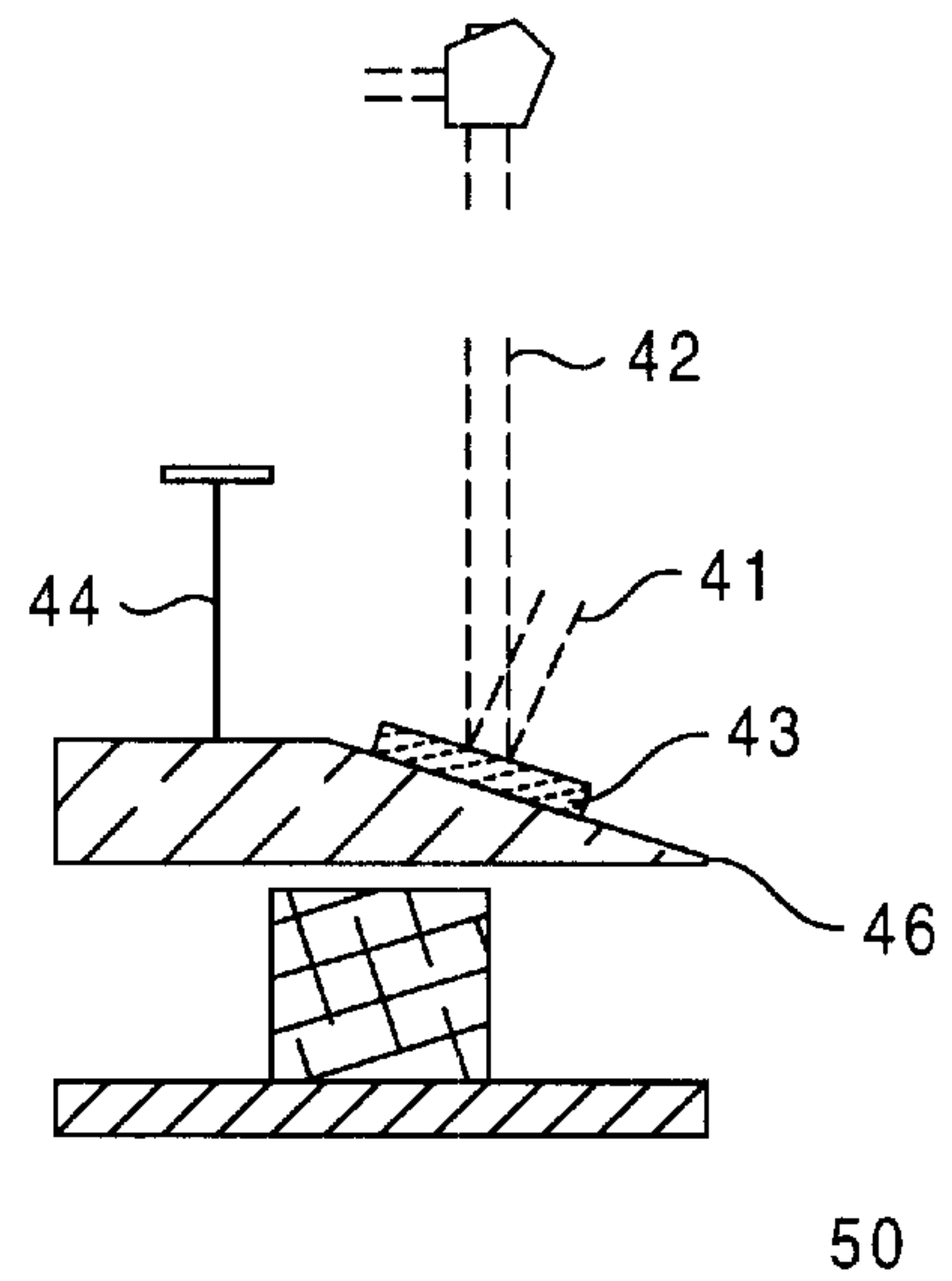
FIG. 5 (Prior Art)
