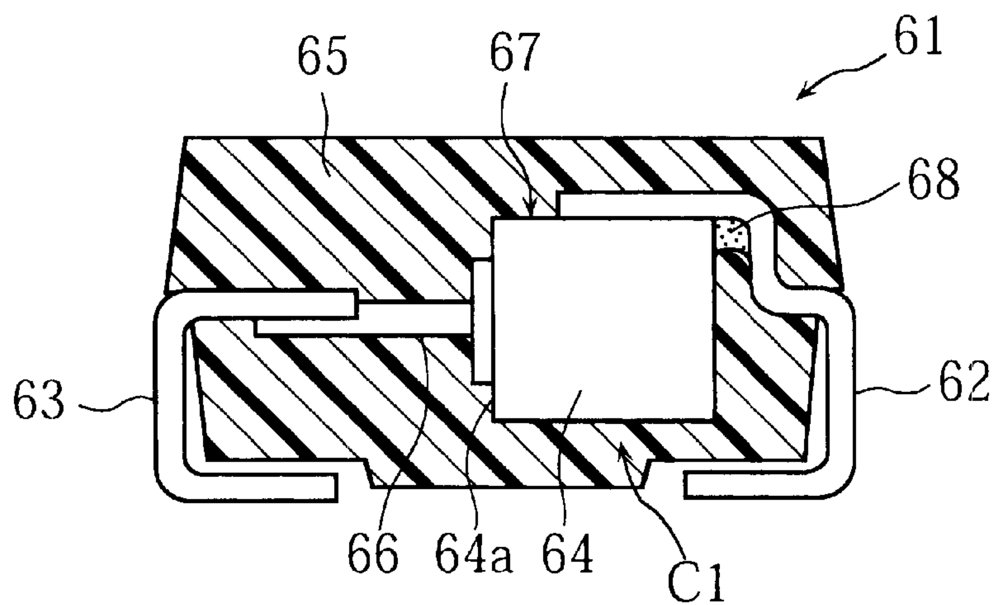
FIG.35 PRIOR ART
