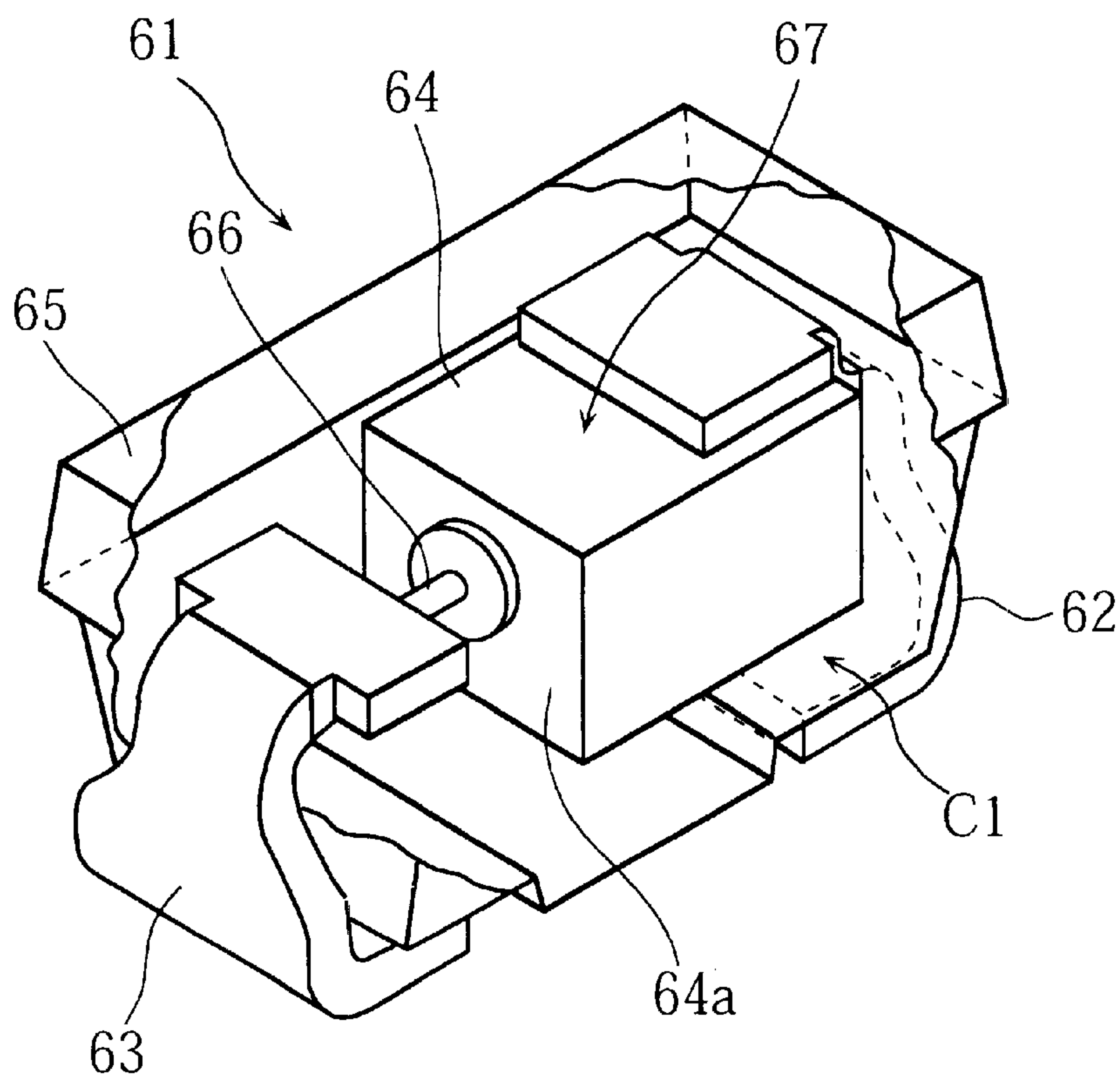
FIG.34 PRIOR ART
