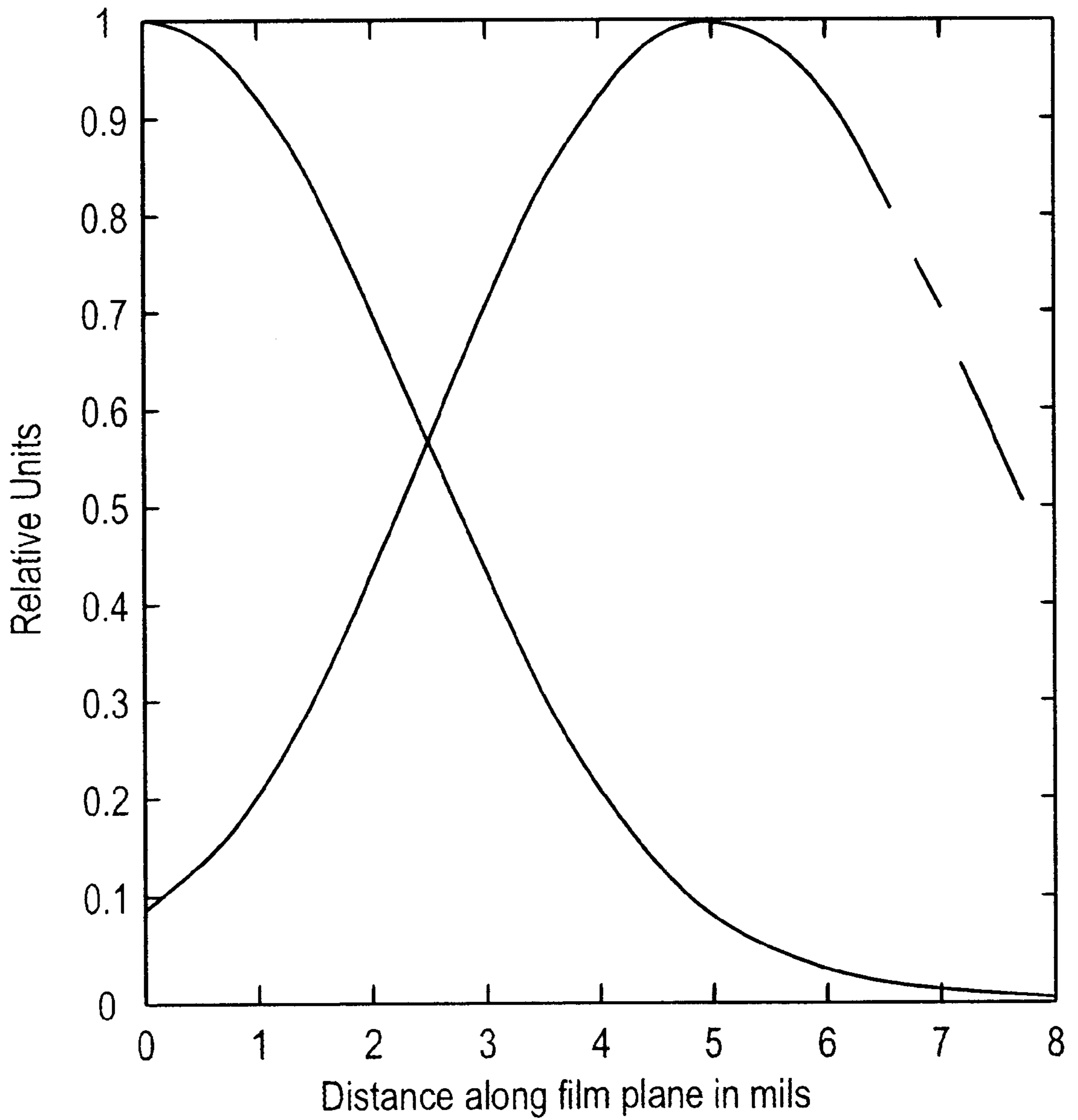
Normalized Intensity Profile on Film 2 with 2mil Thick Cover Sheet: Standard 1.6mil Thick Mask
