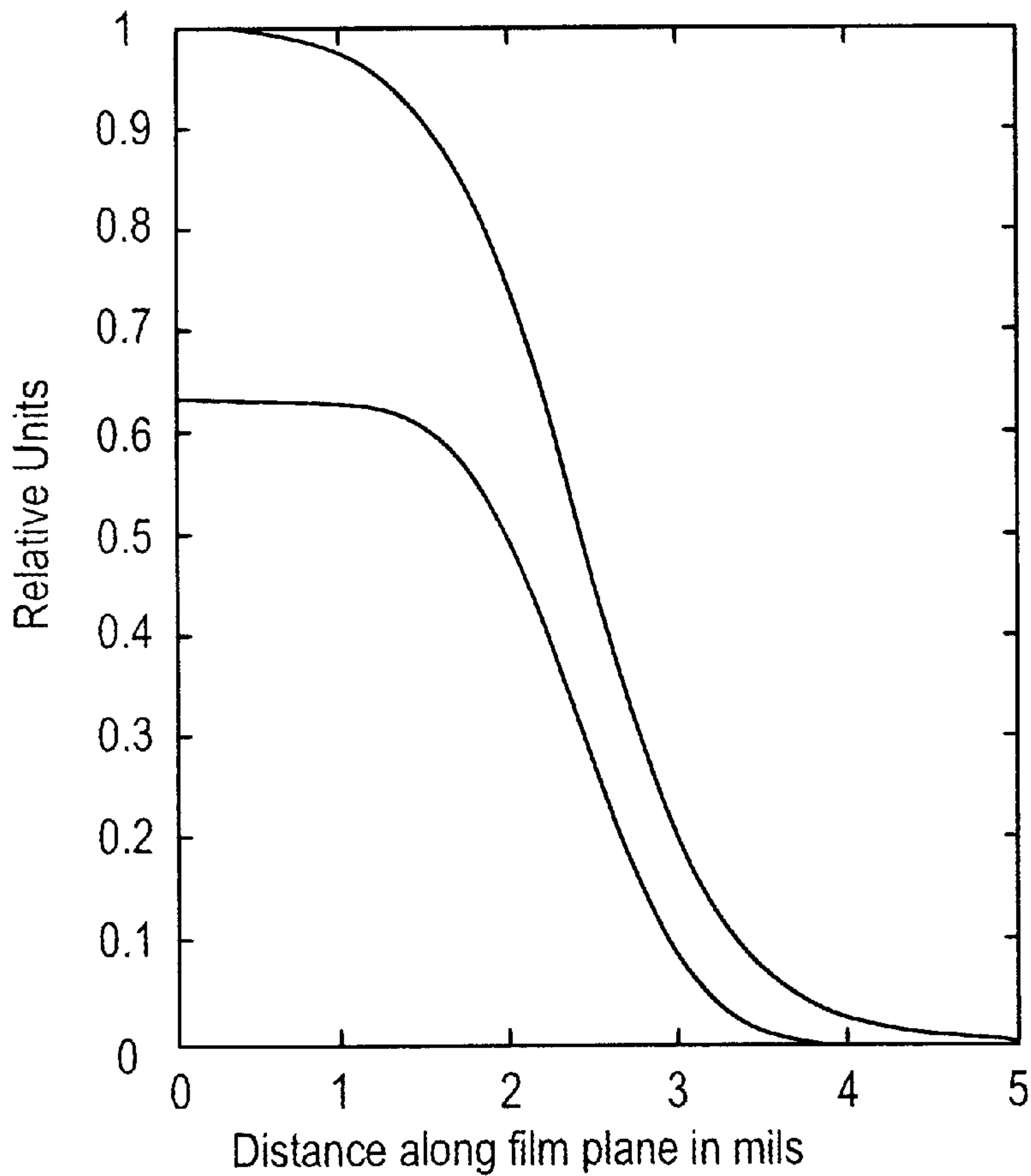
Relative Intensity Profile on Film 1 with and without Air Gap Both the OLED and Film 1 Cover Sheet = 0.7mils (combined 1.4 mils)
