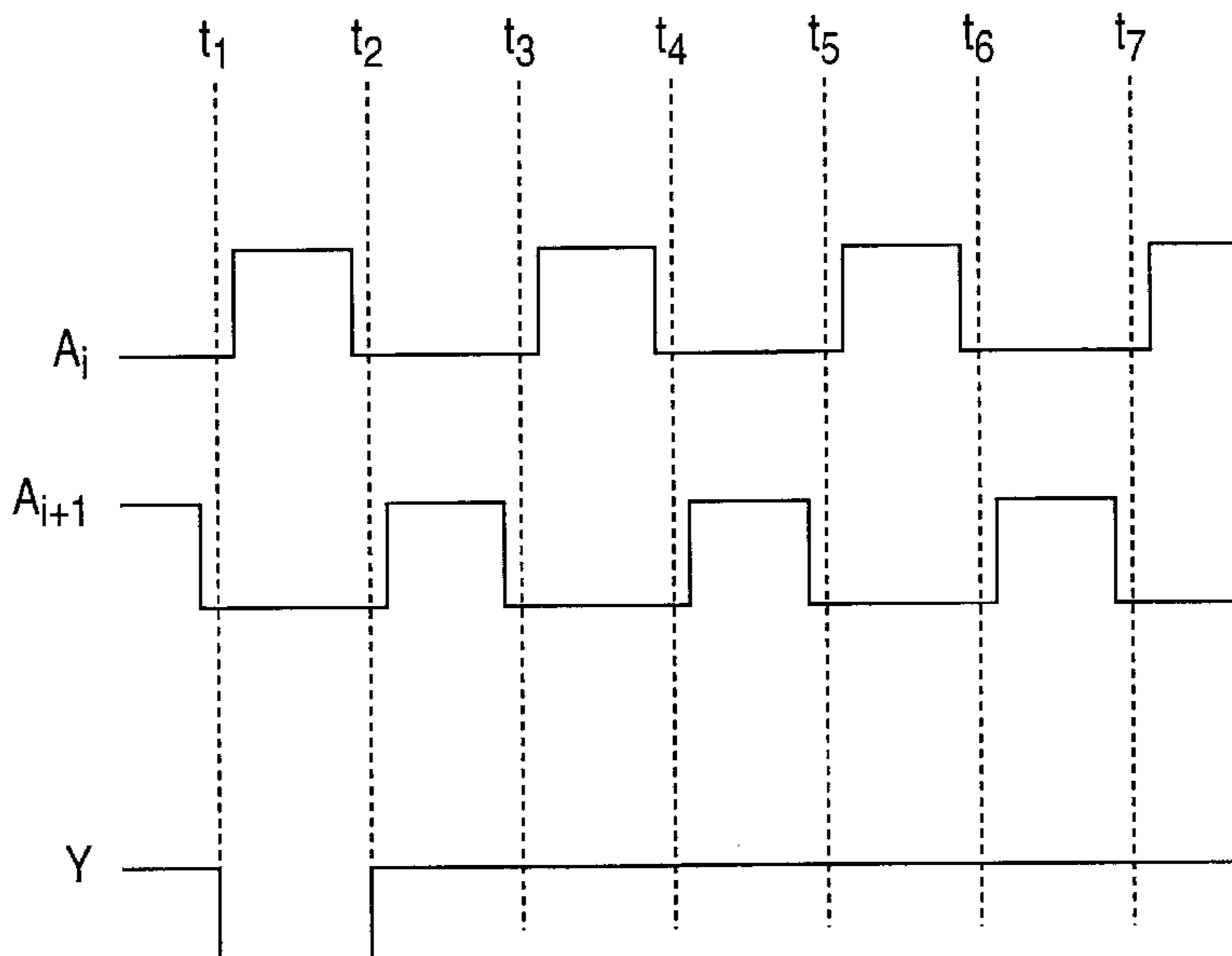
WAVEFORM OF DRIVE PULSE EXAMPLE 1
