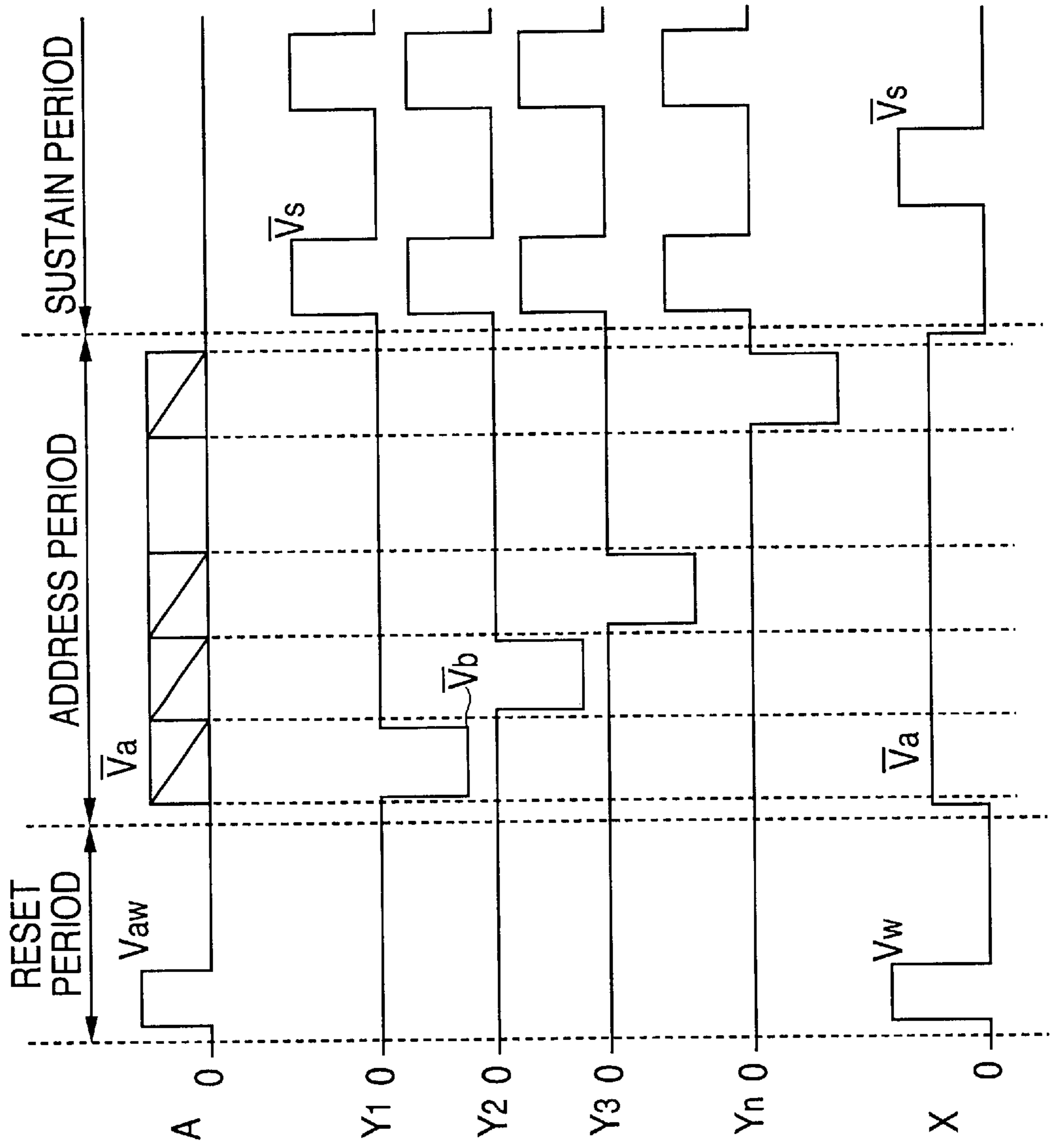
FIG. 4 (PRIOR ART)
