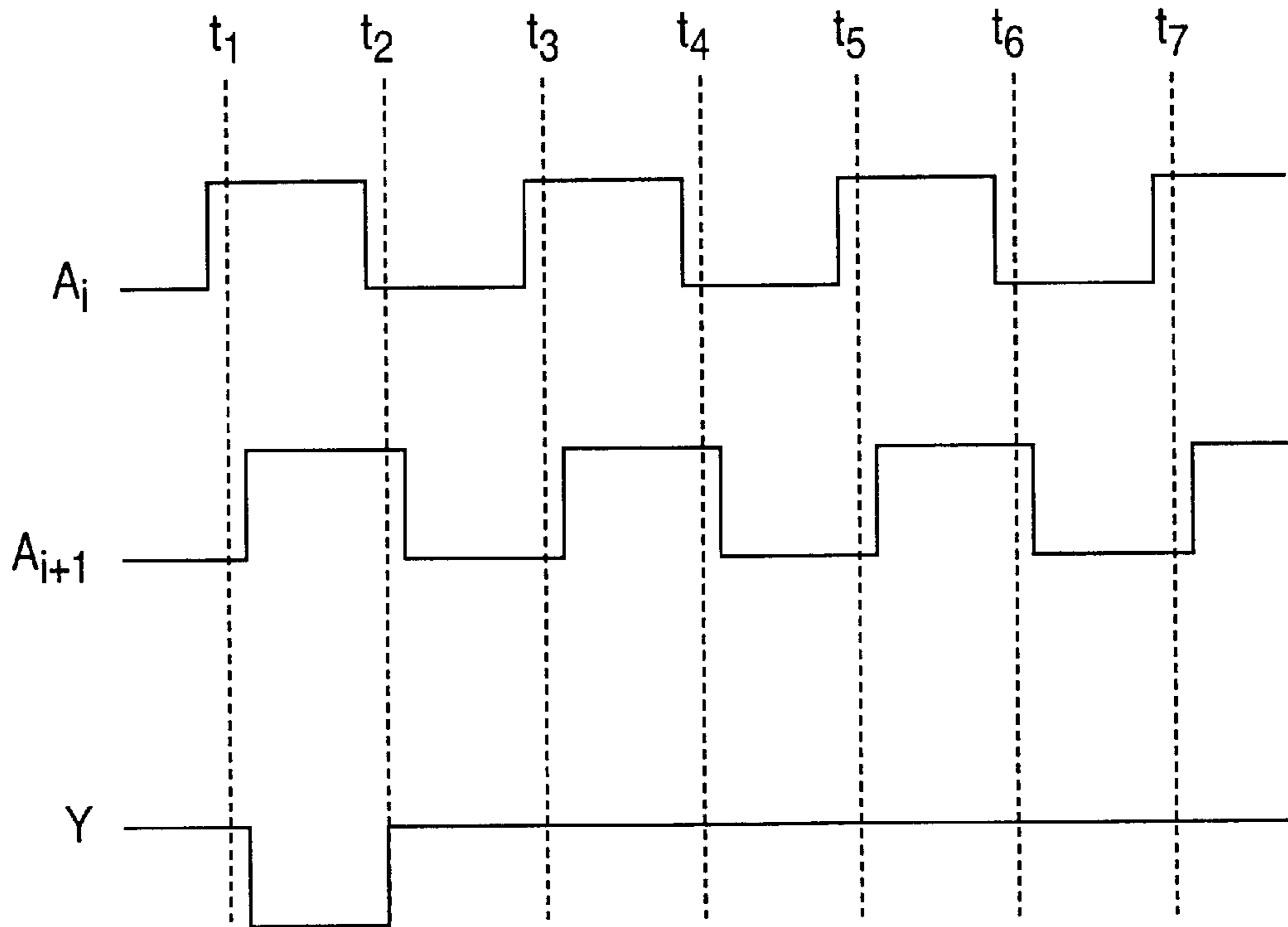
WAVEFORM OF DRIVE PULSE EXAMPLE 4
