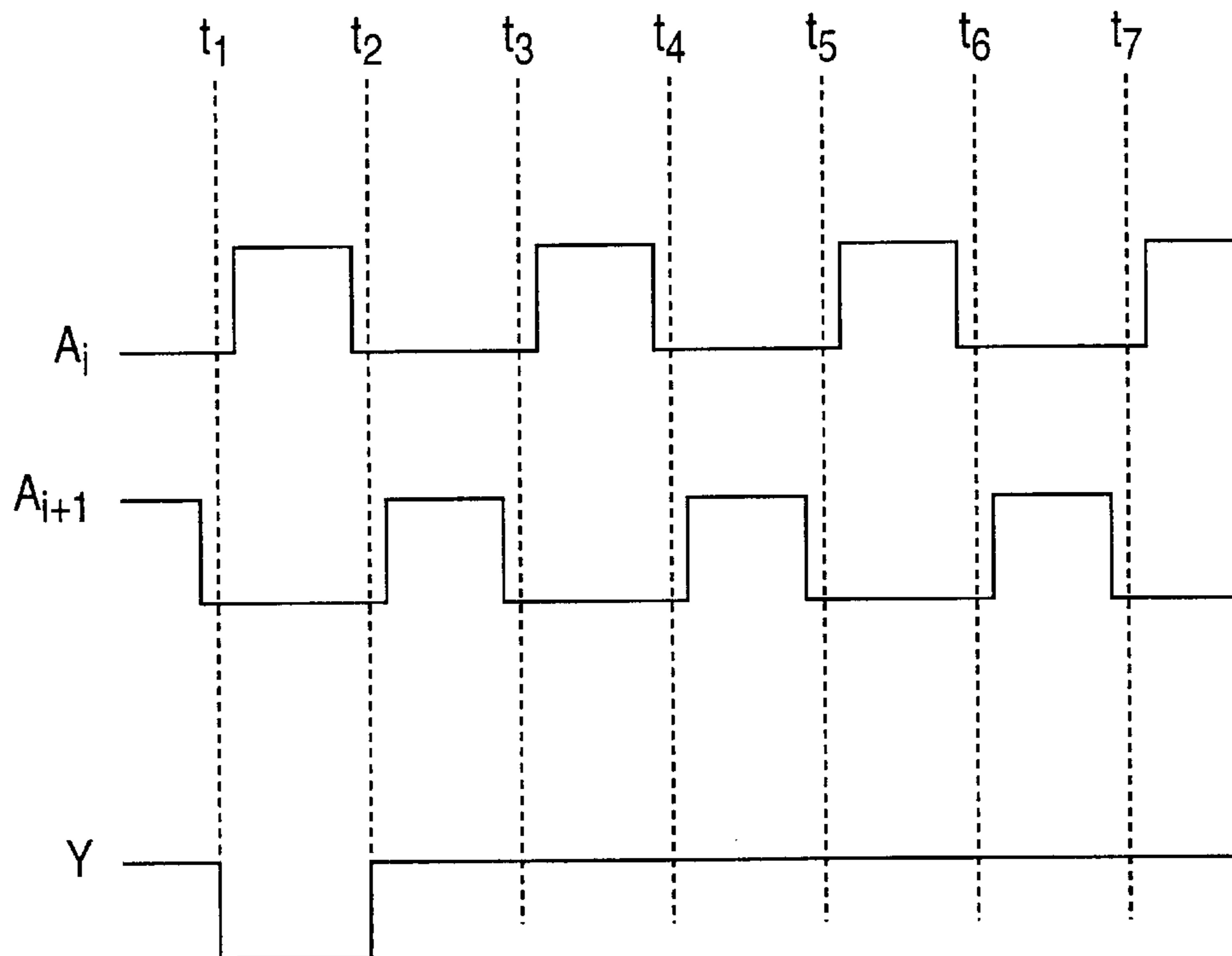
WAVEFORM OF DRIVE PULSE EXAMPLE 1
