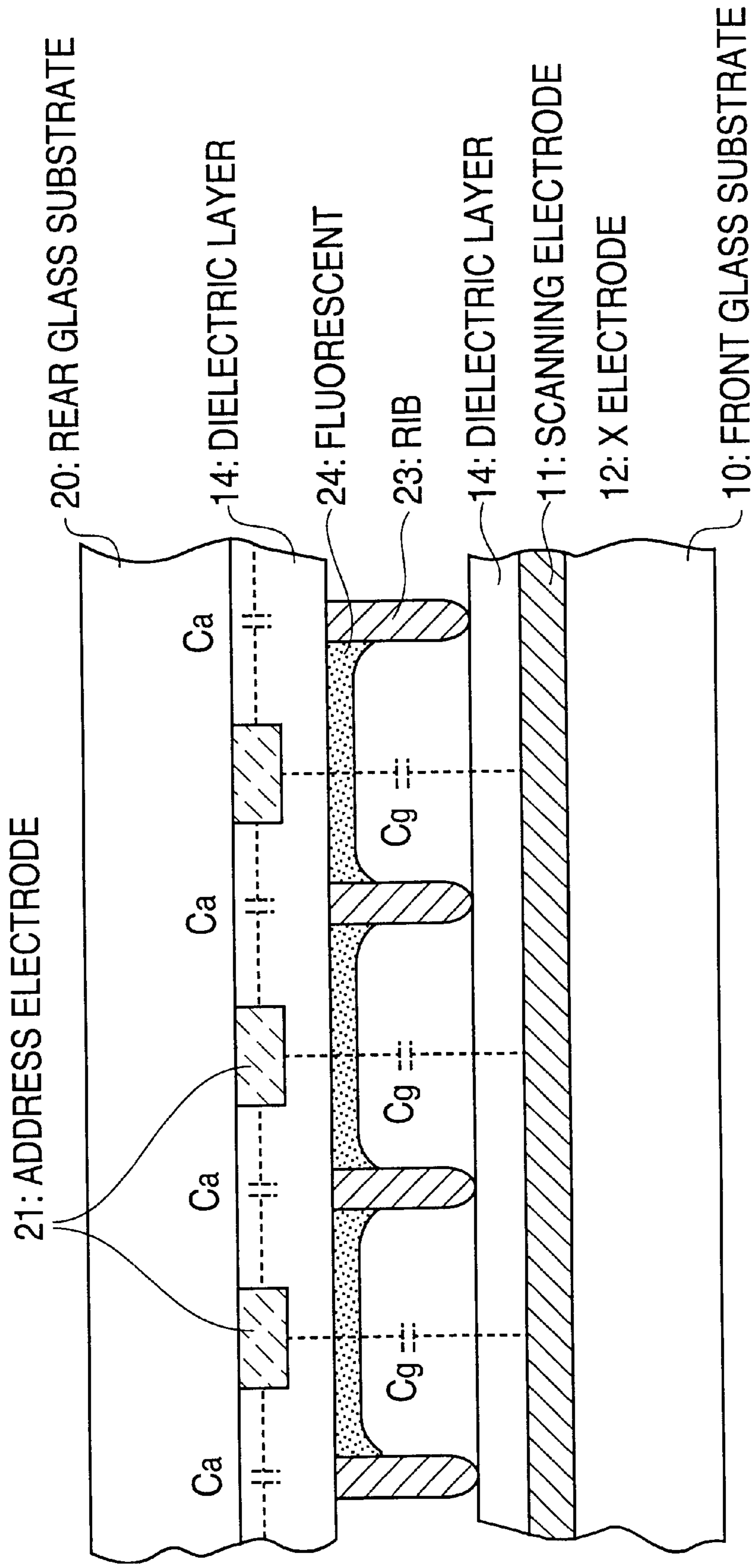
FIG. 2 (PRIOR ART)
