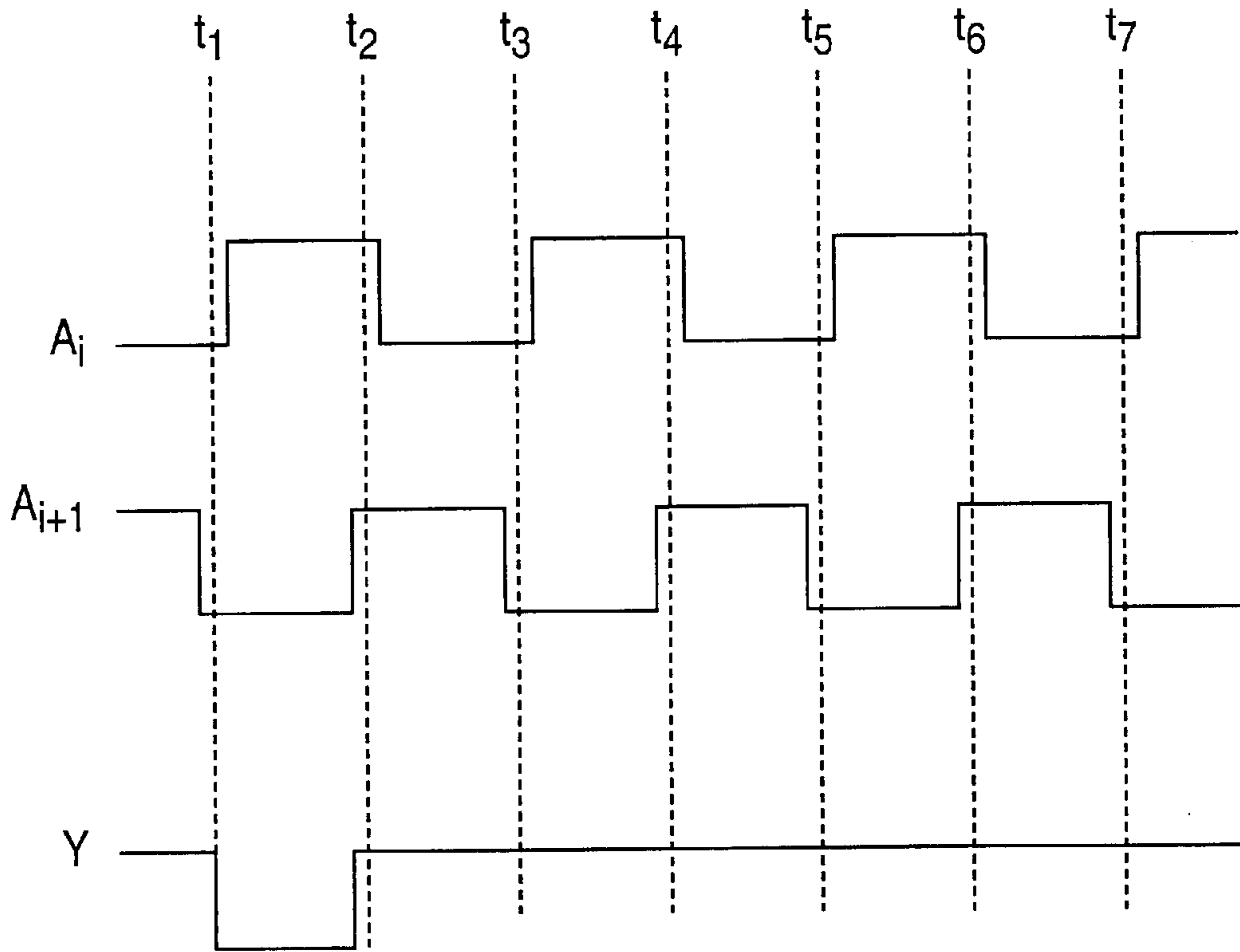
WAVEFORM OF DRIVE PULSE EXAMPLE 3
