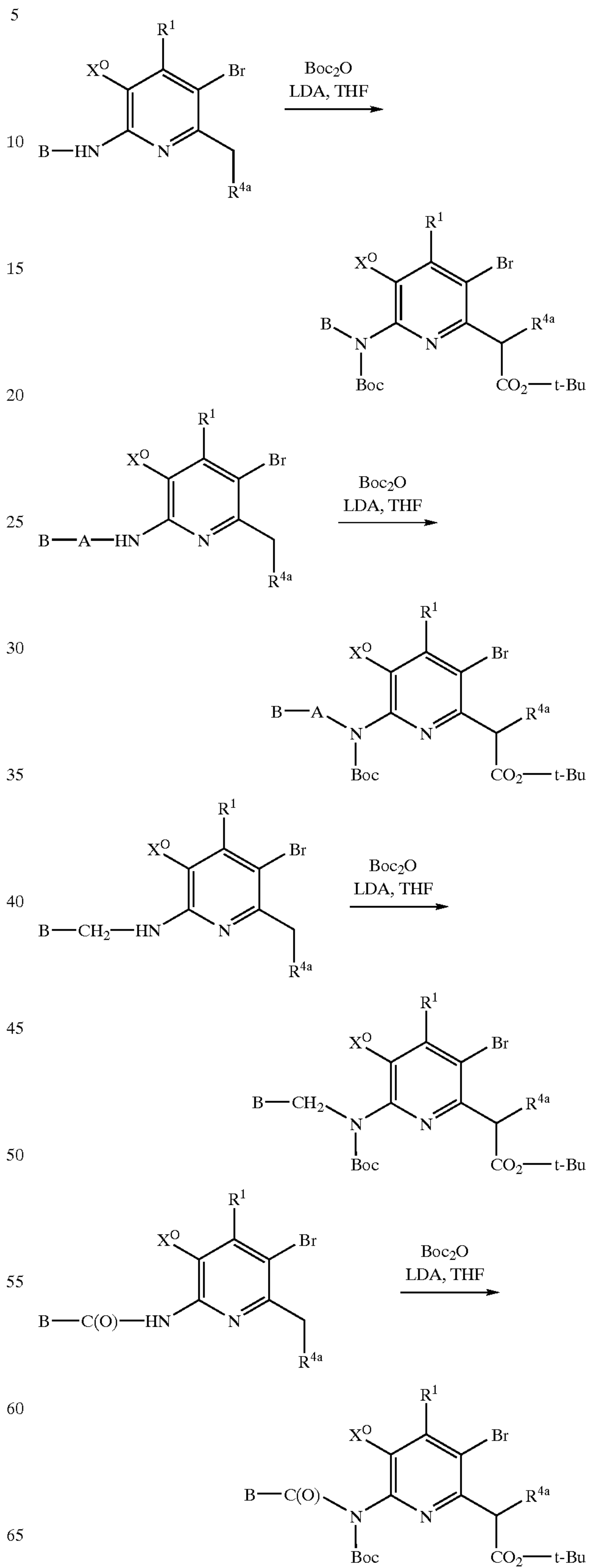
Scheme 3 General Synthesis of Pyridines
