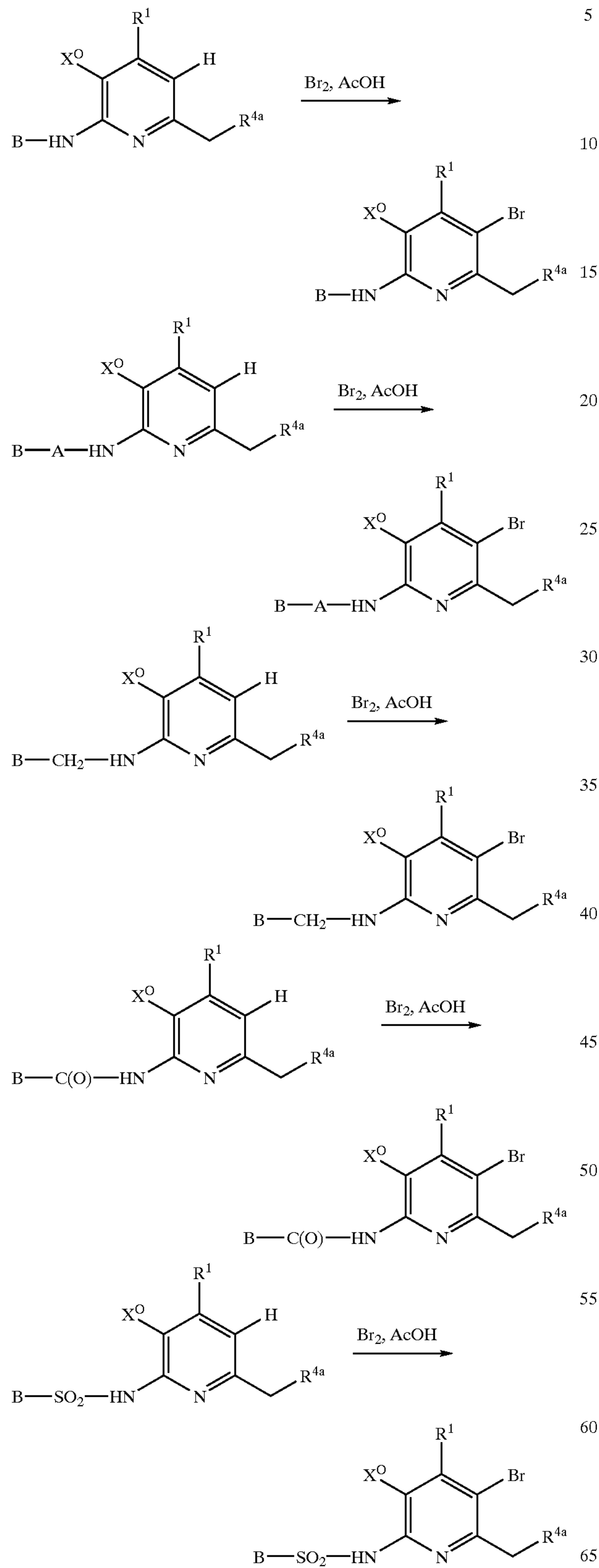
Scheme 2 General Synthesis of Pyridines
