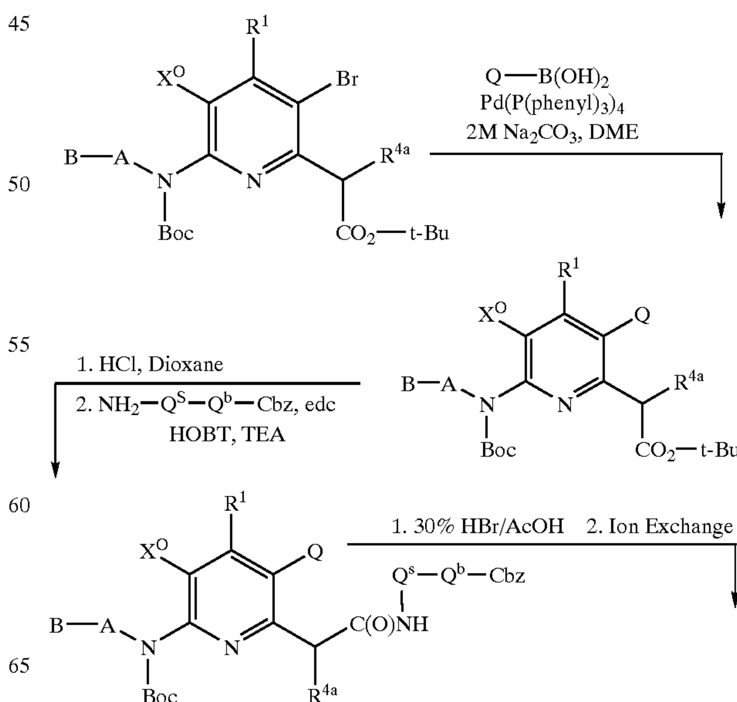
Scheme 5 General Synthesis of Pyridines
