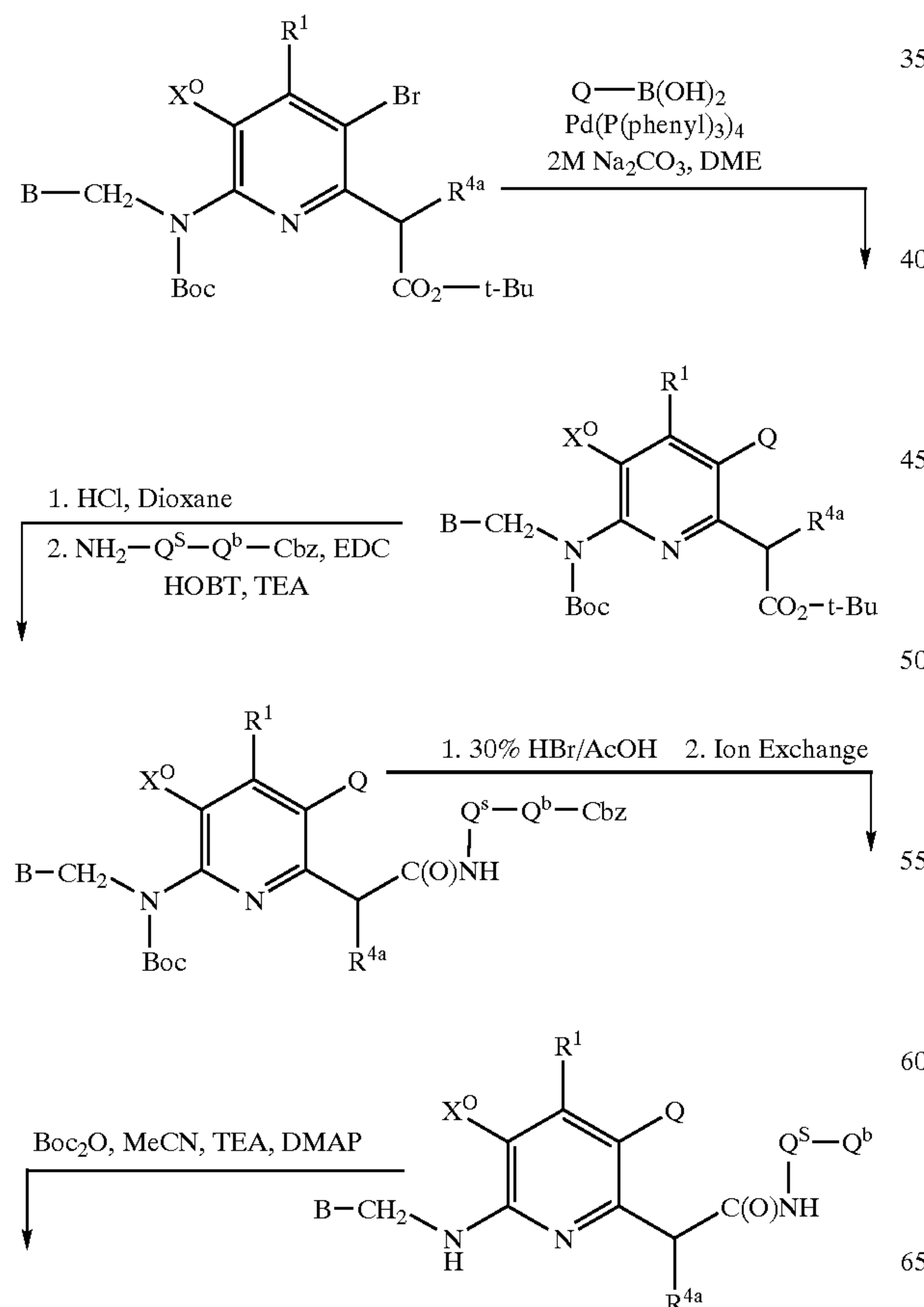
Scheme 6 General Synthesis of Pyridines
