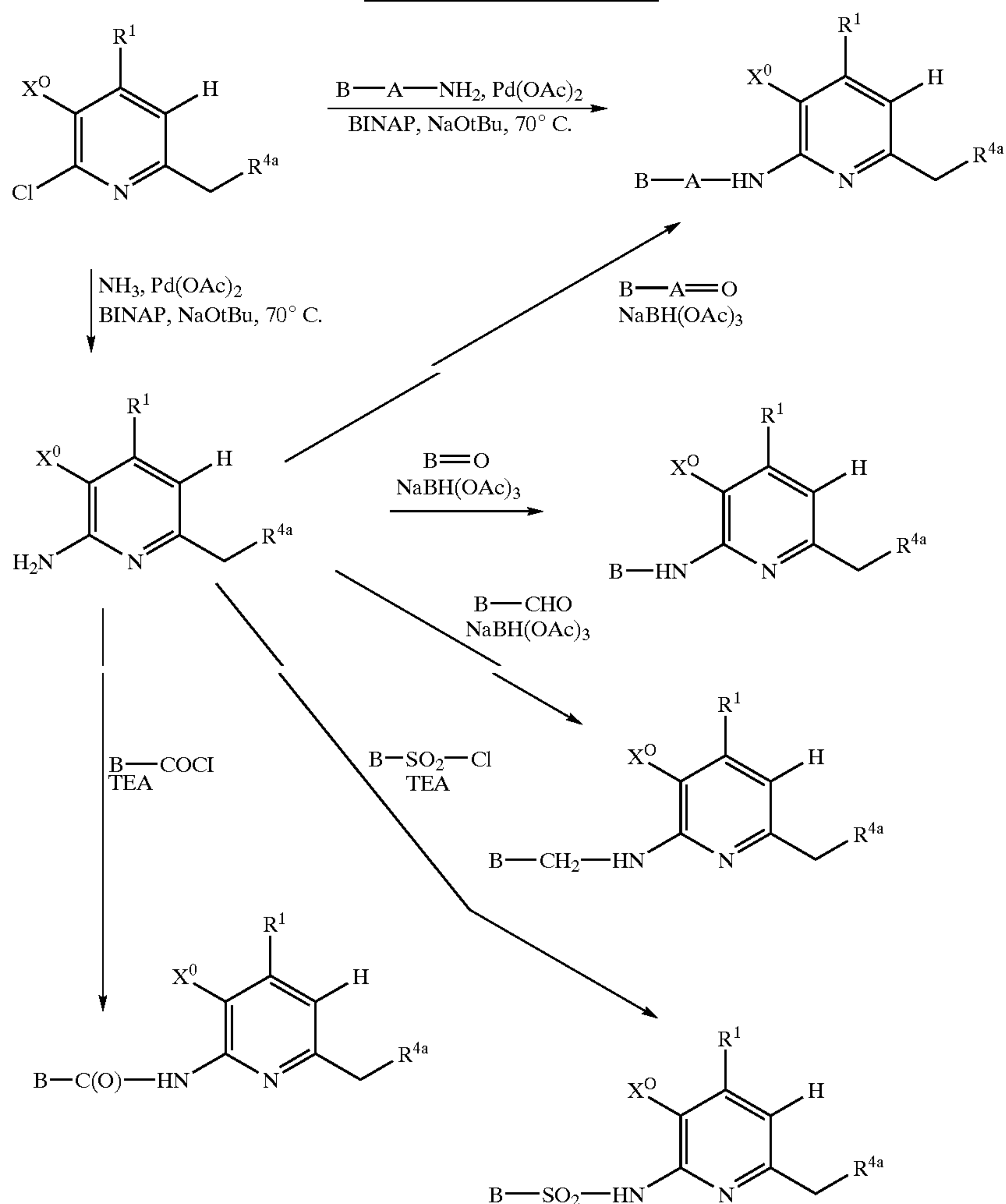
Scheme 1 General Synthesis of Pyridines
