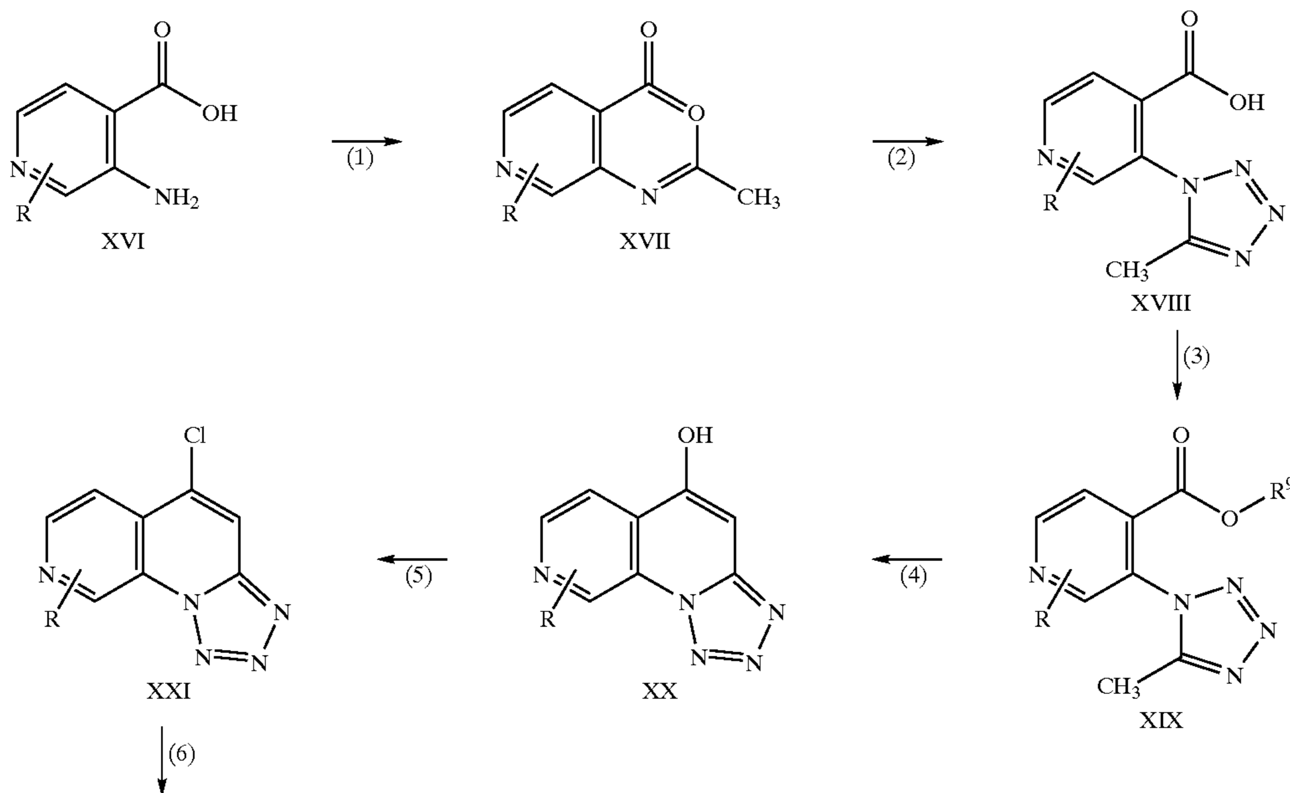
Reaction Scheme II
