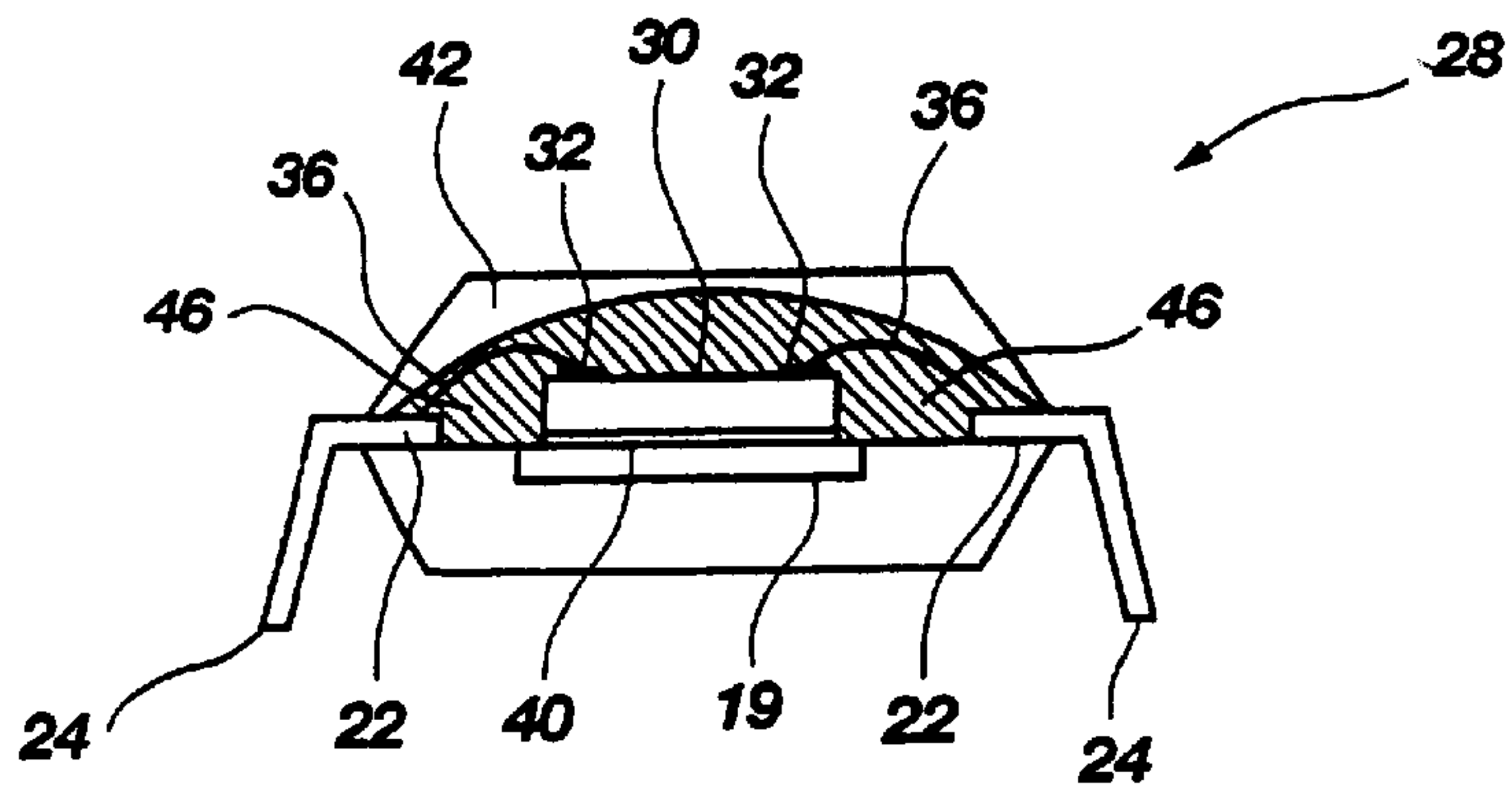
Fig. 2 (PRIOR ART)
