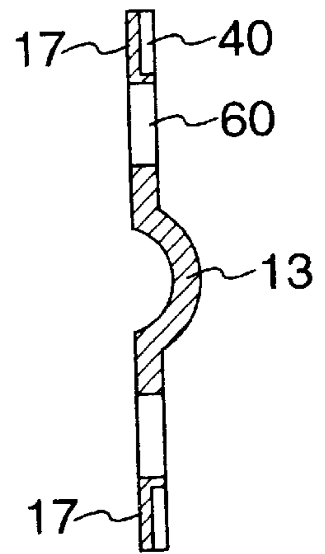
CROSS SECTION TAKEN ALONG LINE E-E (ENLARGED)
