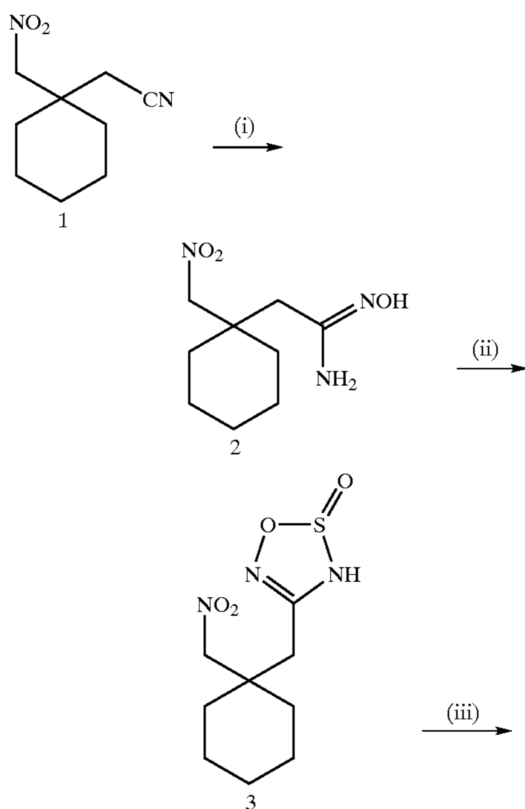
Scheme 8
