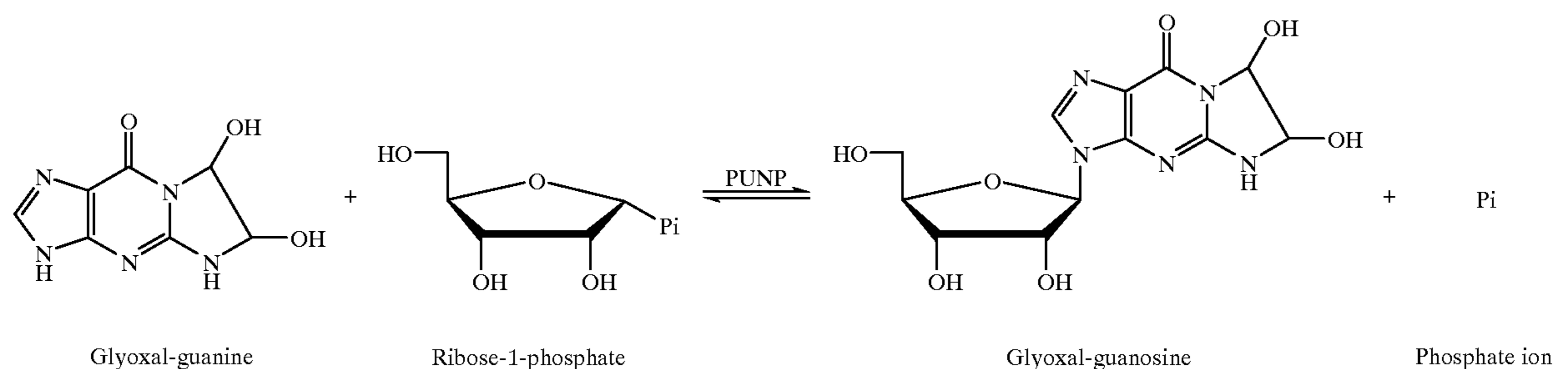
Reaction formula 4
