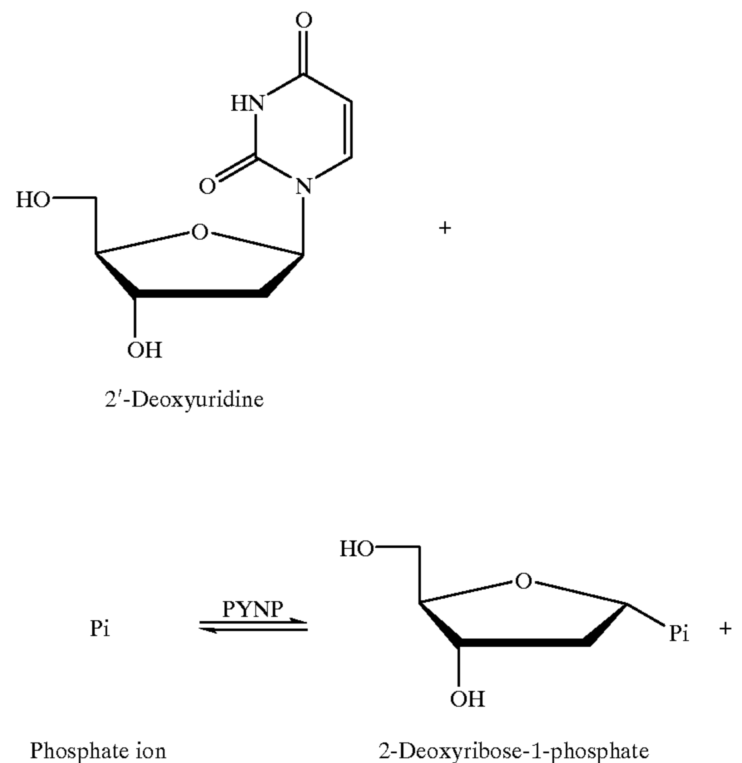
Reaction formula 1
