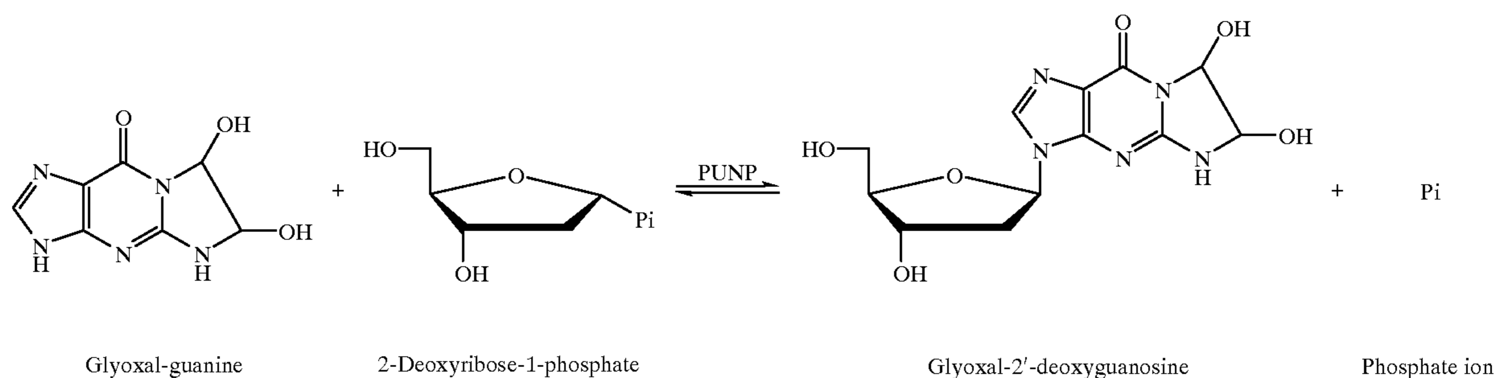
Reaction formula 2
