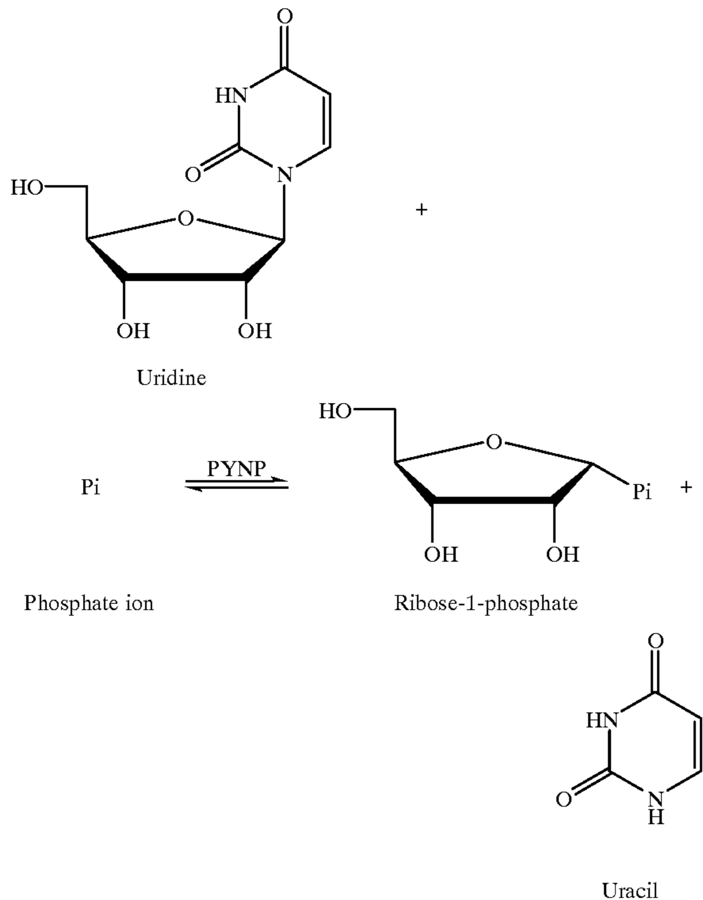
Reaction formula 3
