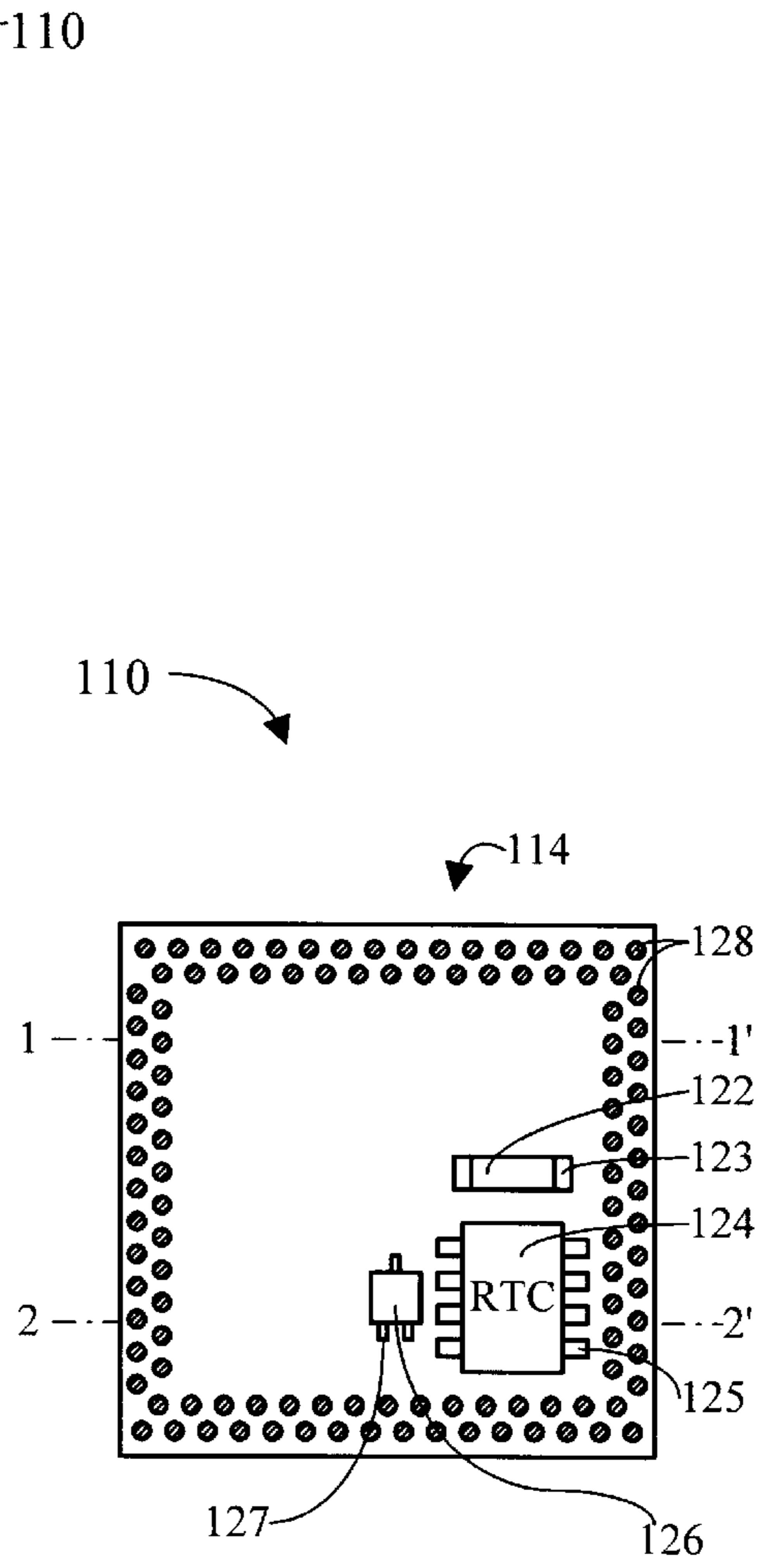
FIG. 1B Bottom Surface of Top Card
