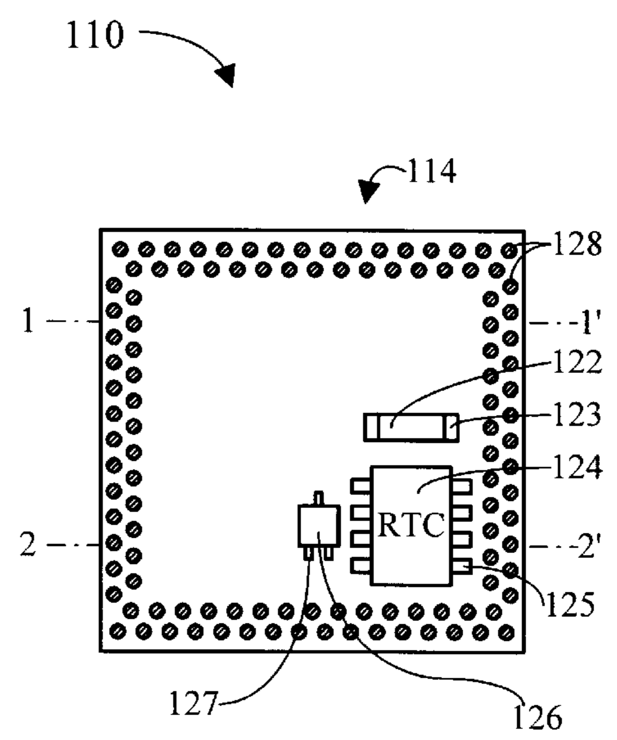
FIG. 1B Bottom Surface of Top Card
