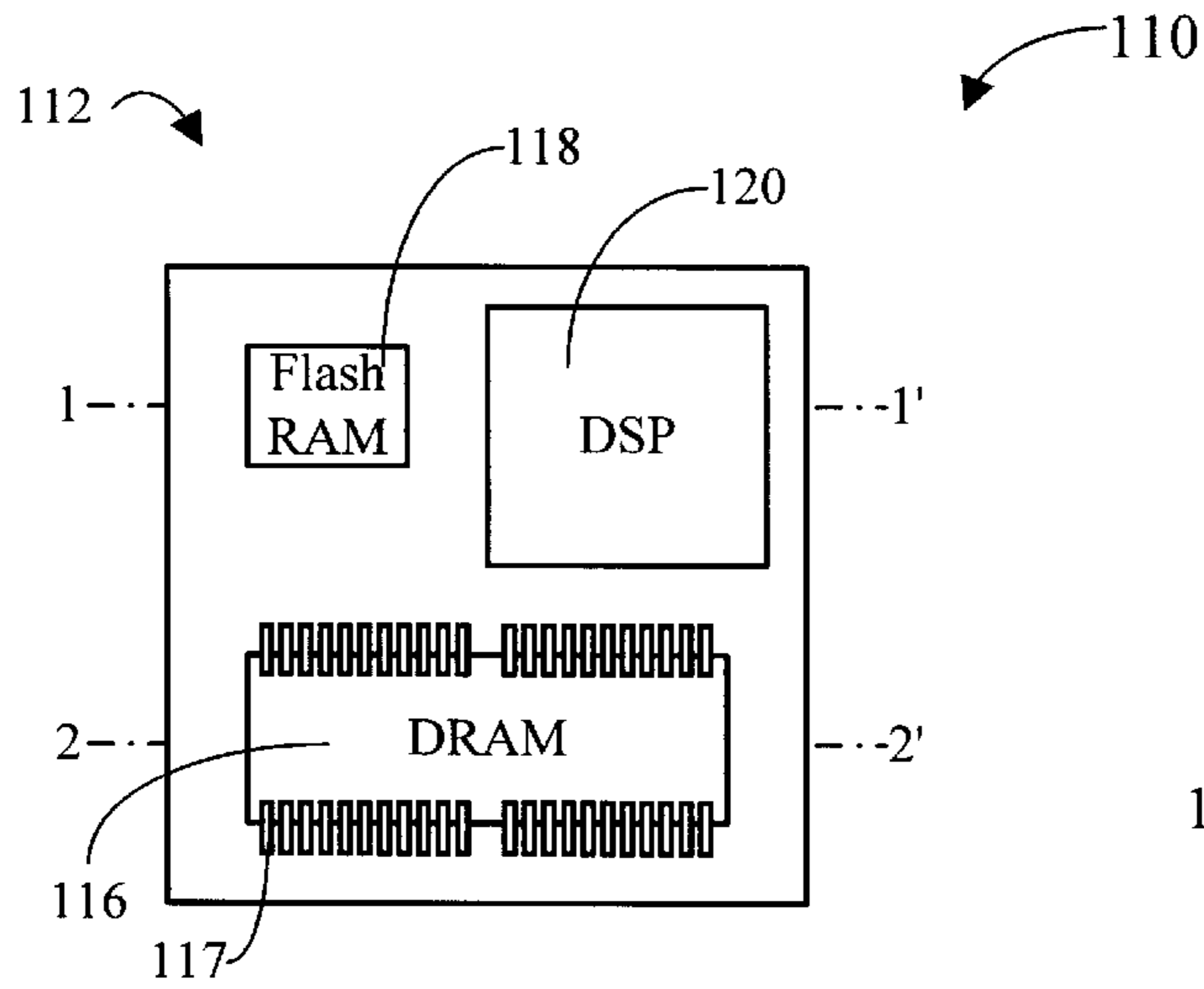
FIG. 1A Top Surface of Top Card
