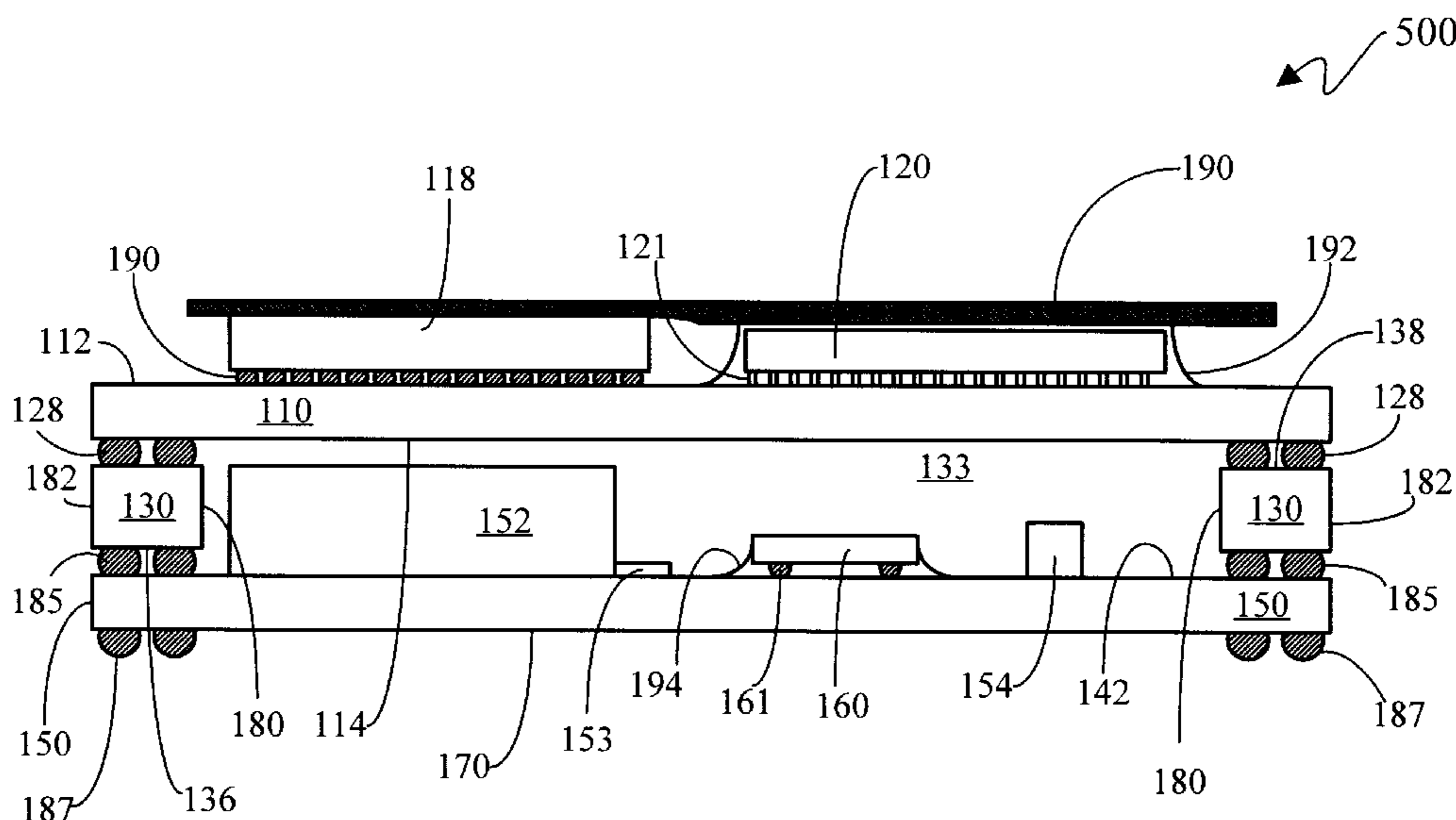
Cross Section 1-1'
