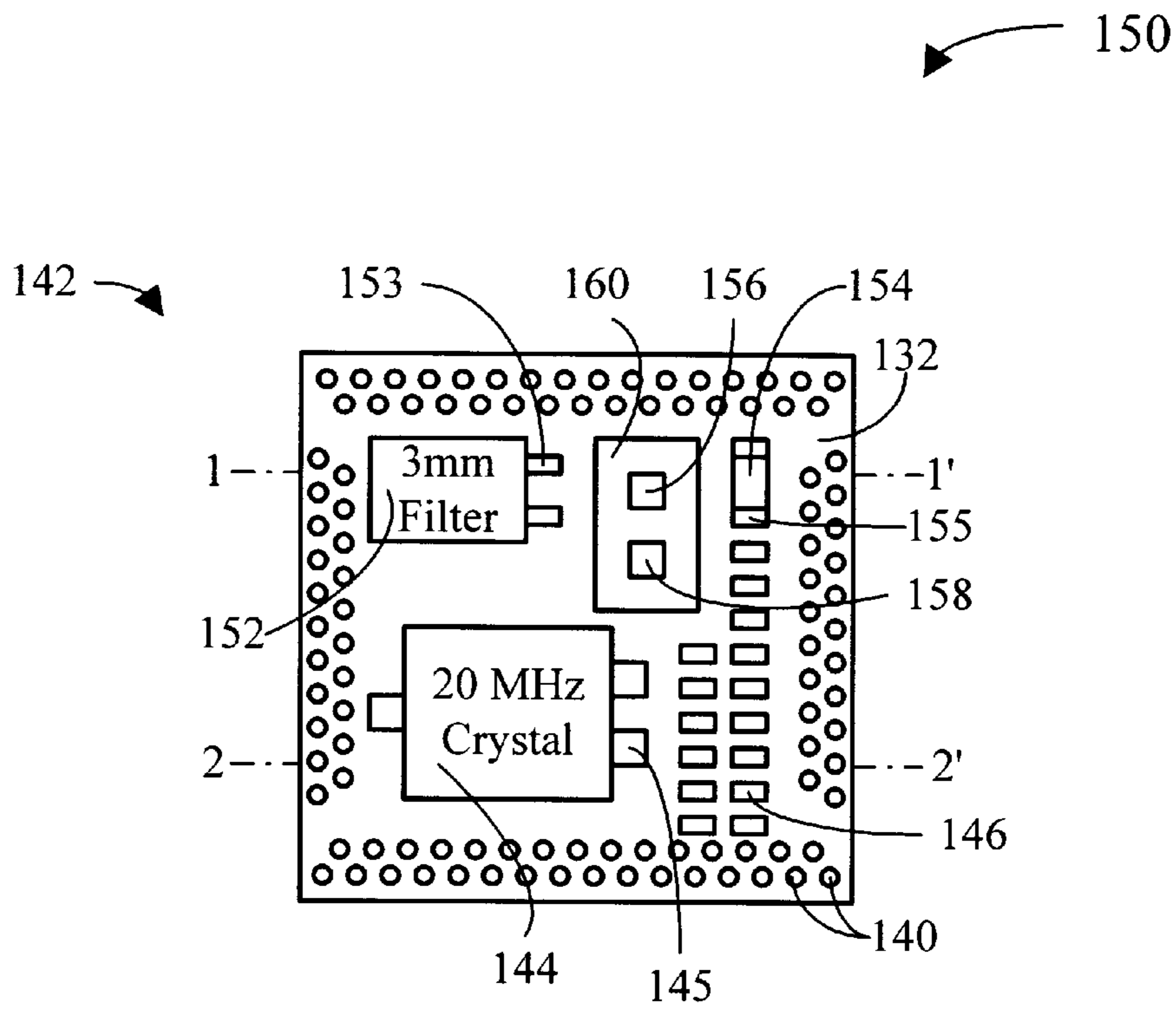
FIG. 3A Top Surface of Bottom Card
