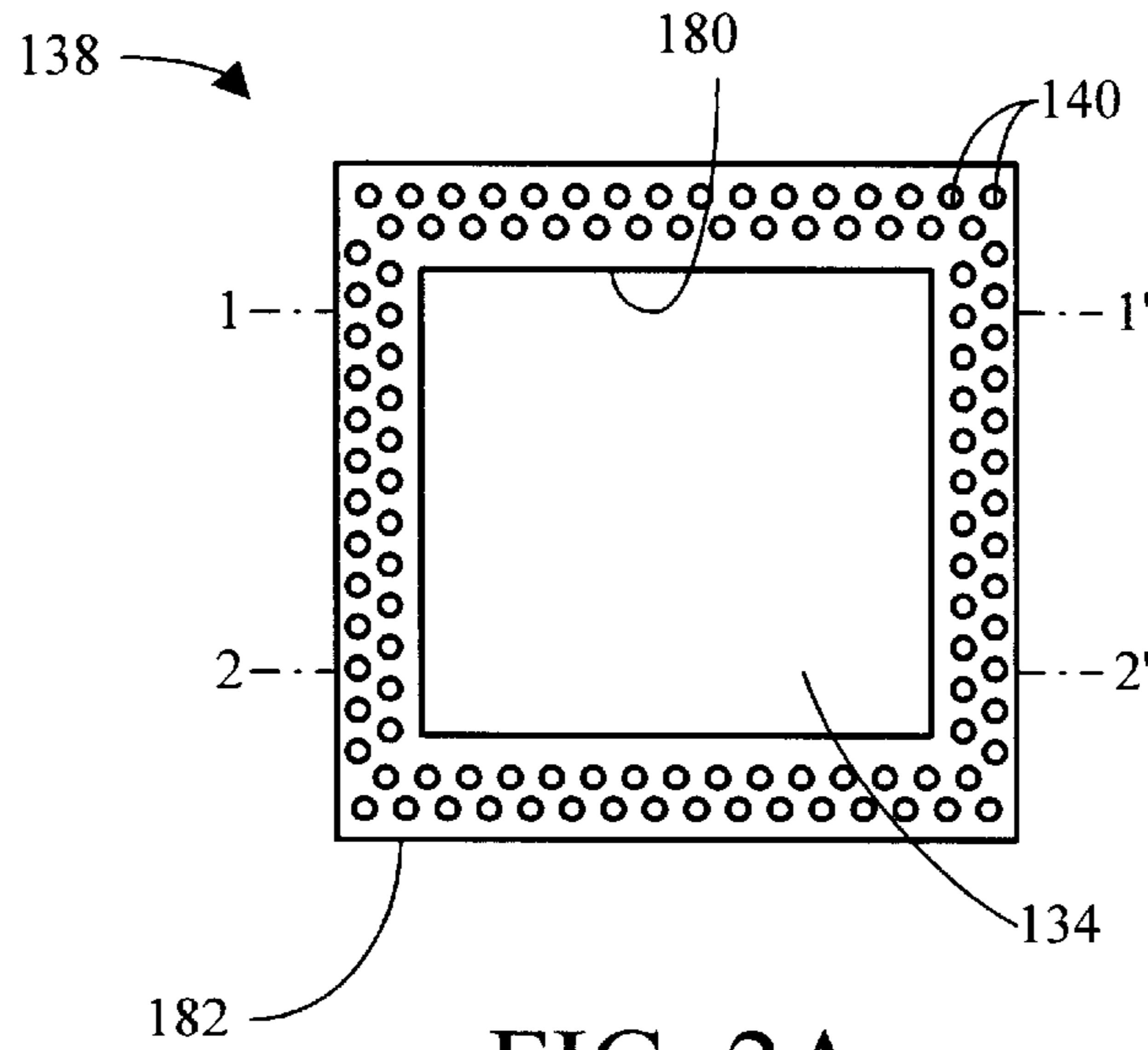
FIG. 2A Top Surface of Interposer
