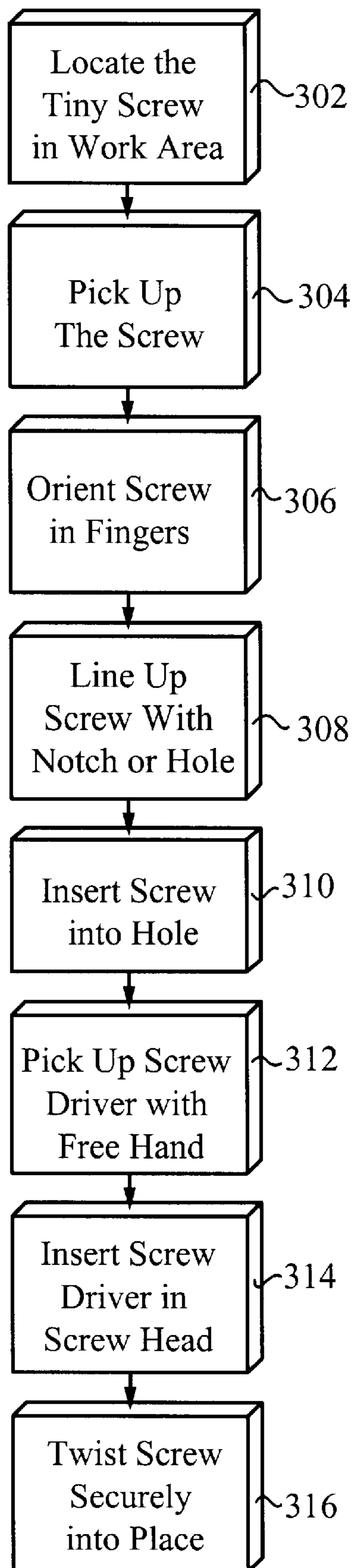
Fig. 3 PRIOR ART
