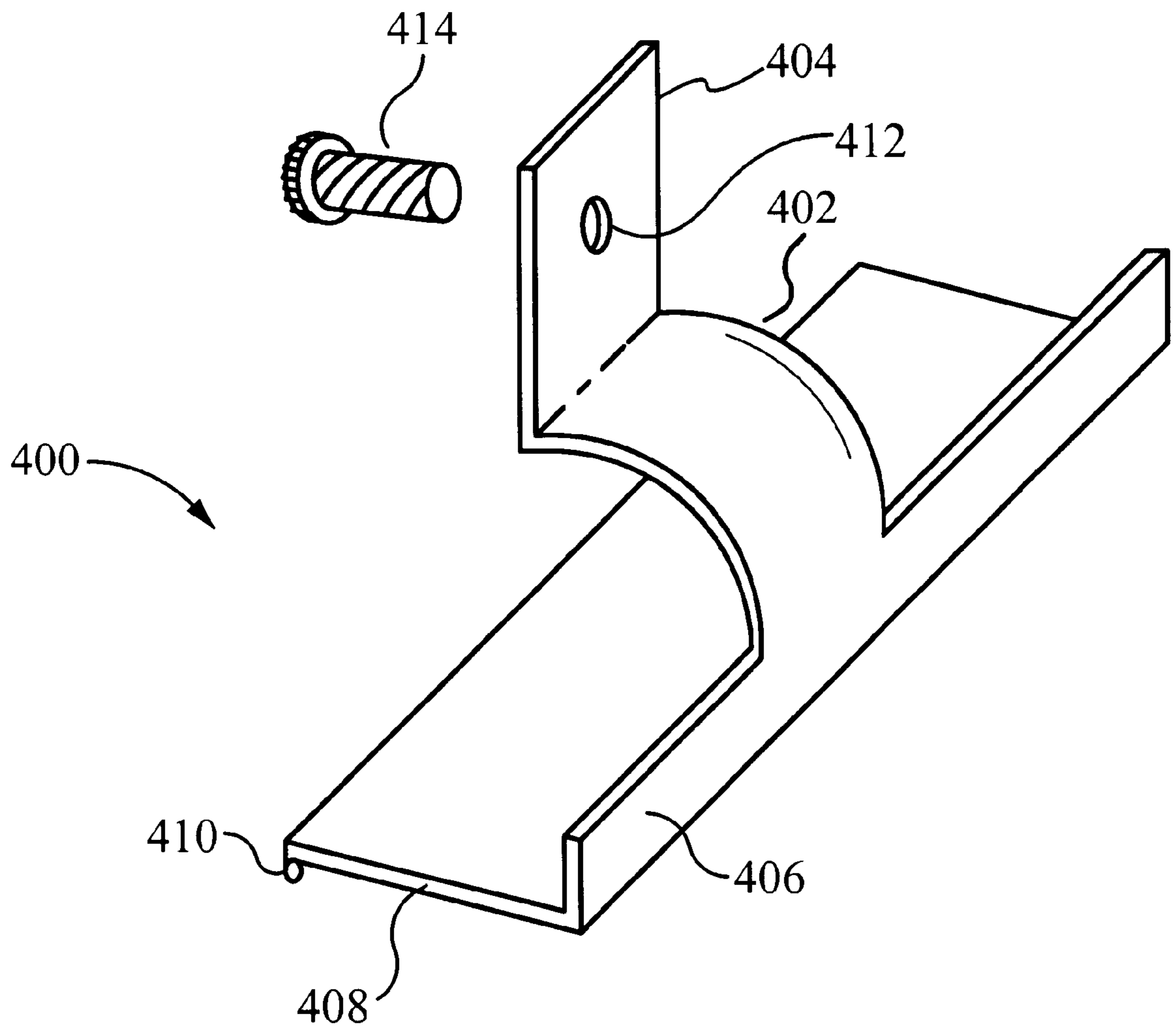
Fig. 4 PRIOR ART
