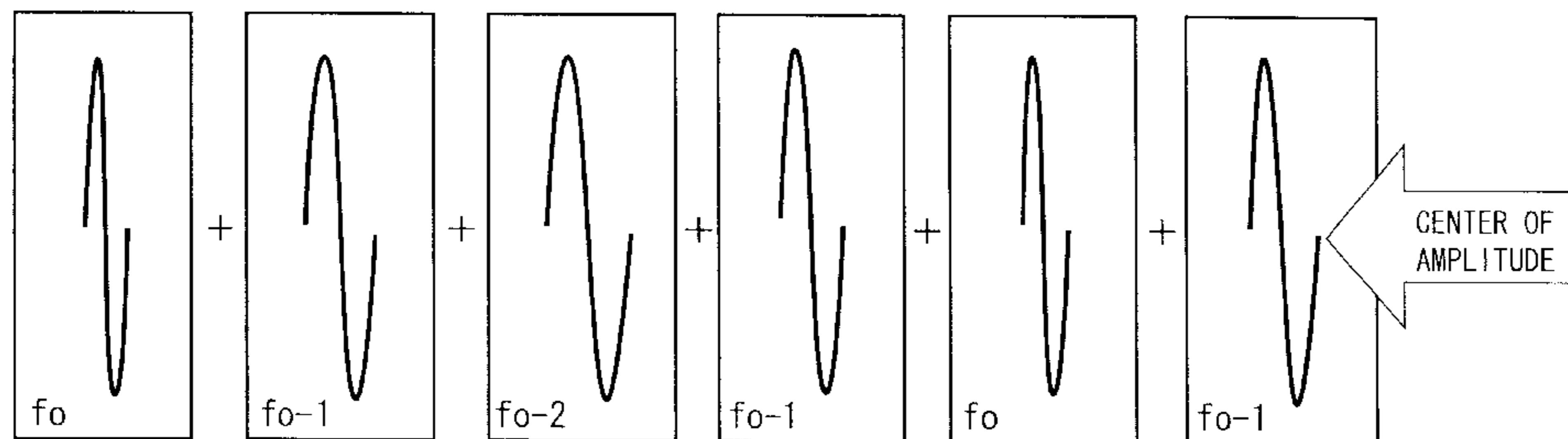
METHOD OF JOINING THE SWEEP WAVEFORM
