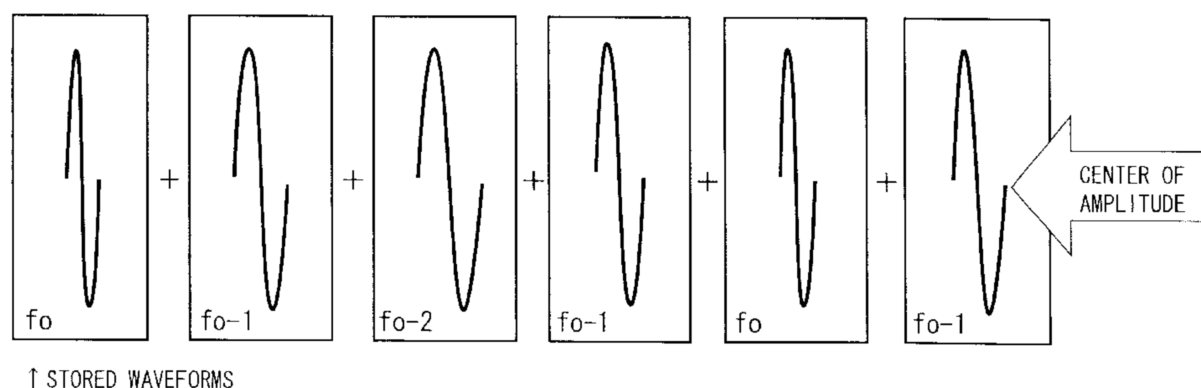
METHOD OF JOINING THE SWEEP WAVEFORM
