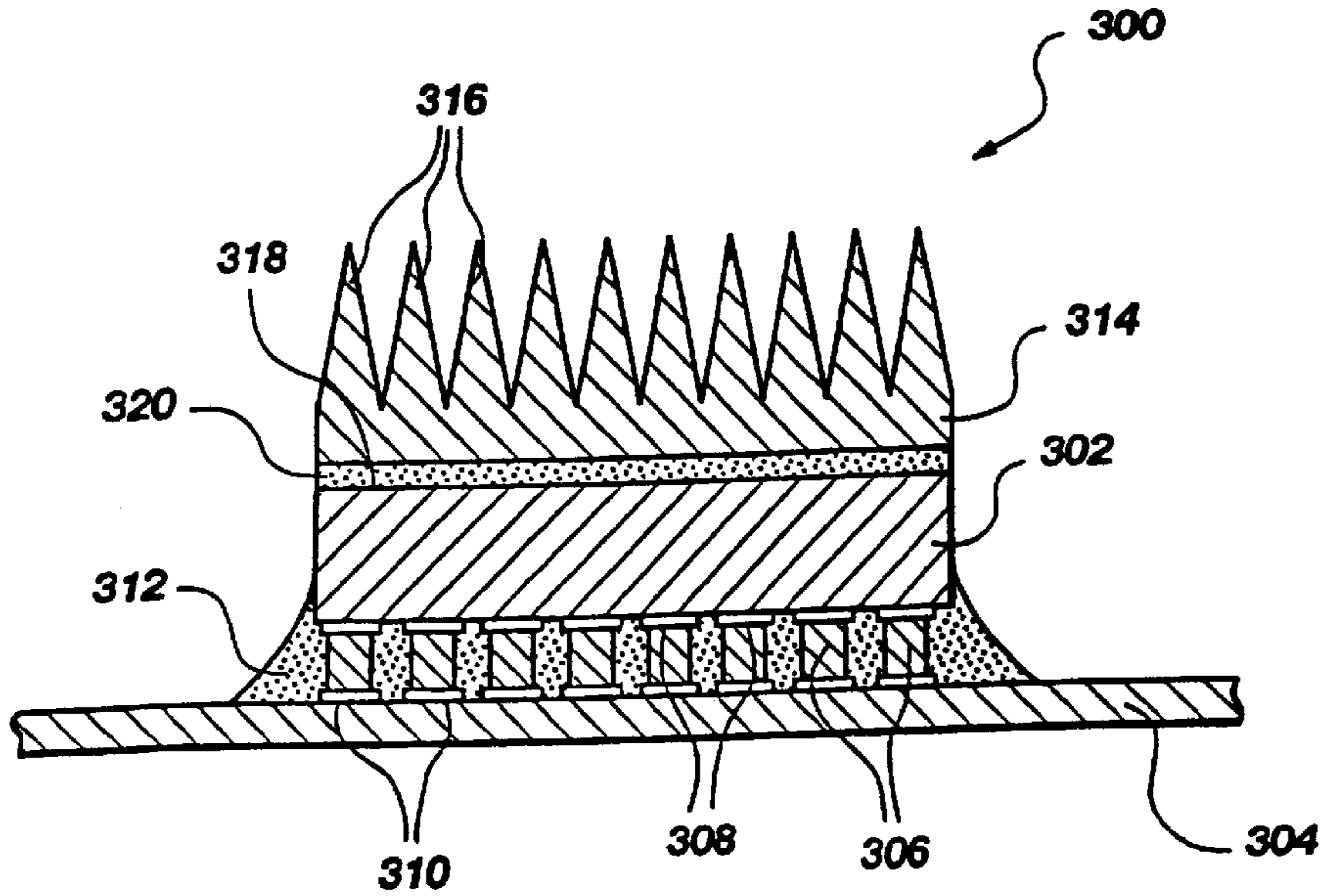
Fig. 3 PRIOR ART
