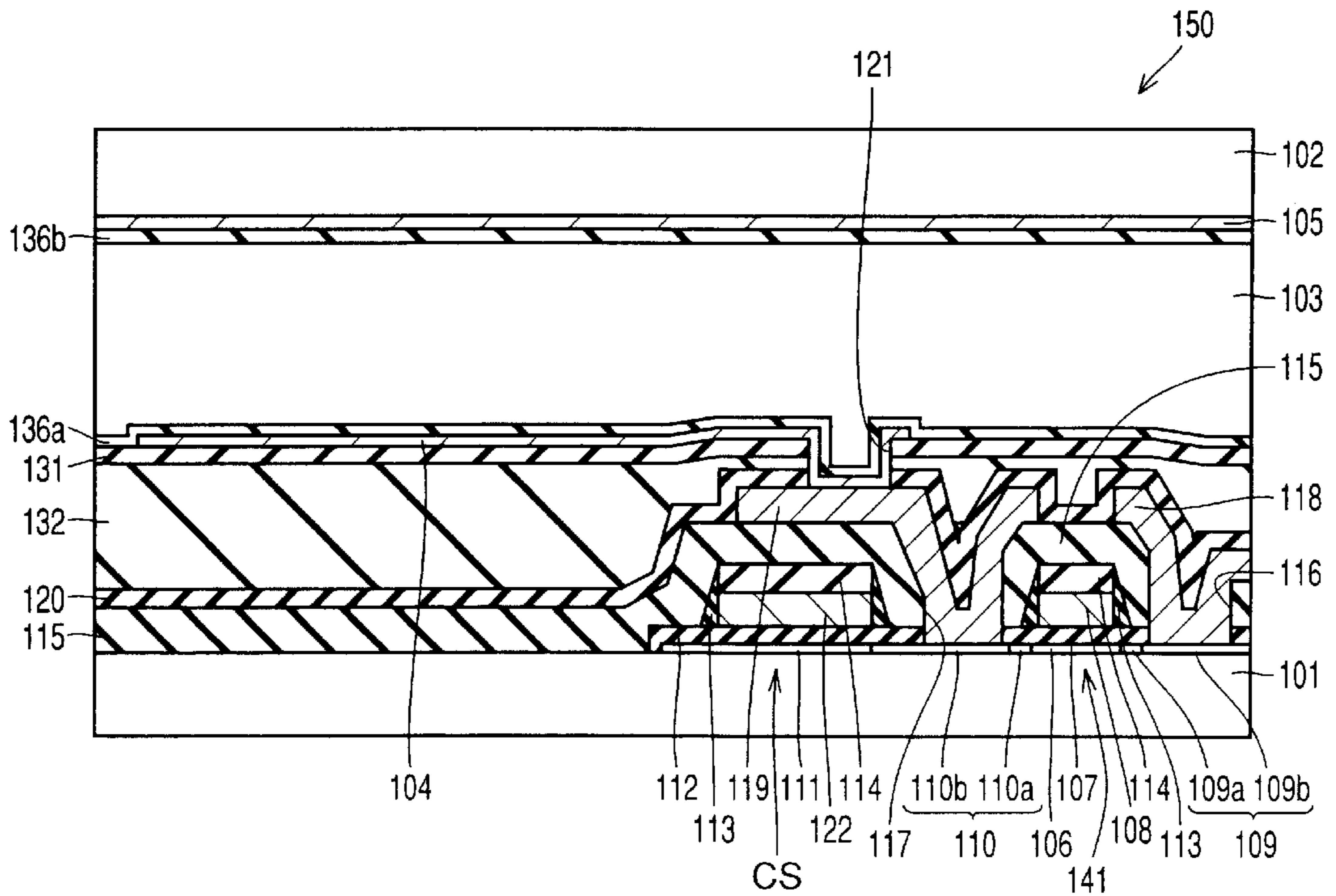
FIG. 10 PRIOR ART
