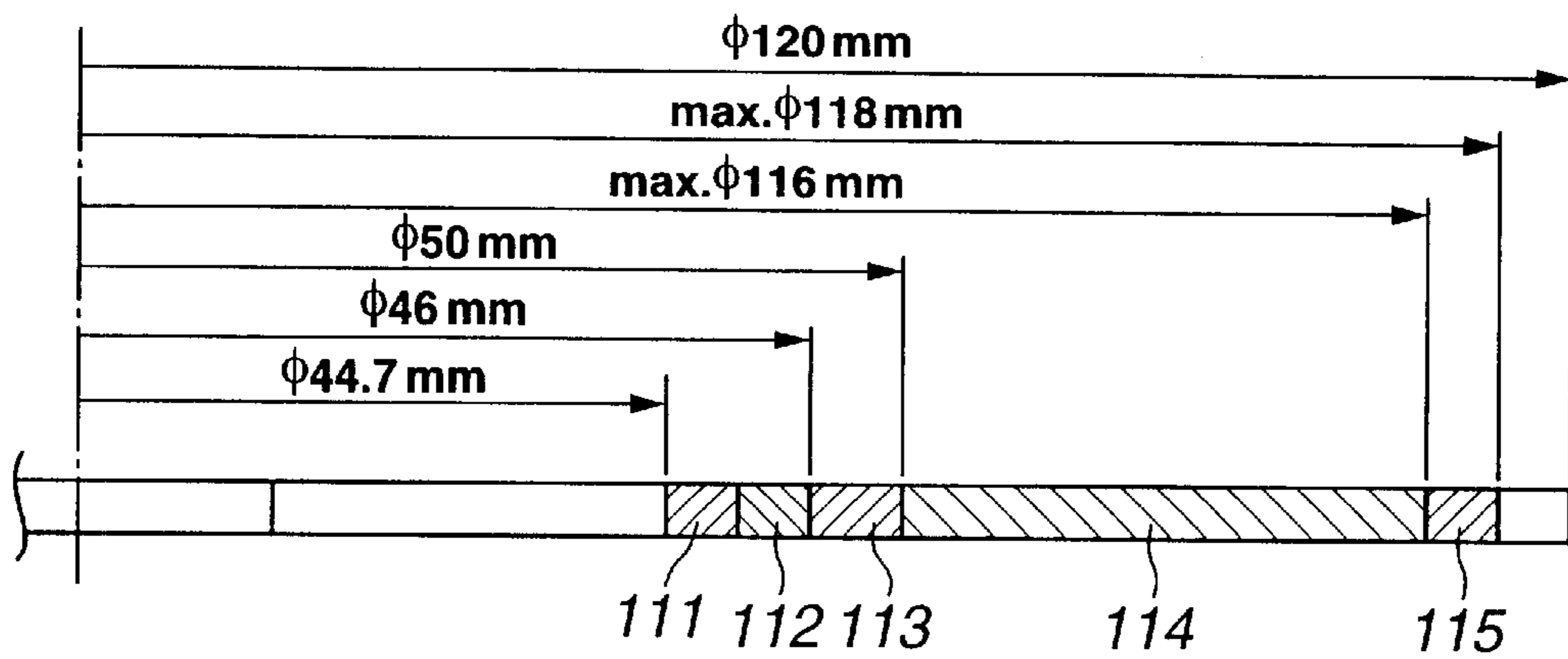
FIG.2A
