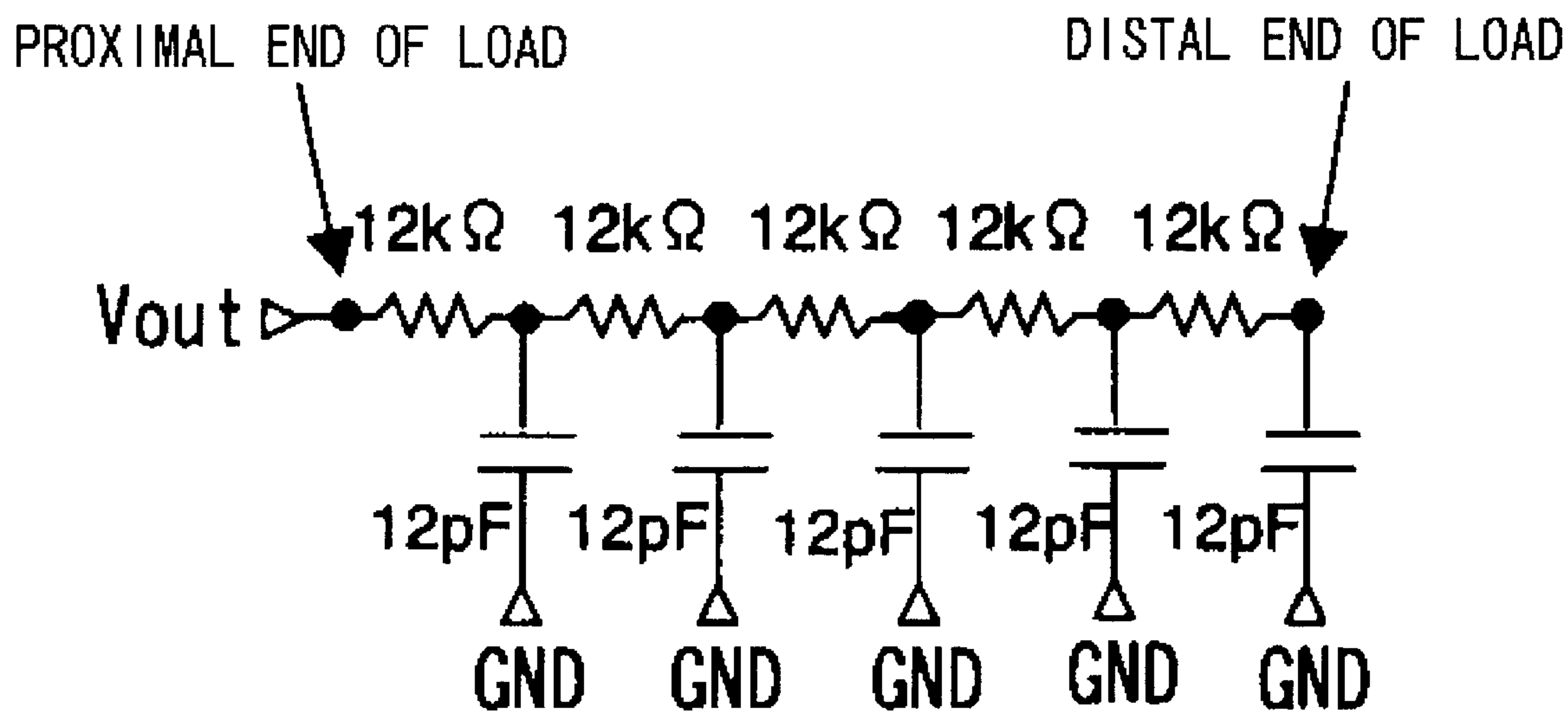
ONE DATA LINE LOAD EQUIVALENT CIRCUIT
