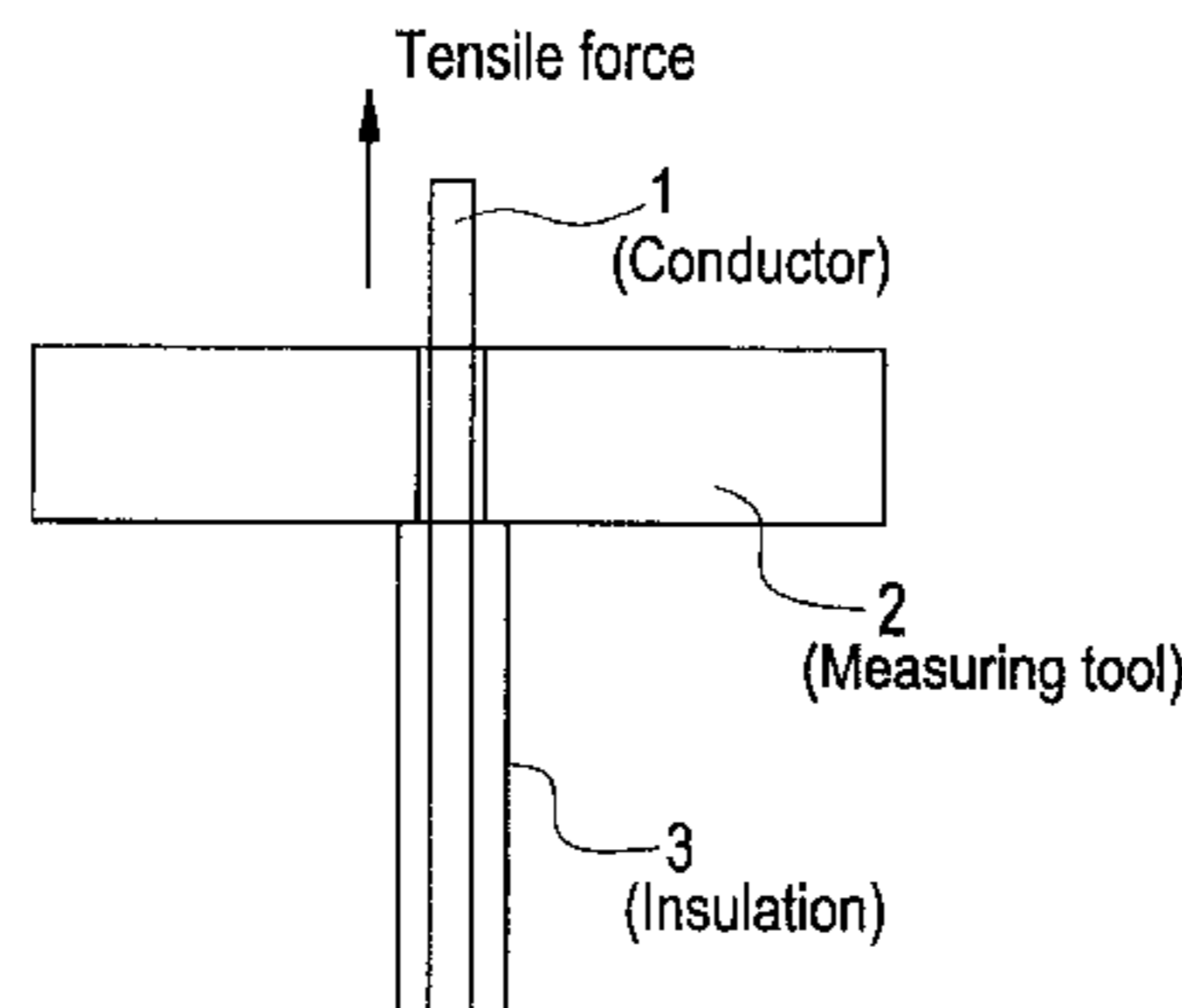
Measuring method of conductor stripping force
