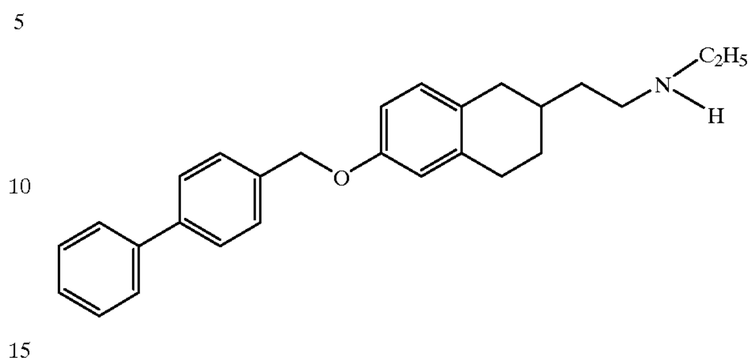
6-(4-Biphenyl)methoxy-2-[2-(N-ethylamino)ethyl]tetralin
