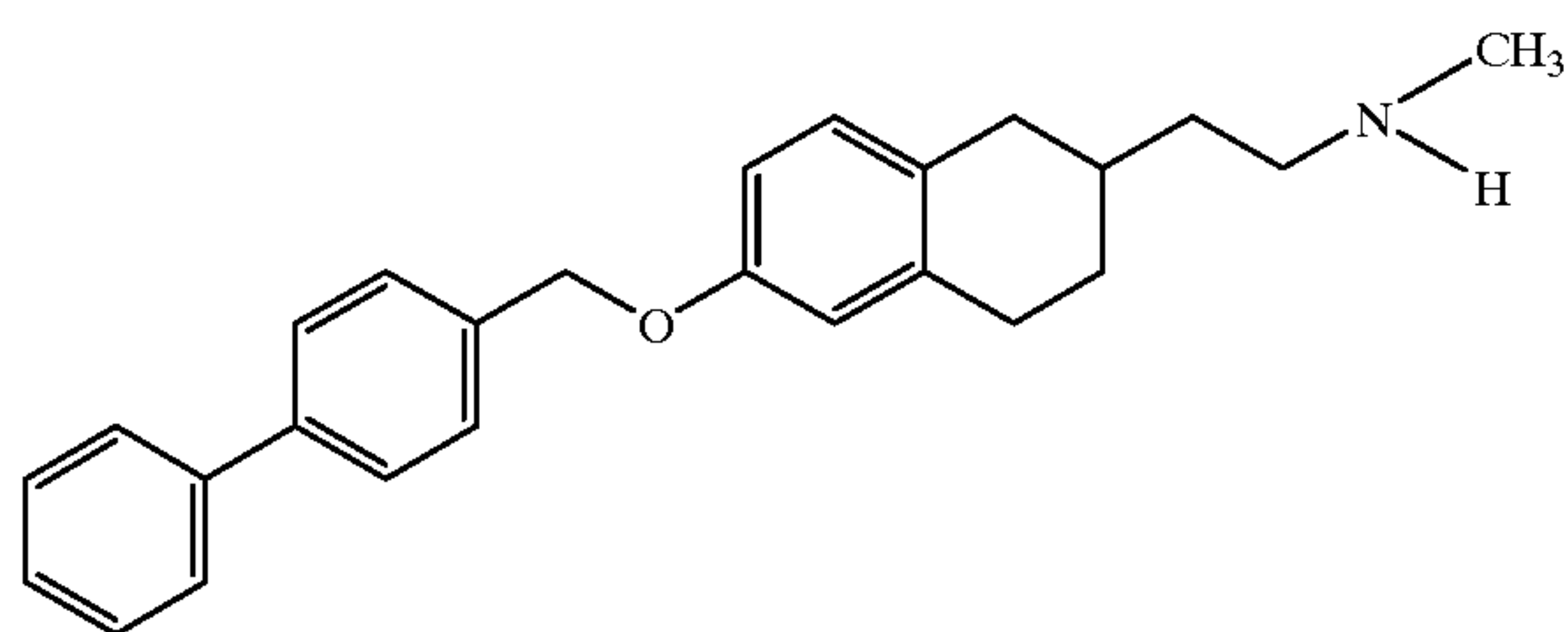
6-(4-Biphenyl)methoxy-2-[2-(N-methylamino)ethyl]tetralin
