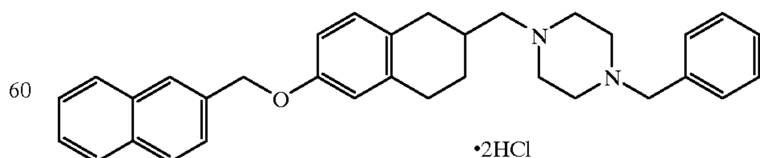
2-(4-Benzylpiperazin-1-yl)methyl-6-(2-naphthyl)methoxytetralin dihydrochloride
