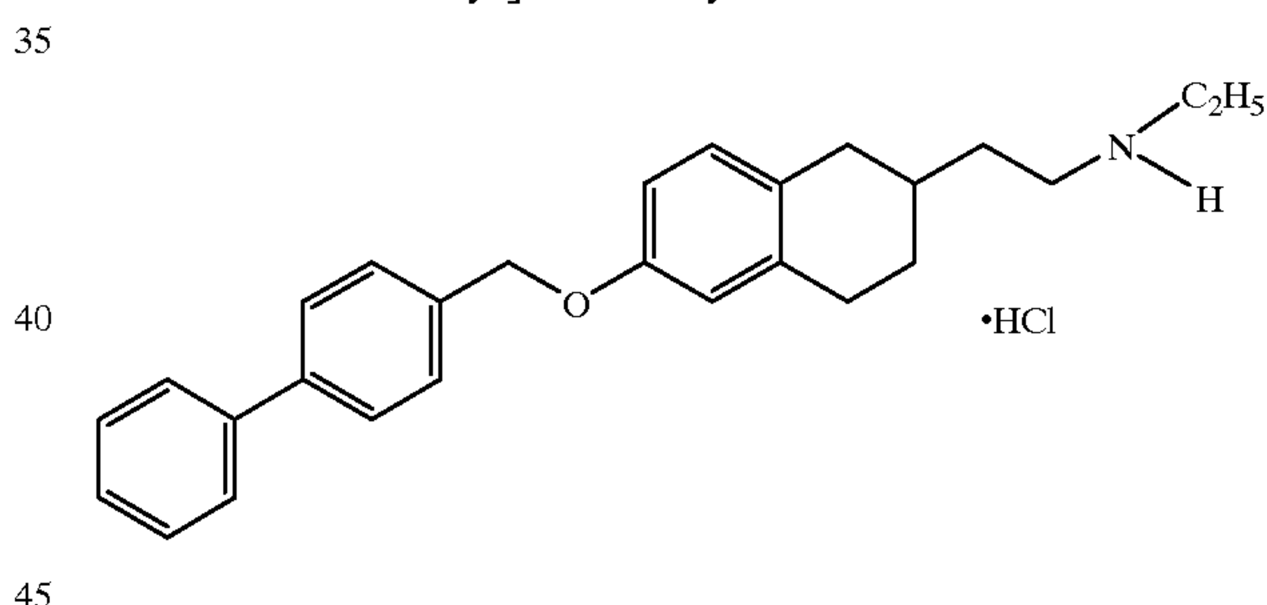
6-(4-Biphenyl)methoxy-2-[2-(N-ethylamino)ethyl]tetralin hydrochloride
