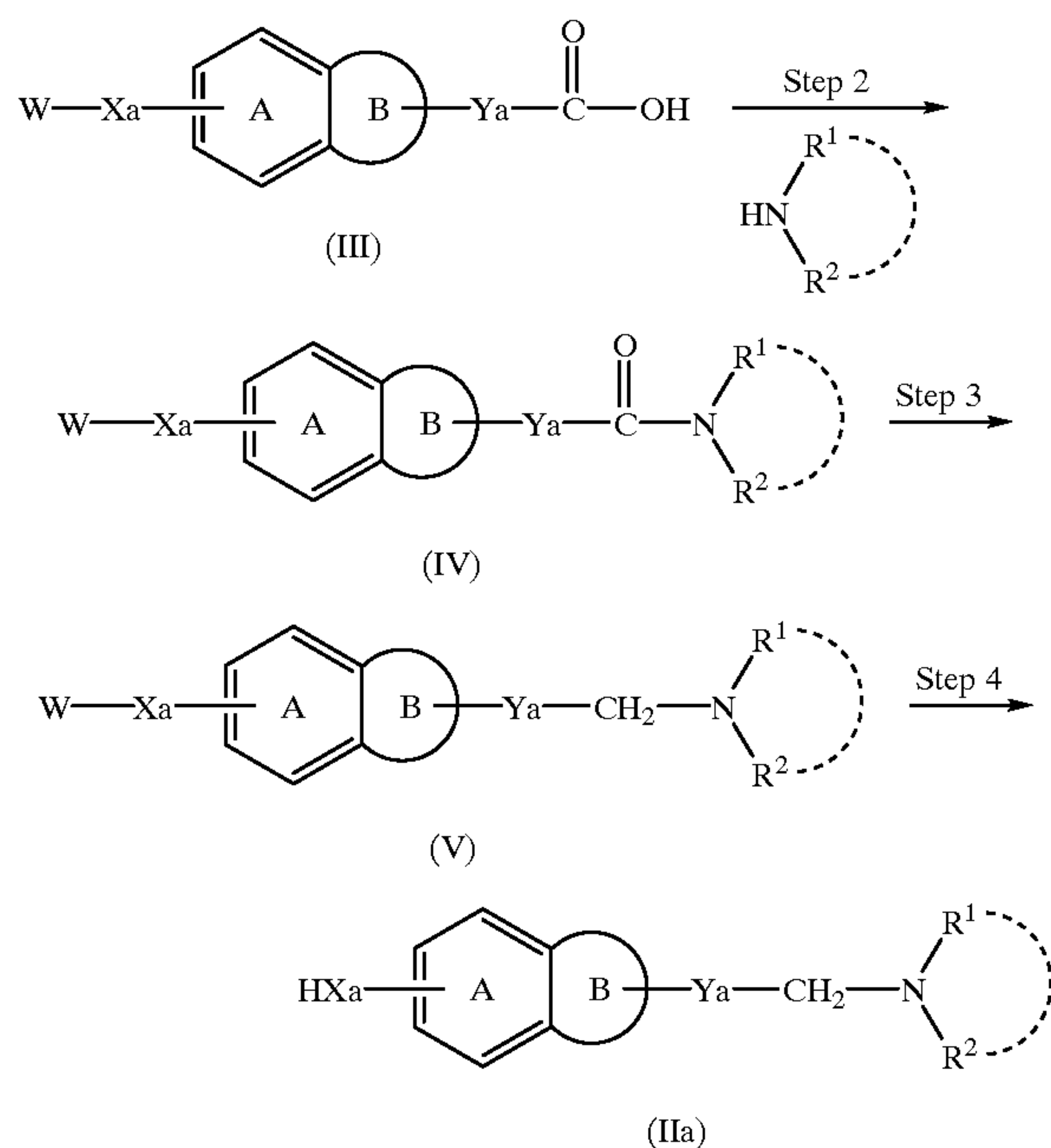
Scheme 2
