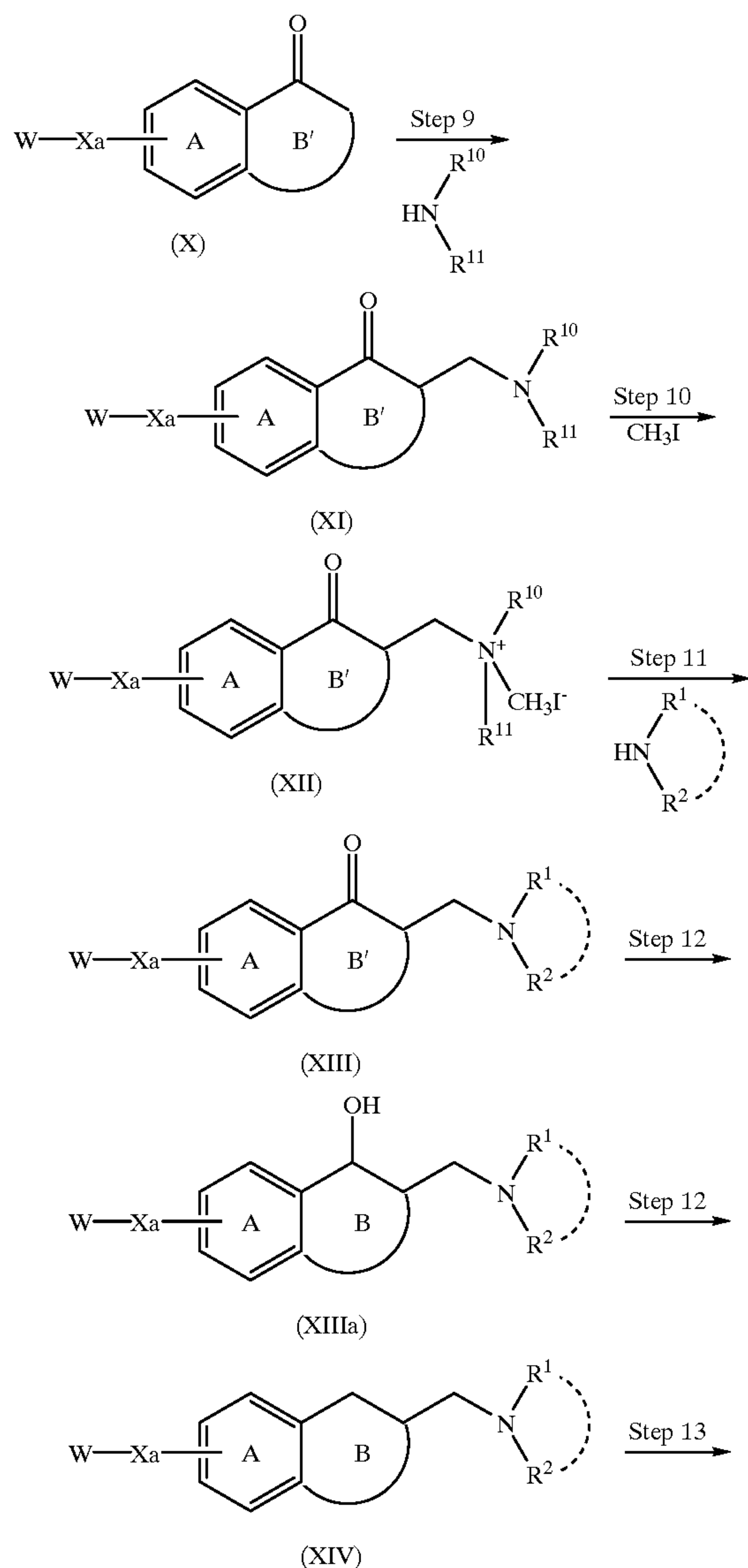
Scheme 4
