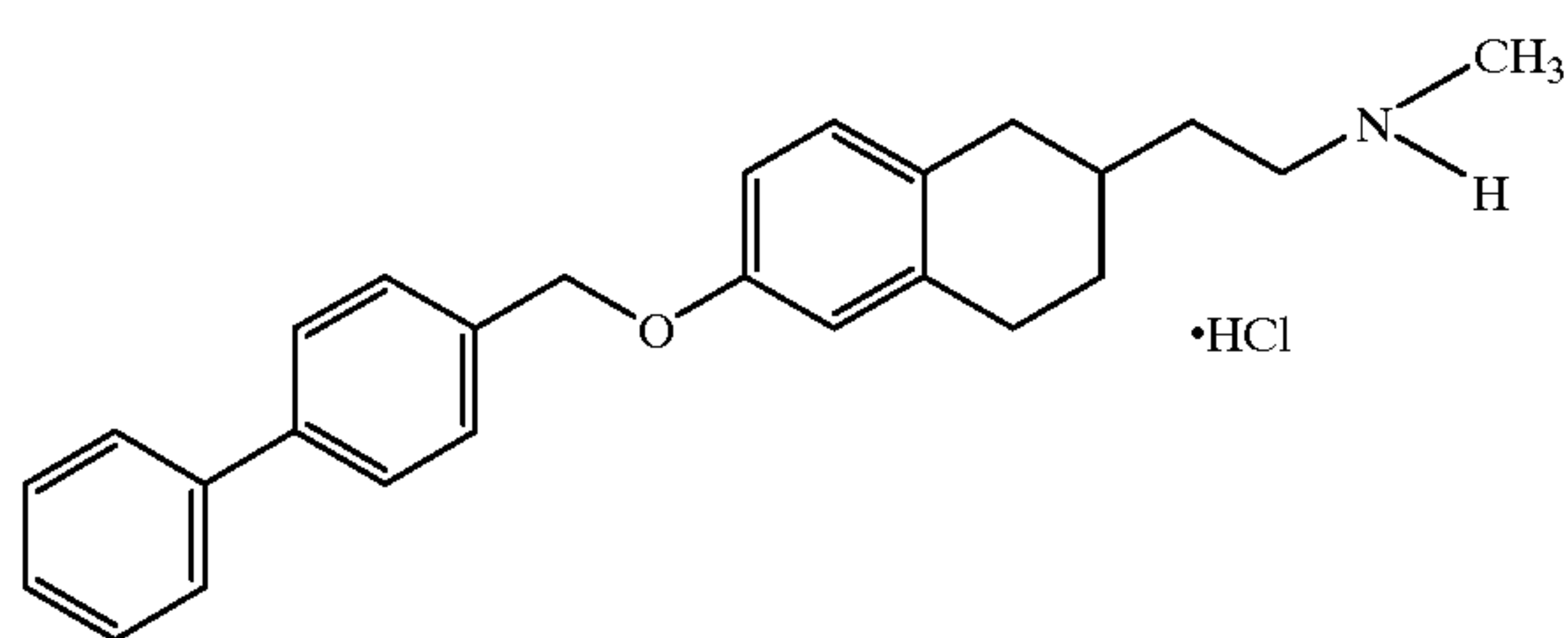
6-(4-Biphenyl)methoxy-2-[2-(N-methylamino)ethyl]tetralin hydrochloride
