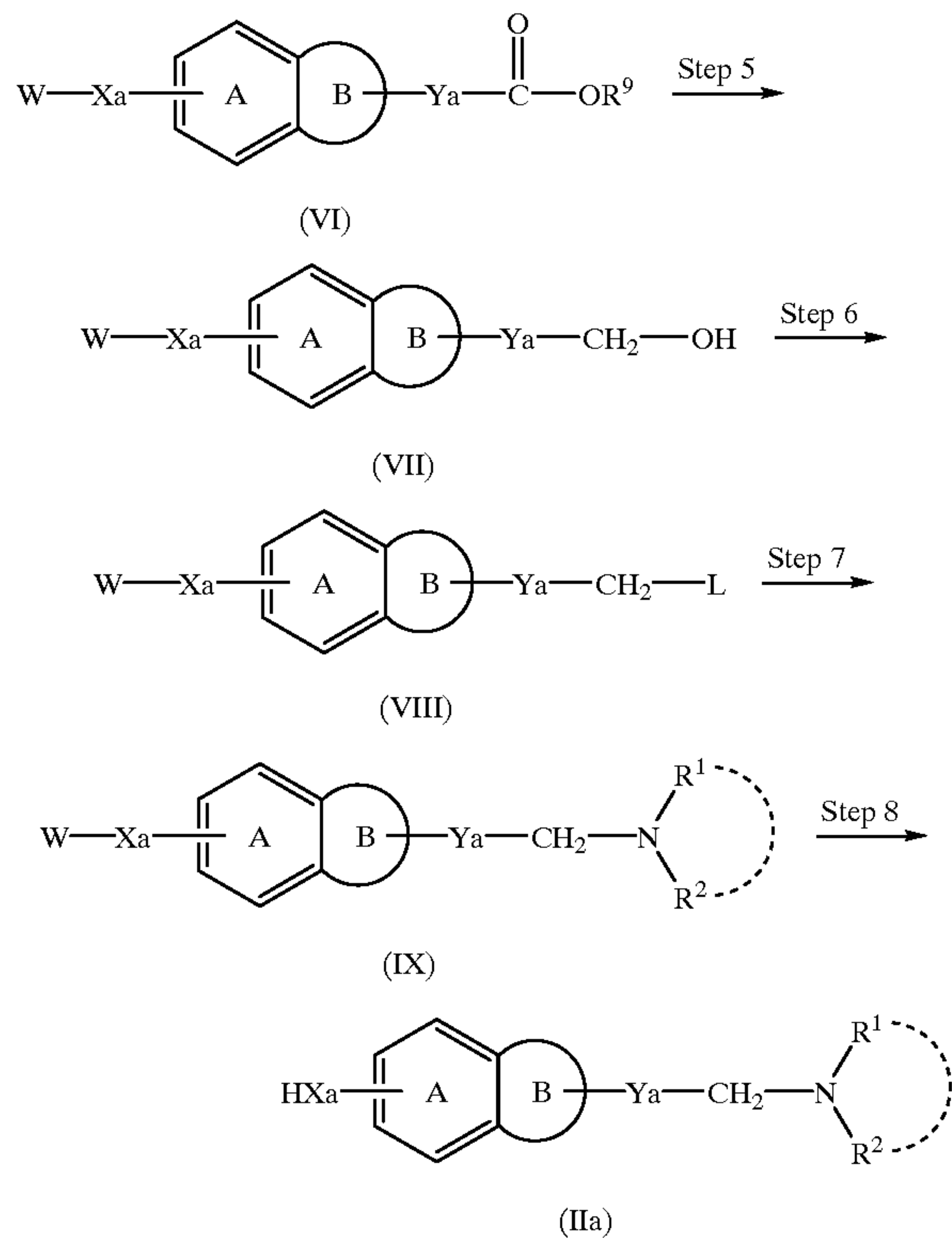
Scheme 3
