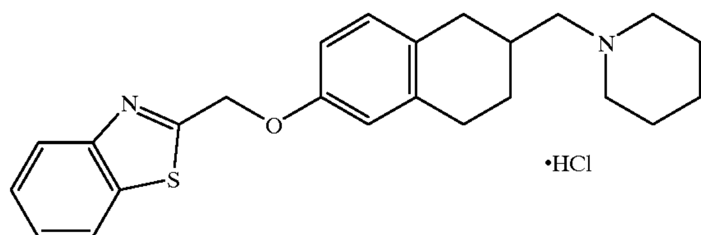
6-(2-Benzothiazolyl)methoxy-2-piperidinomethyltetralin hydrochloride
