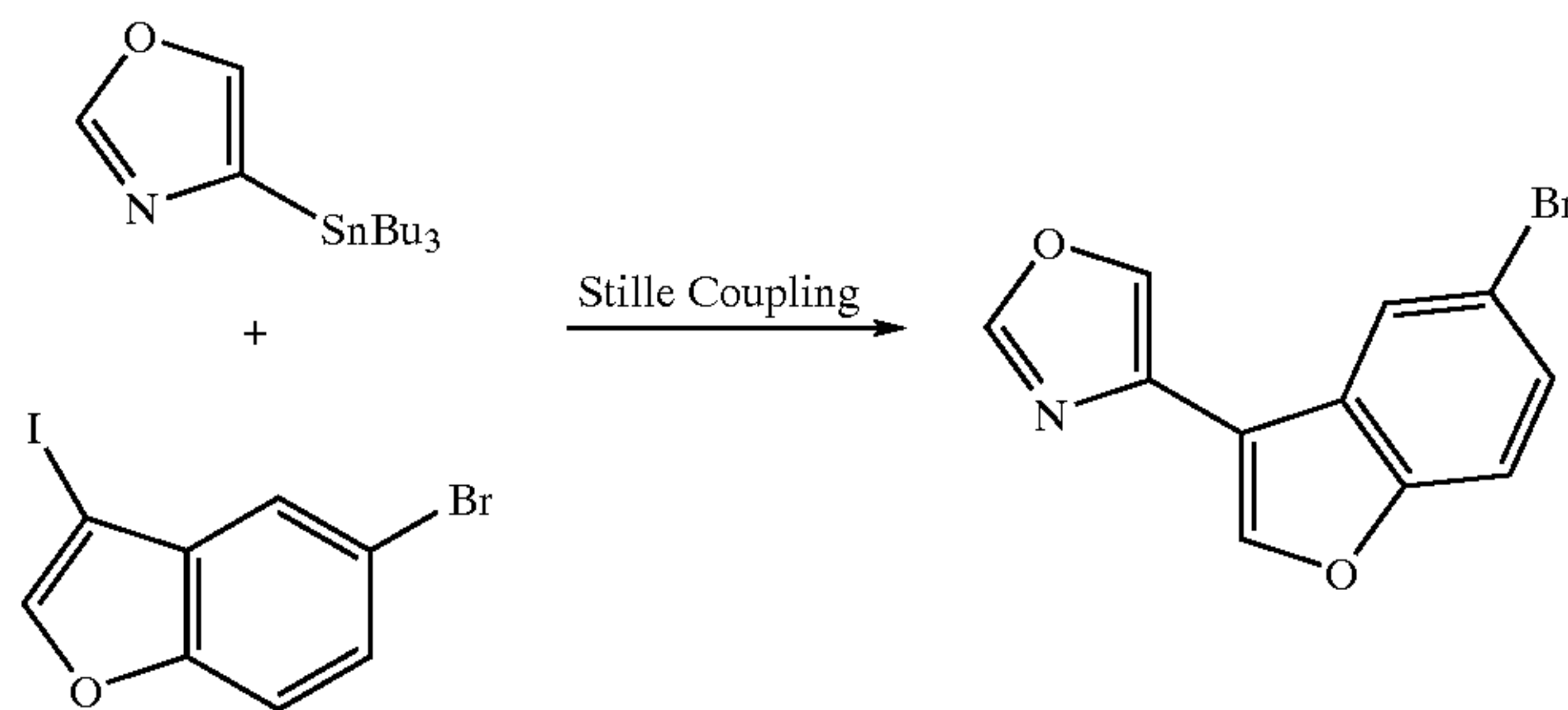
Stille Coupling No. 2
