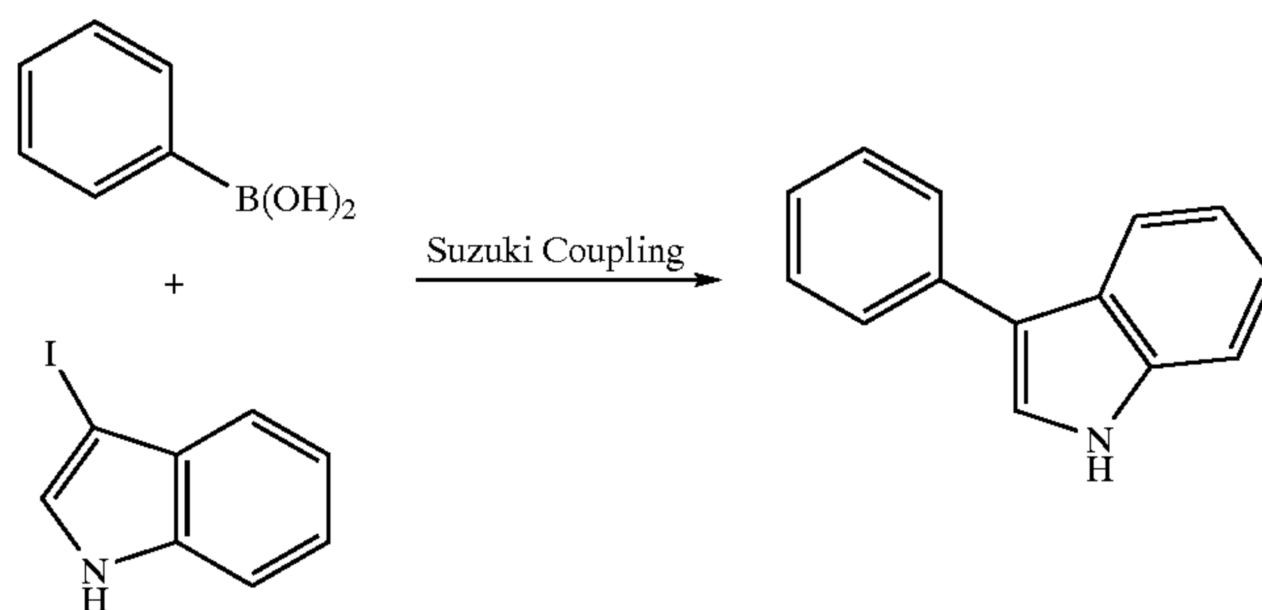
Suzuki Coupling No. 2:
