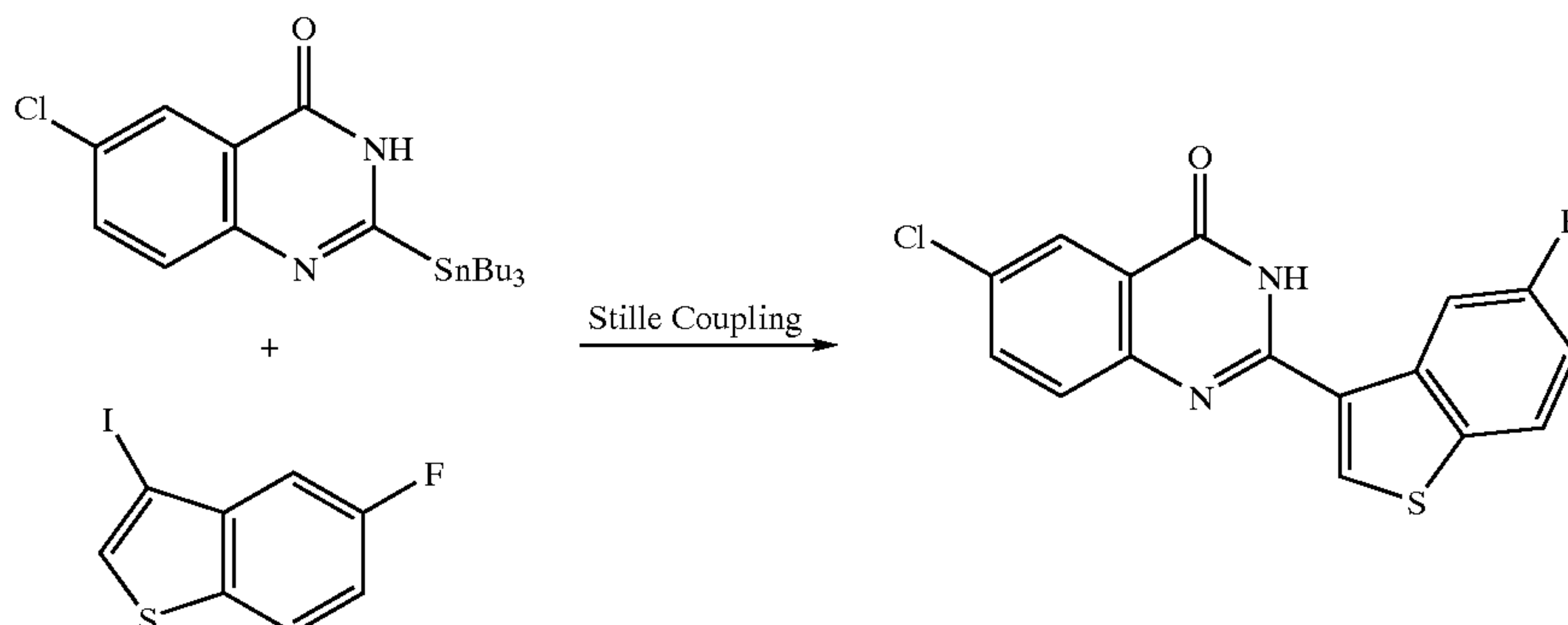
Stille Coupling No. 2
