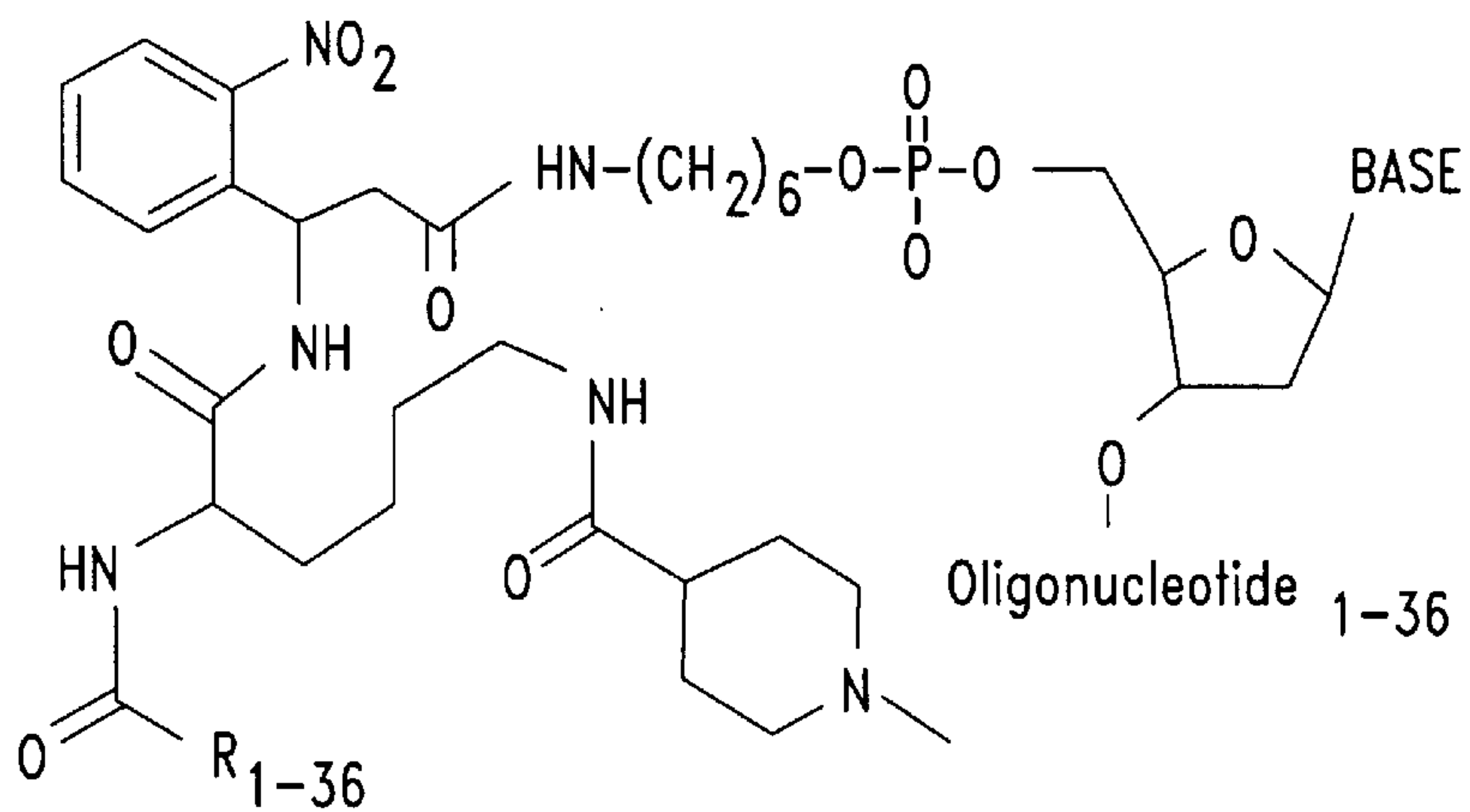
5'-CMST-Oligonucleotide Conjugate \text{XII}_{1-36}
