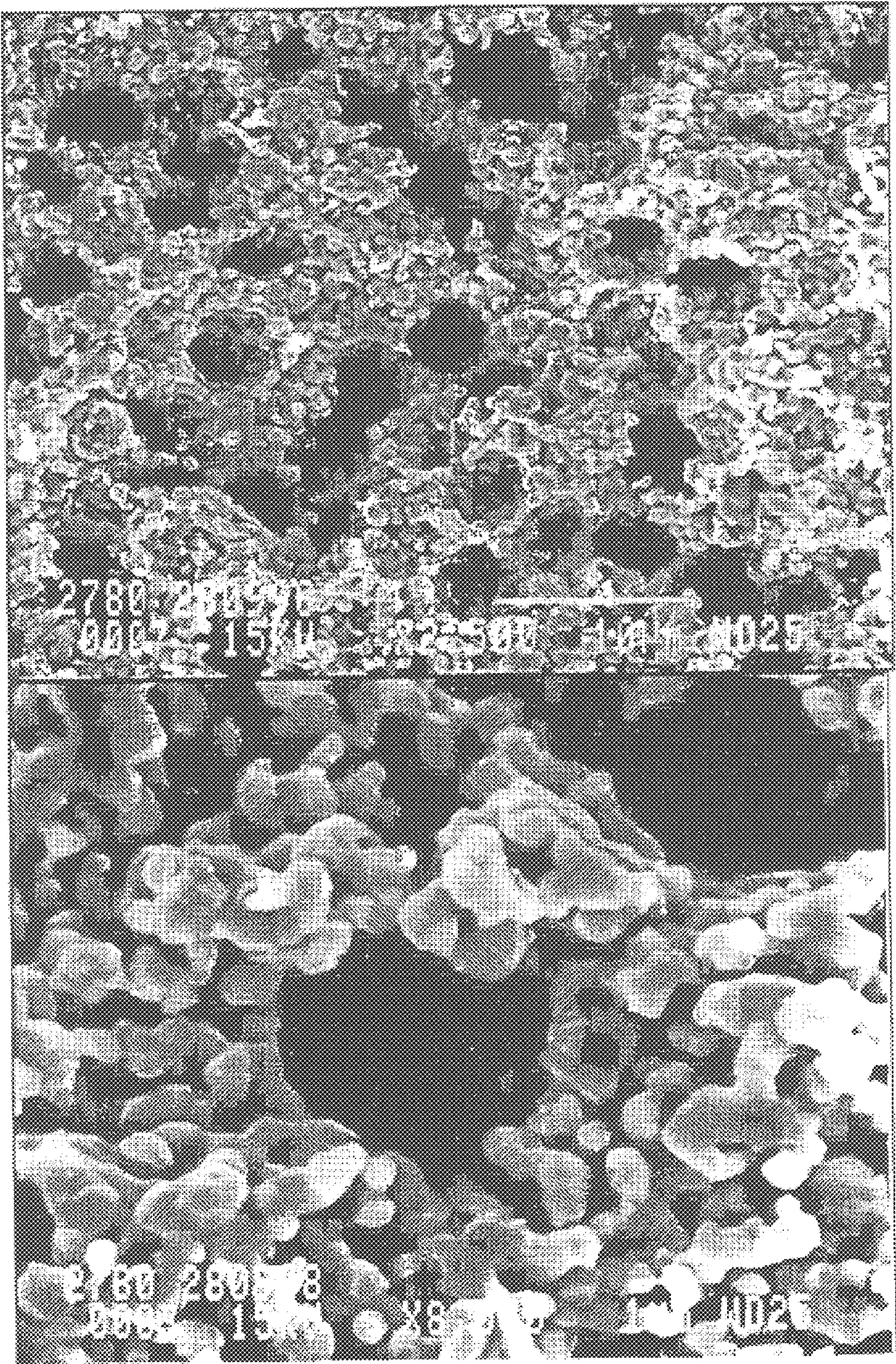
Figure 2. Micrograph of \text{La}_2\text{NiO}_4 Substrate sintered at 1100°C
