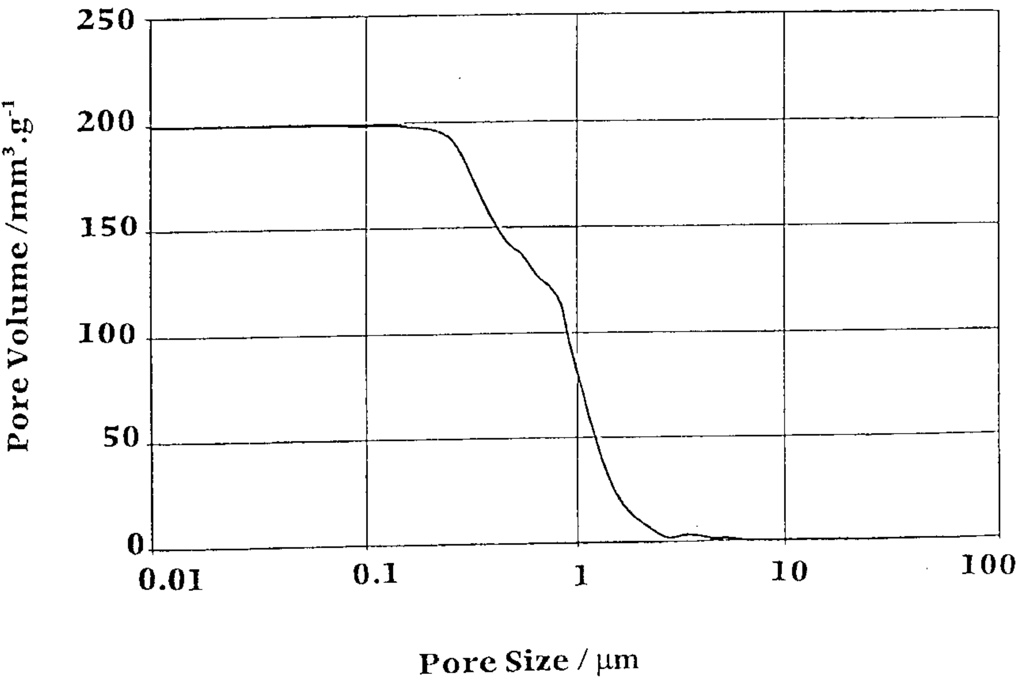
Pore Size Distribution in La 2 NiO 4 Substrate Sintered at 1100°C
