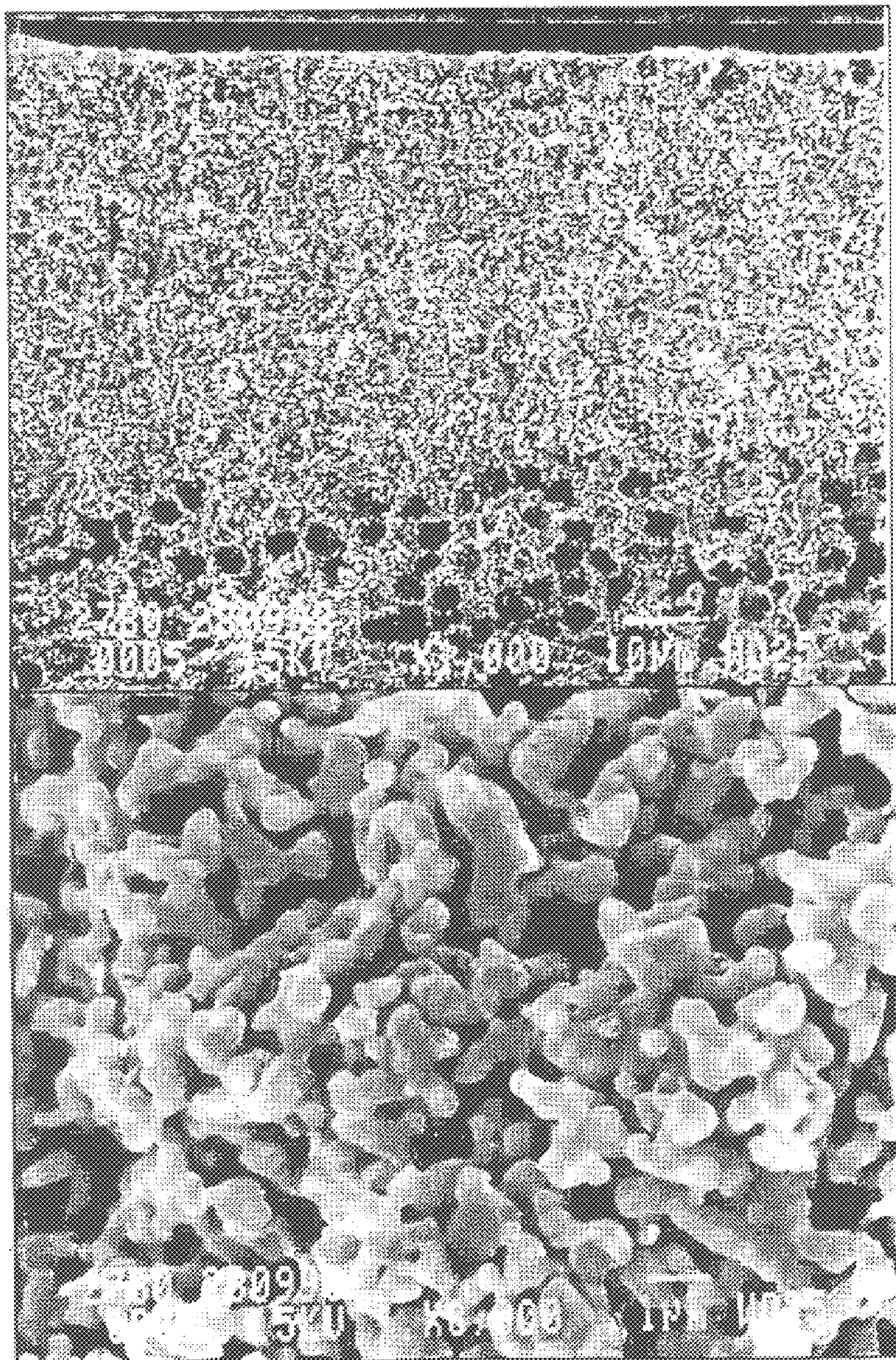
Figure 3. Micrograph of \text{La}_2\text{NiO}_4 Layer deposited onto porous substrate and sintered at 1100^\circ\text{C}
