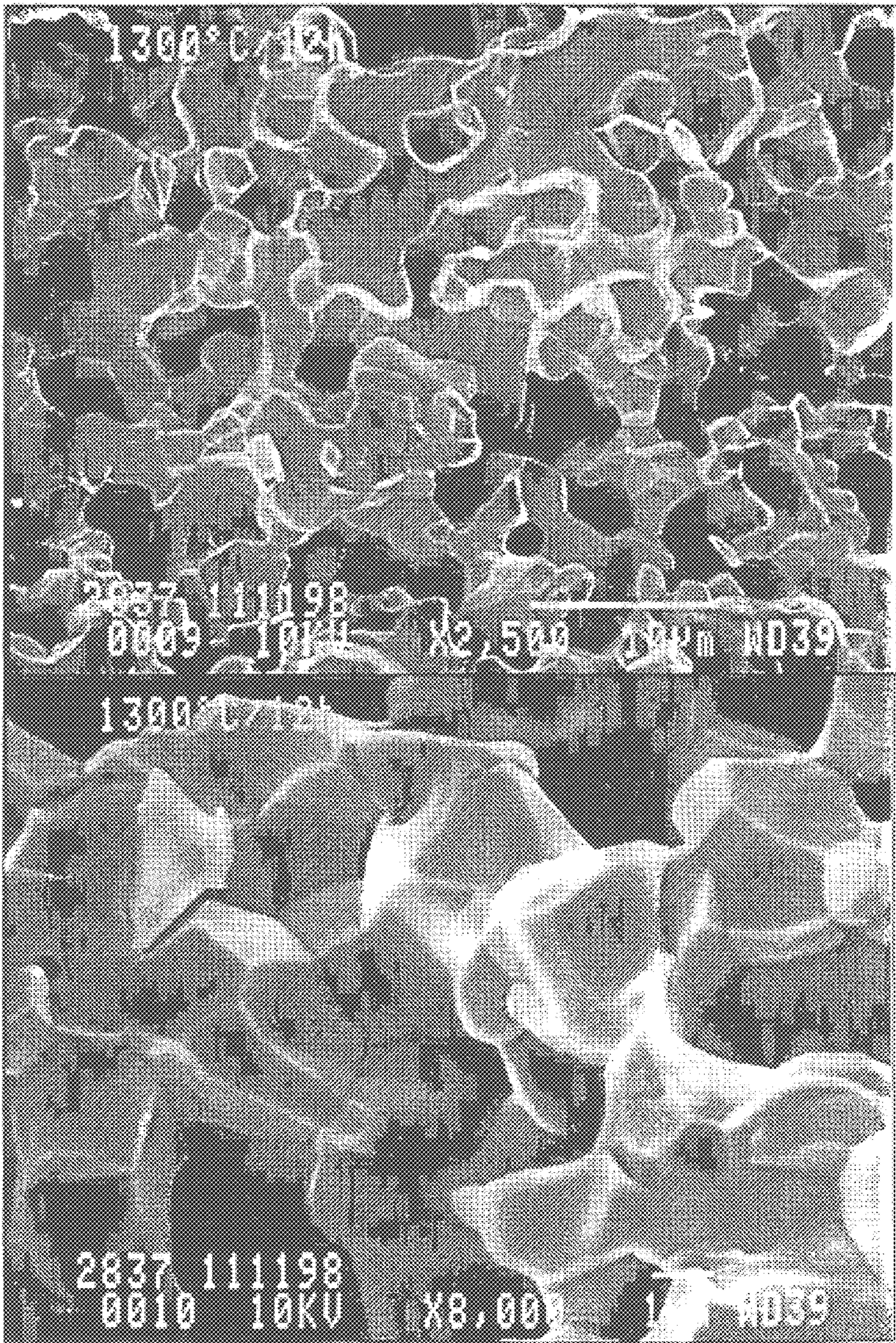
Figure 5. Micrograph of \text{La}_2\text{NiO}_4 Substrate sintered at 1300°C
