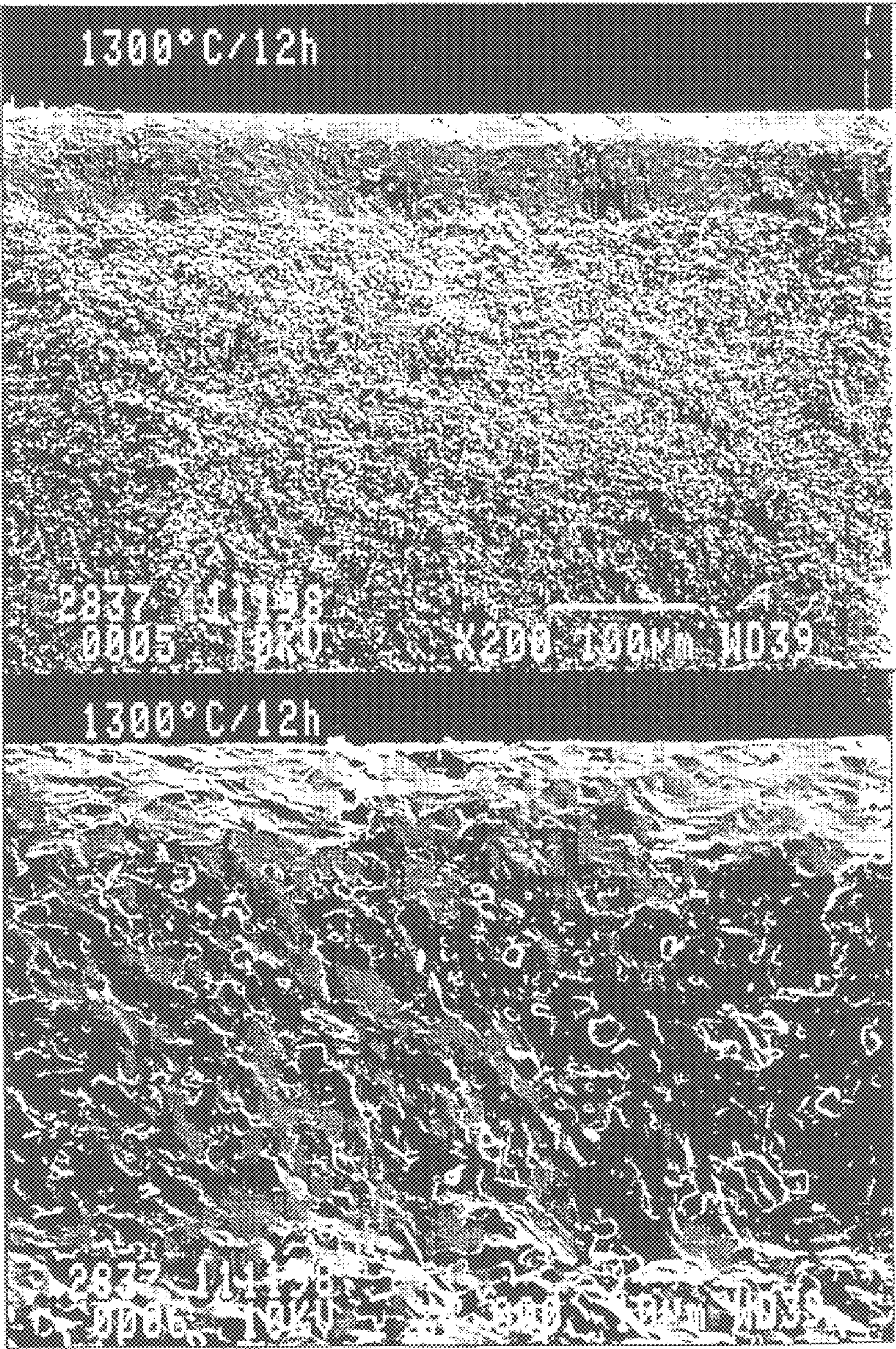
Figure 7. Micrograph of \text{La}_2\text{NiO}_4 Film and substrate sintered at 1300°C
