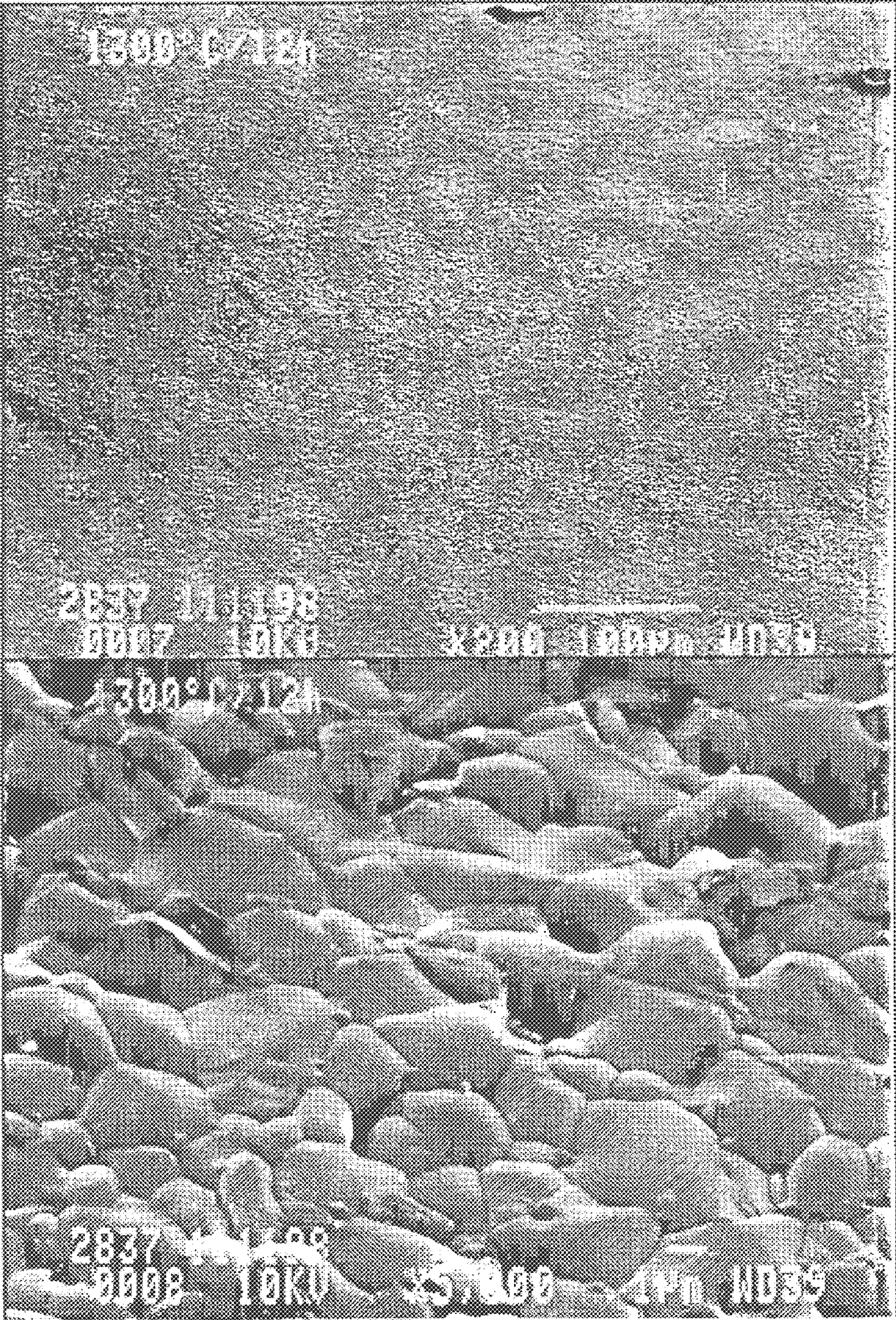
Figure 8. Micrograph of \text{La}_2\text{NiO}_4 Film sintered at 1300°C
