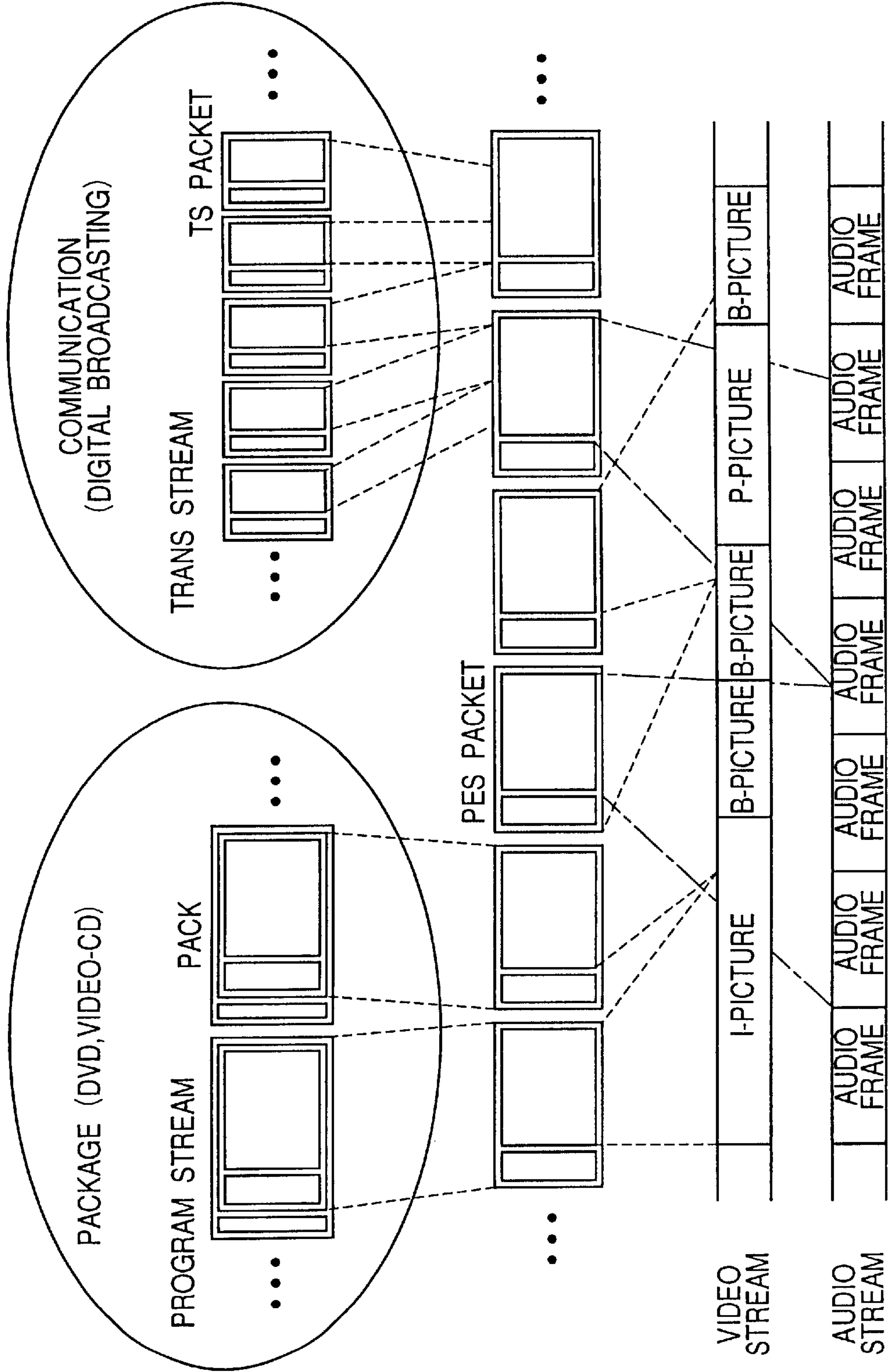
Fig.5 PRIOR ART
