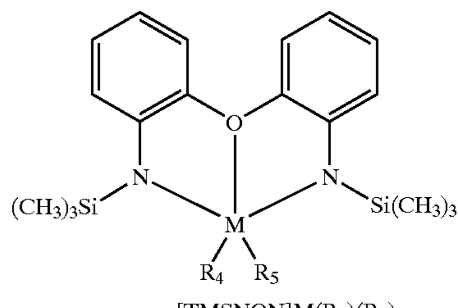
[TMSNON]M(R 4 )(R 5 )
