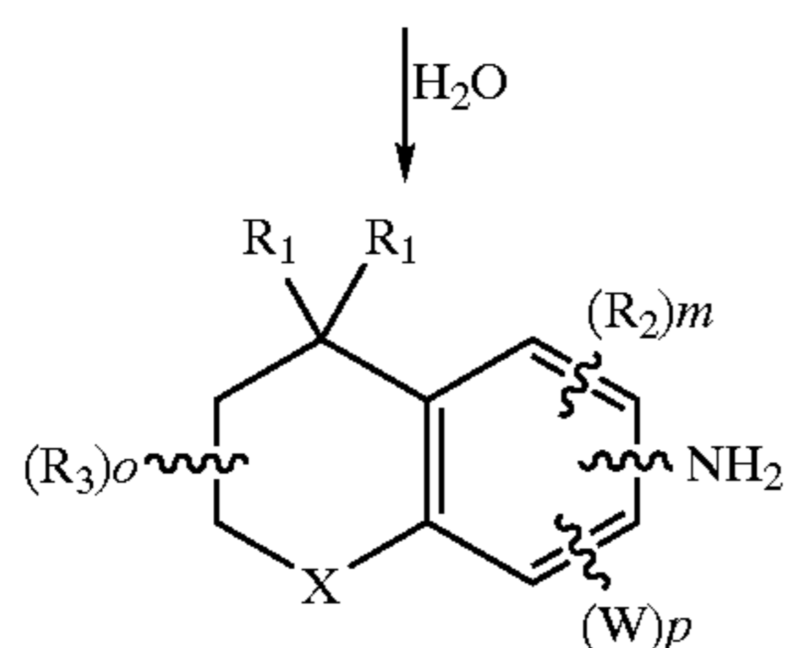
Formula 6 a
