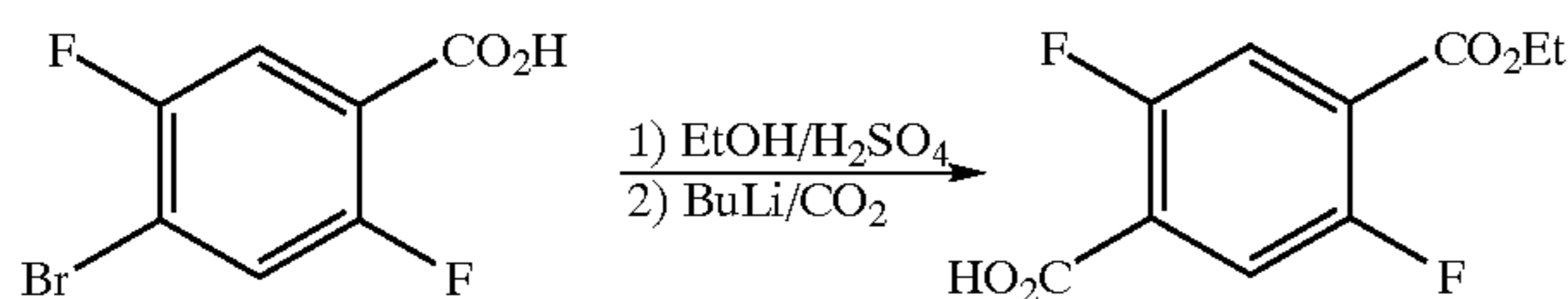
Reaction Scheme 12
