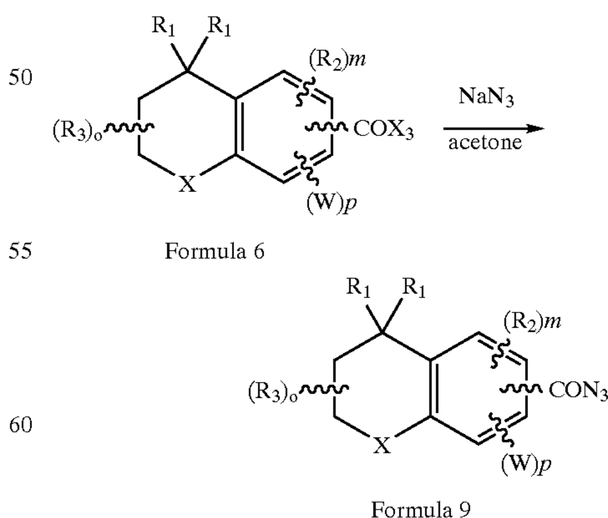
Reaction Scheme 11
