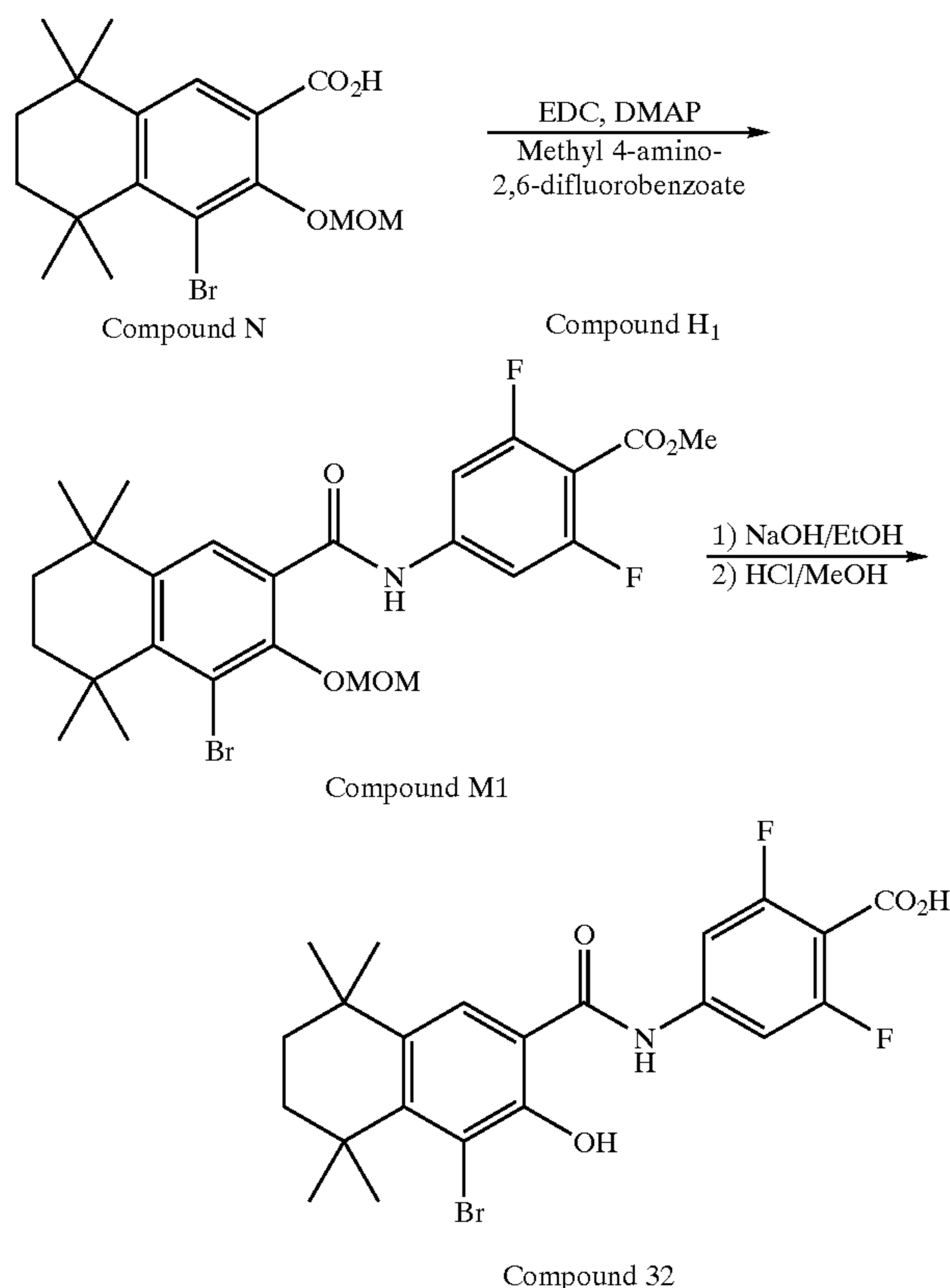
Reaction Scheme 9
