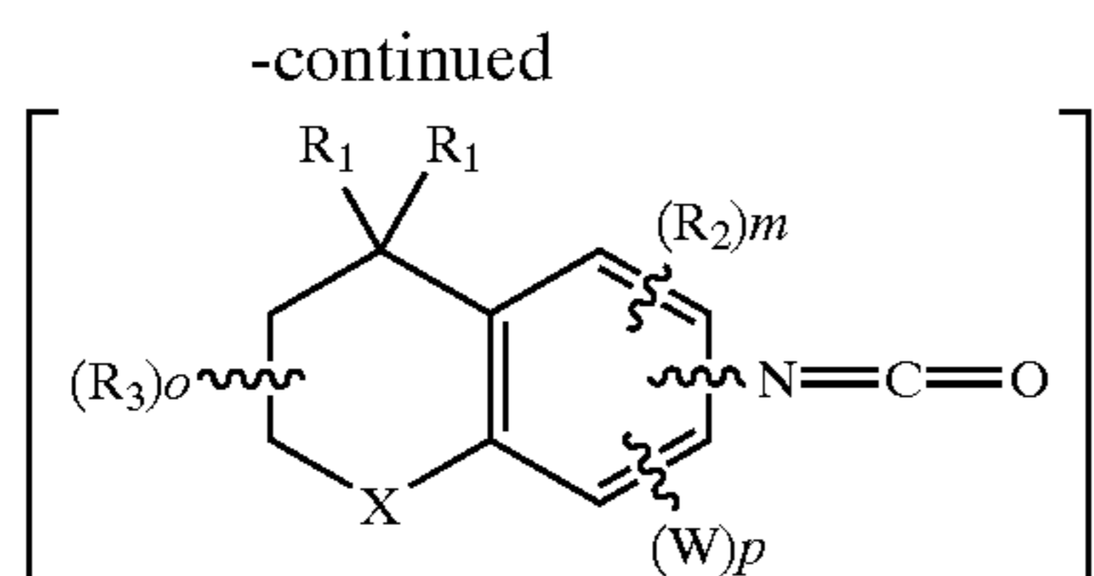
Formula 10
