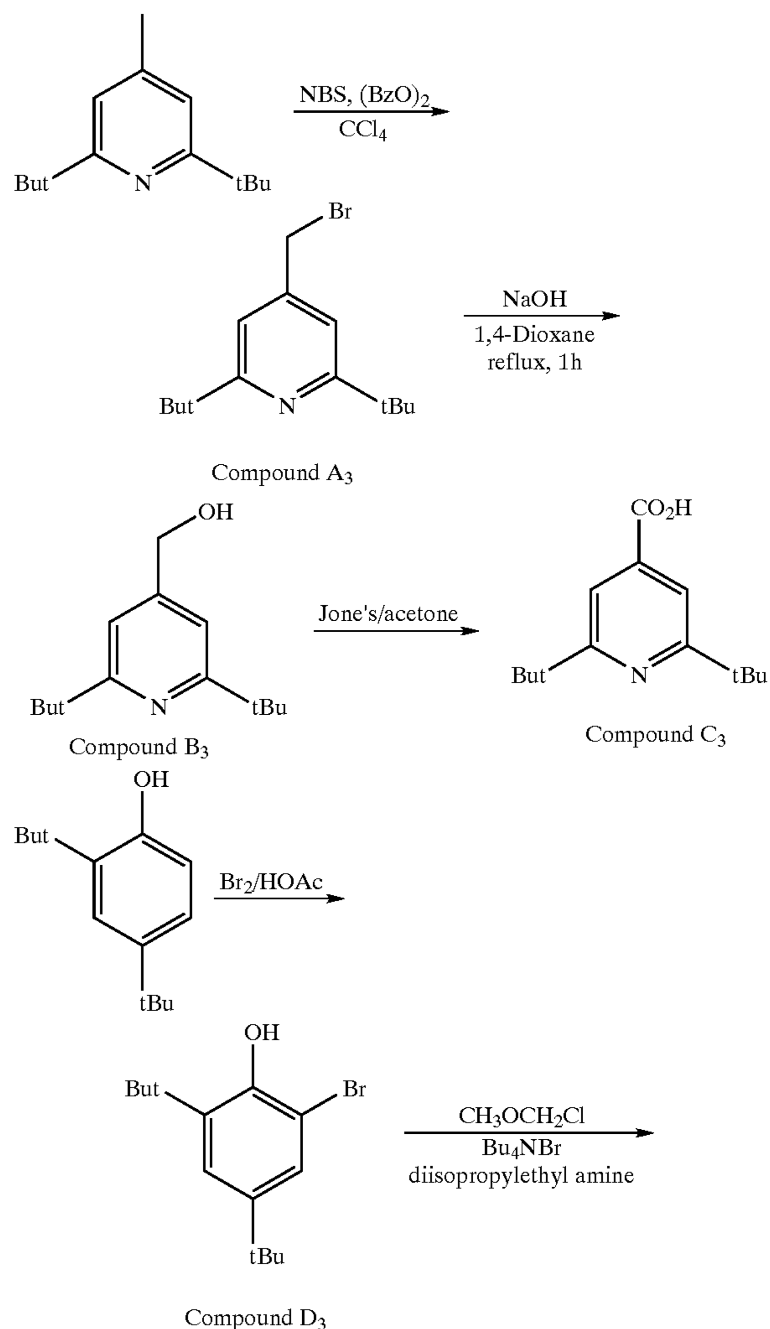
Reaction Scheme 13
