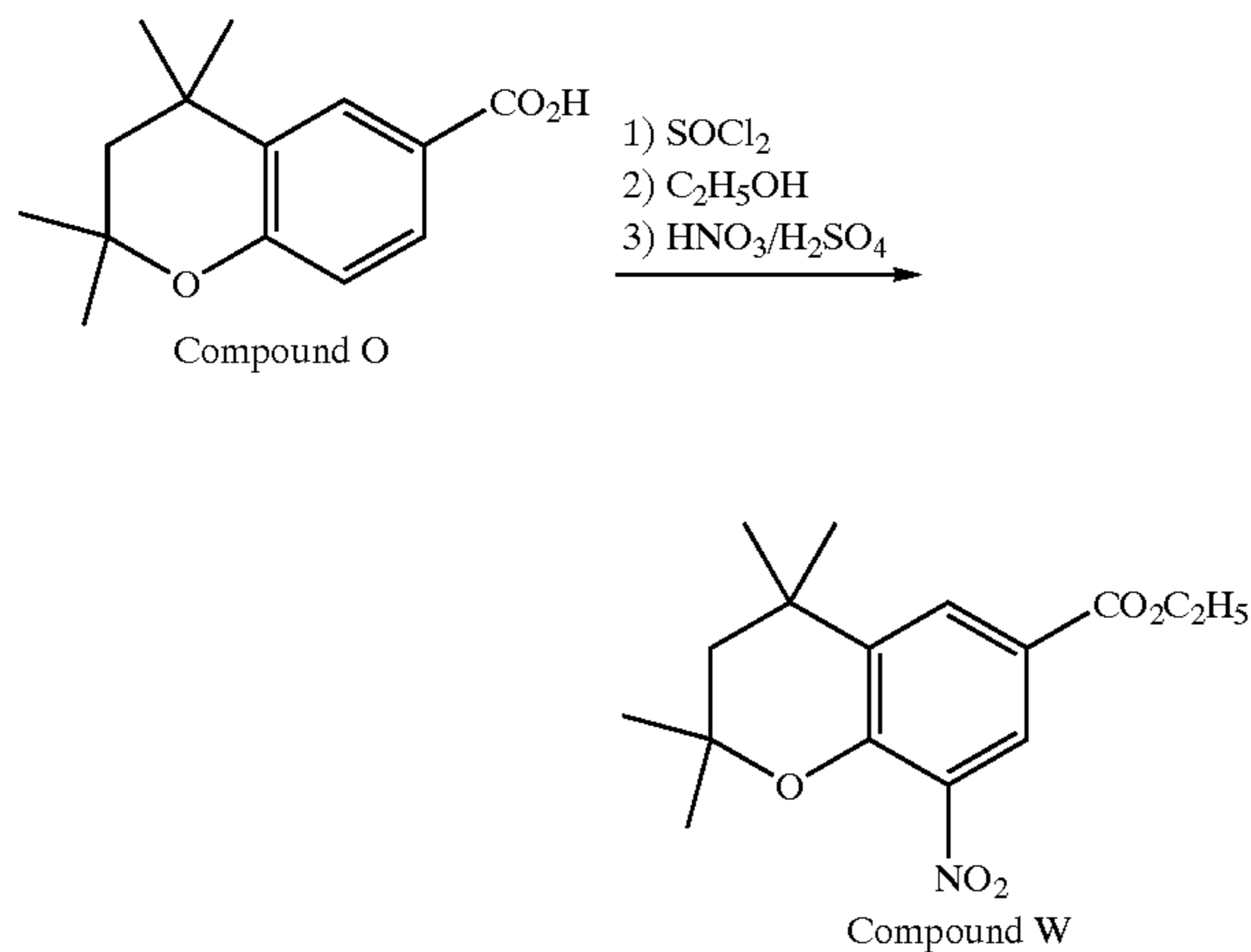
Reaction Scheme 3
