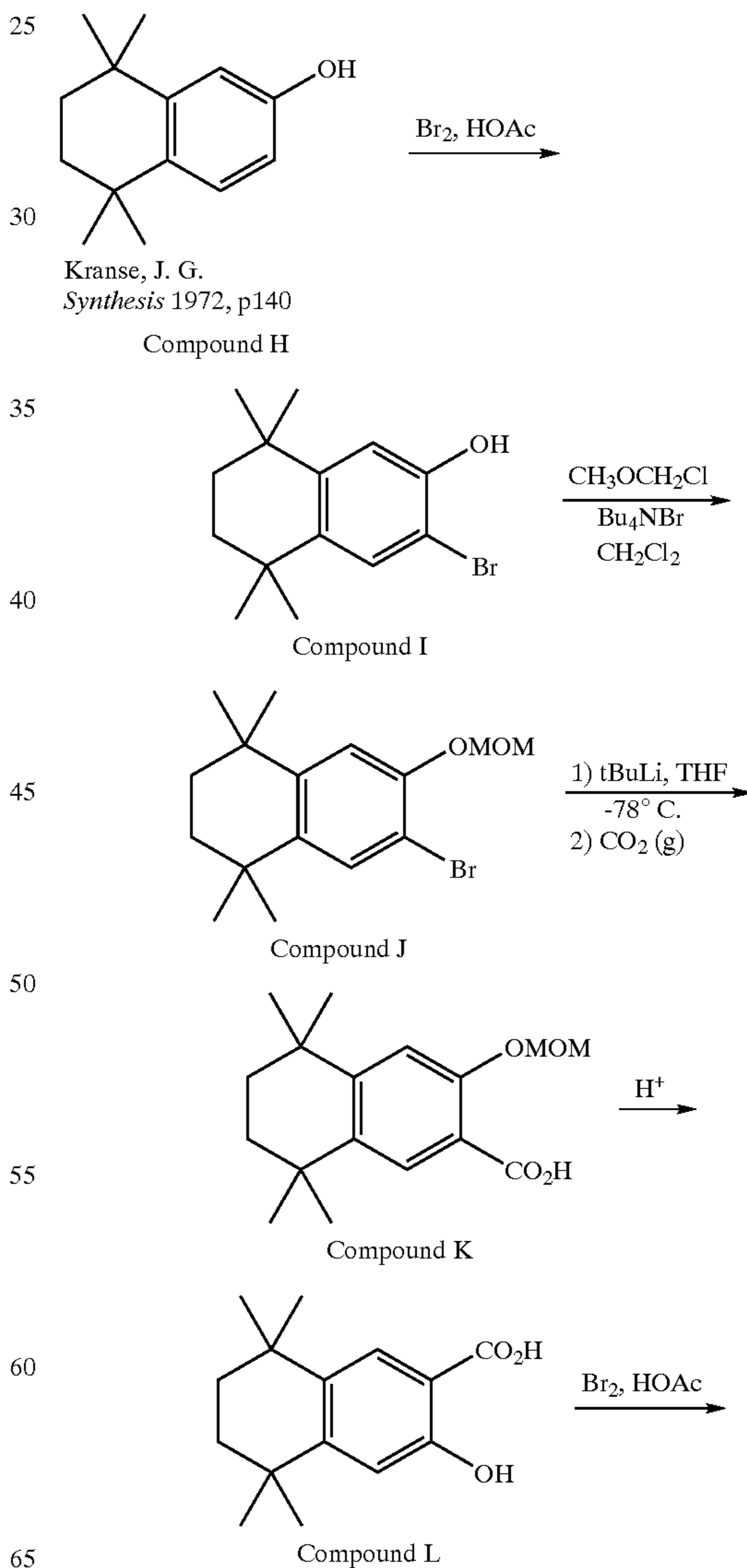
Reaction Scheme 2
