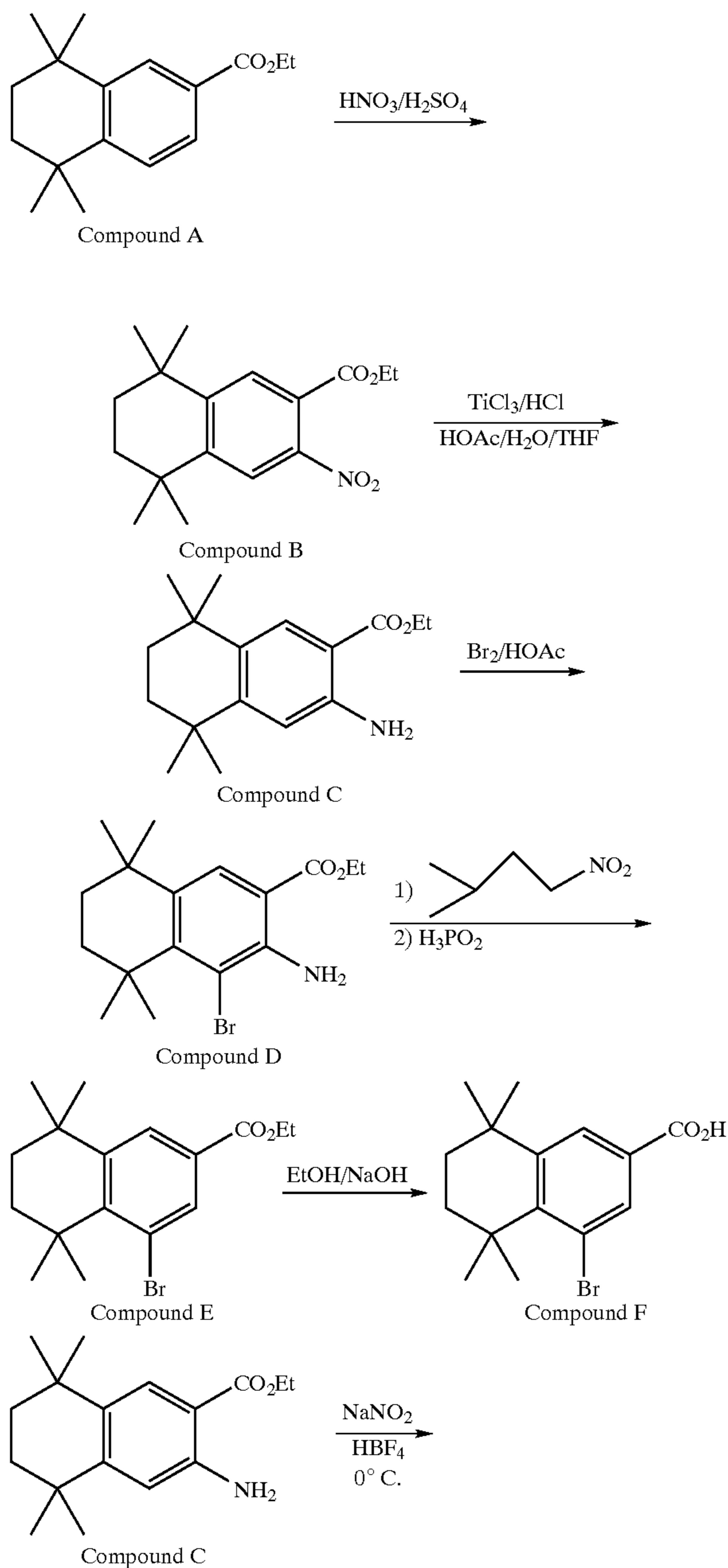
Reaction Scheme 1
