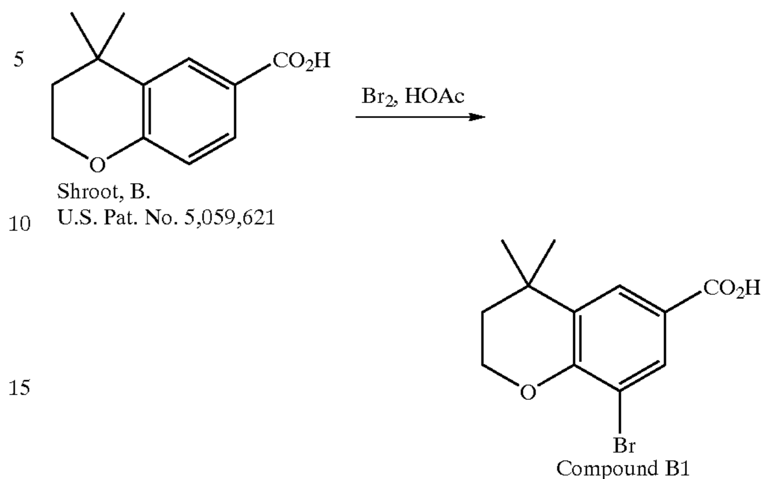
Reaction Scheme 5
