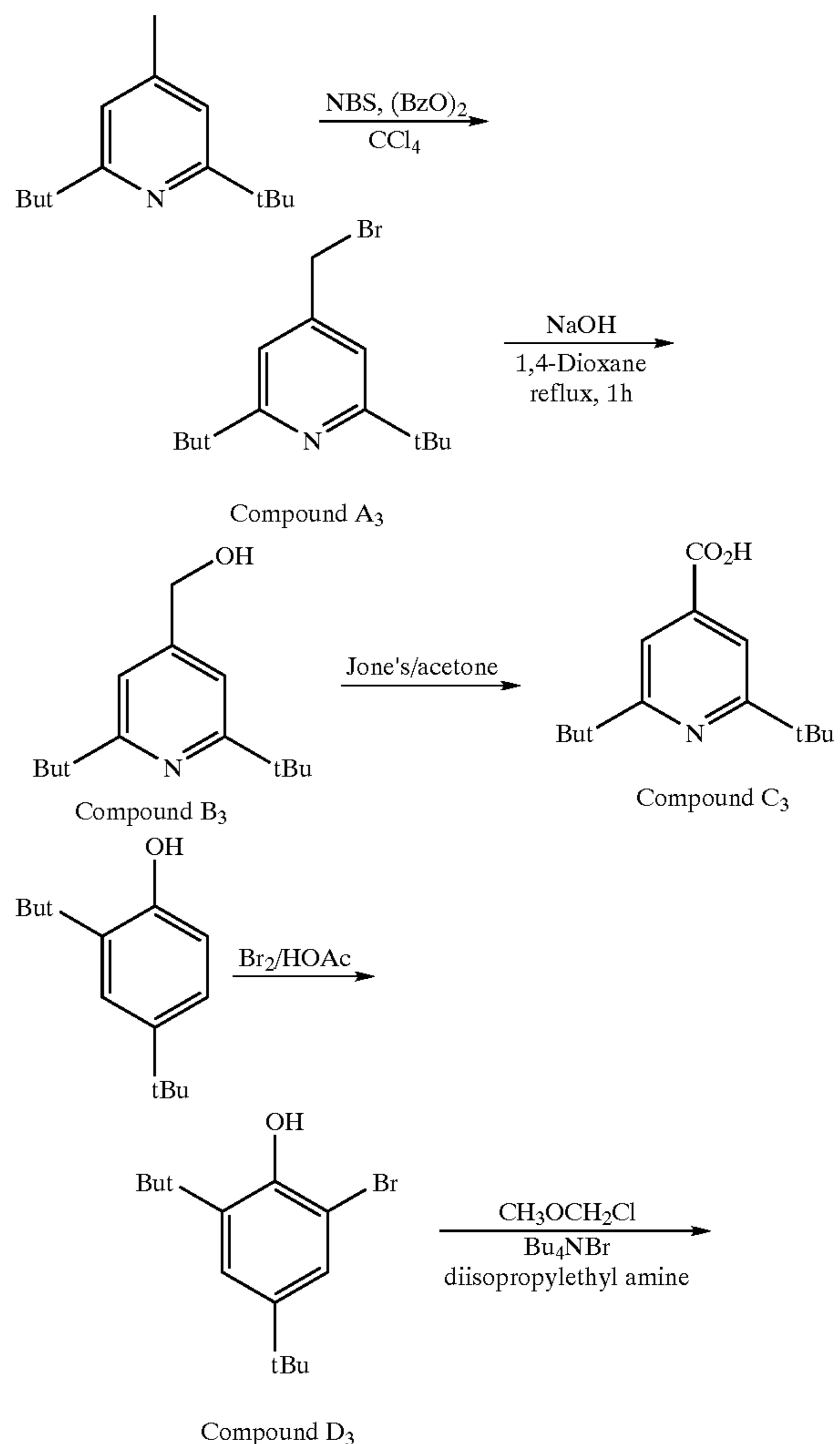
Reaction Scheme 13
