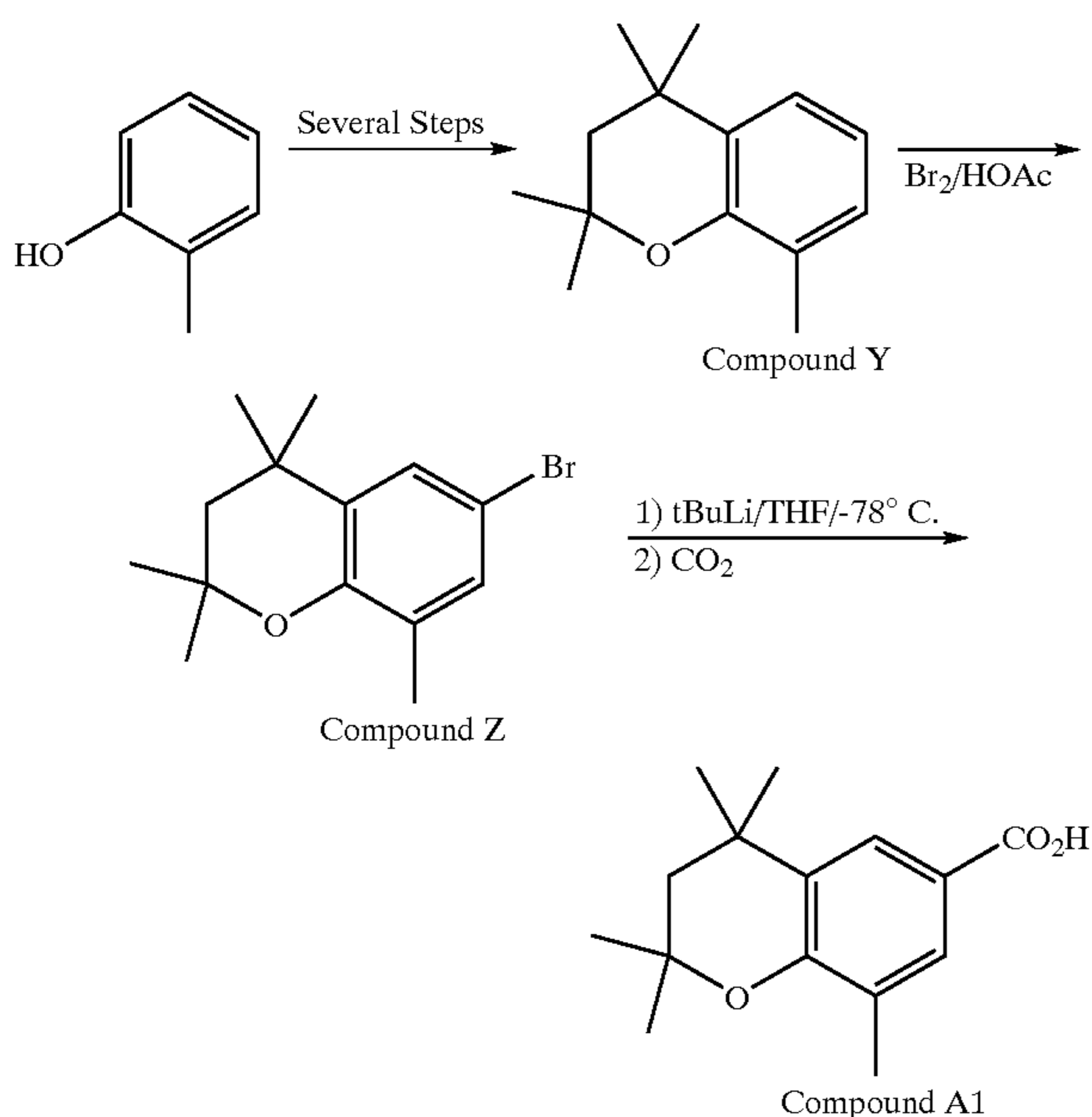
Reaction Scheme 4
