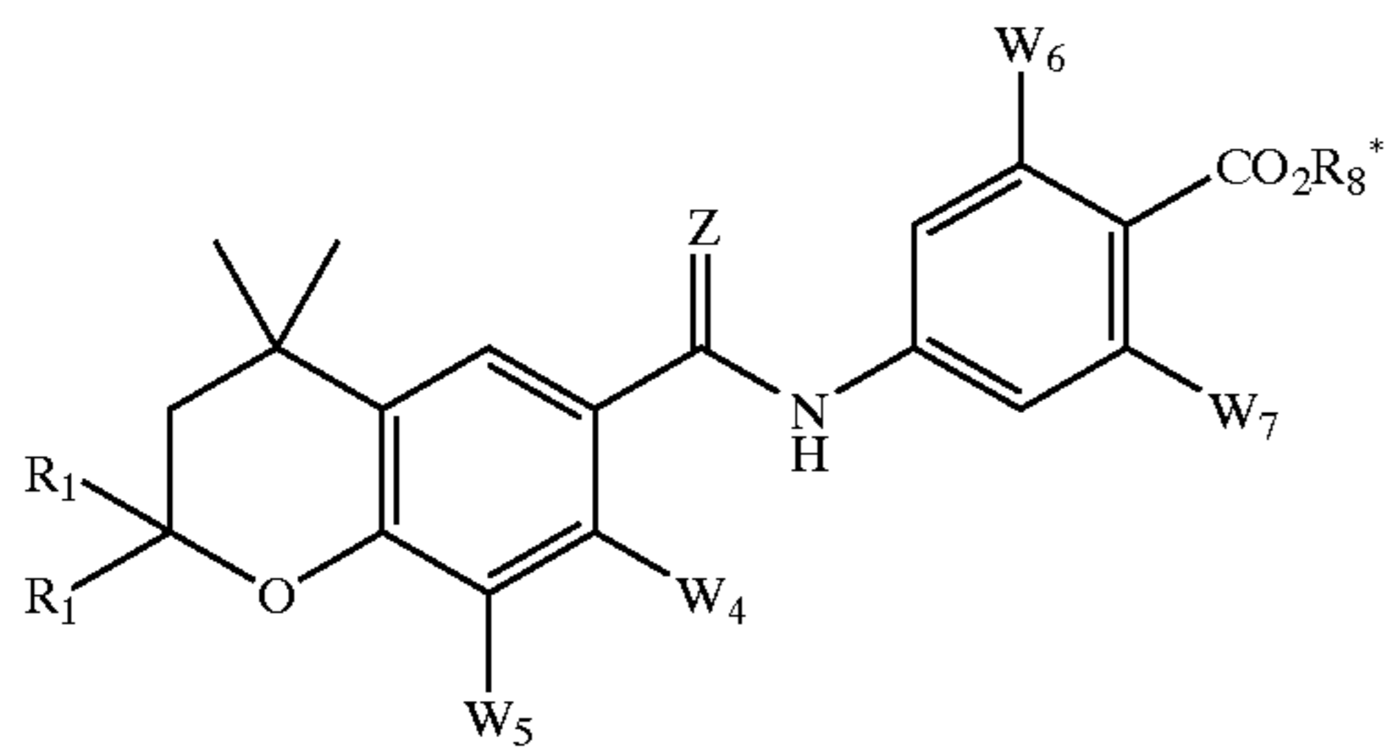
Formula 4
