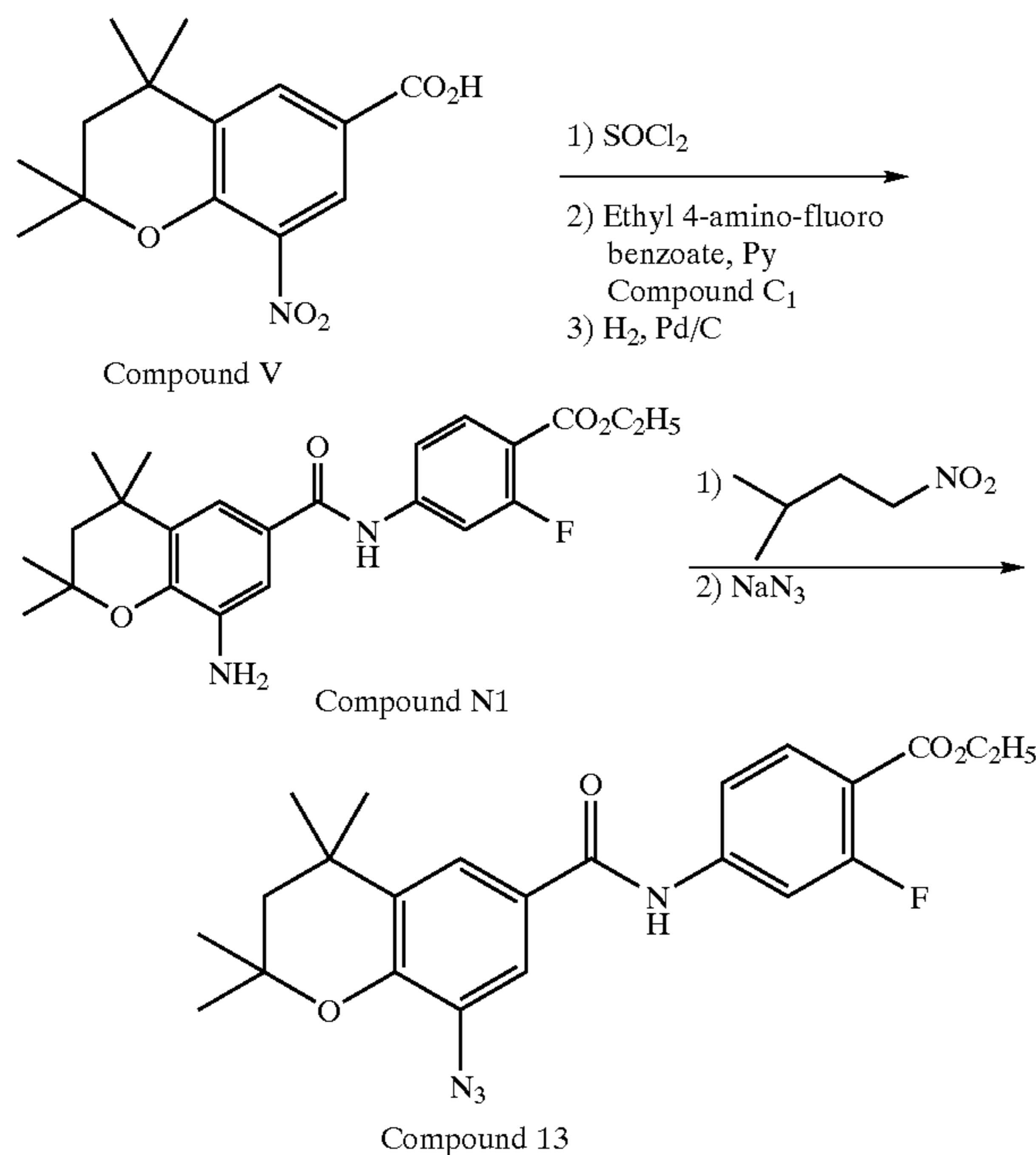
Reaction Scheme 10
