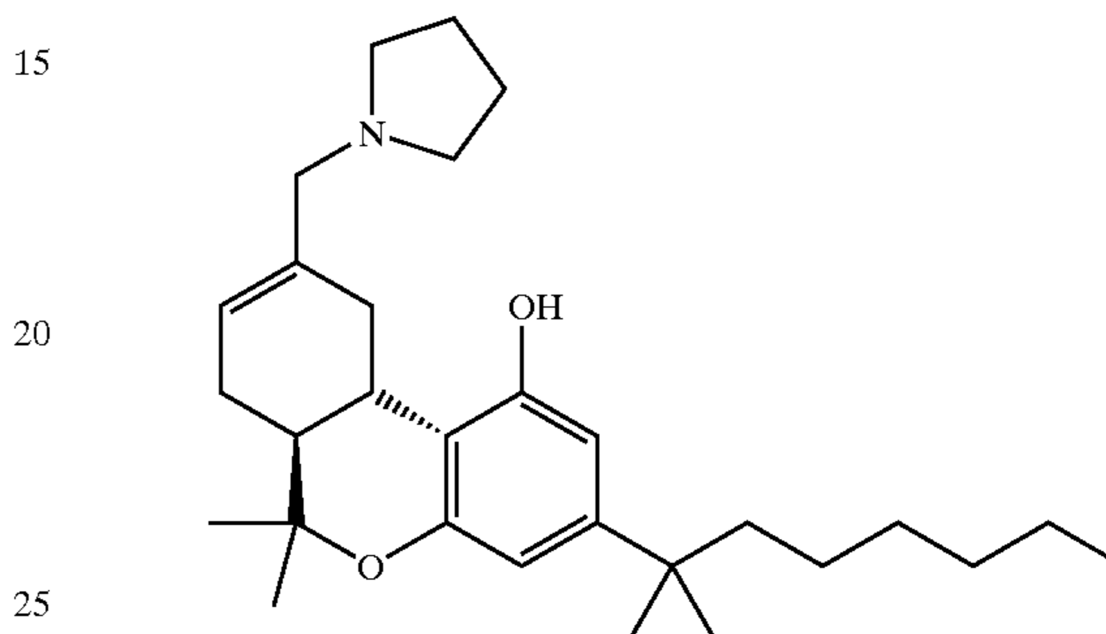
Compound 8
