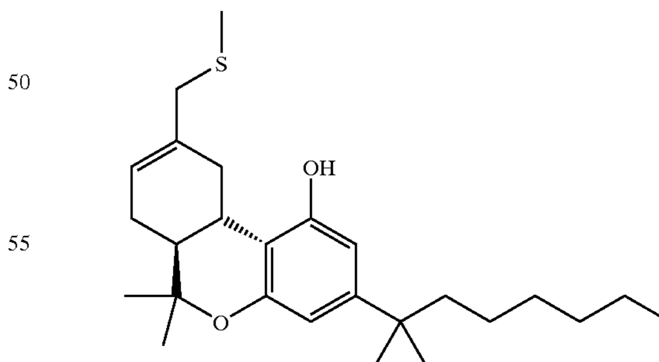
Compound 9
