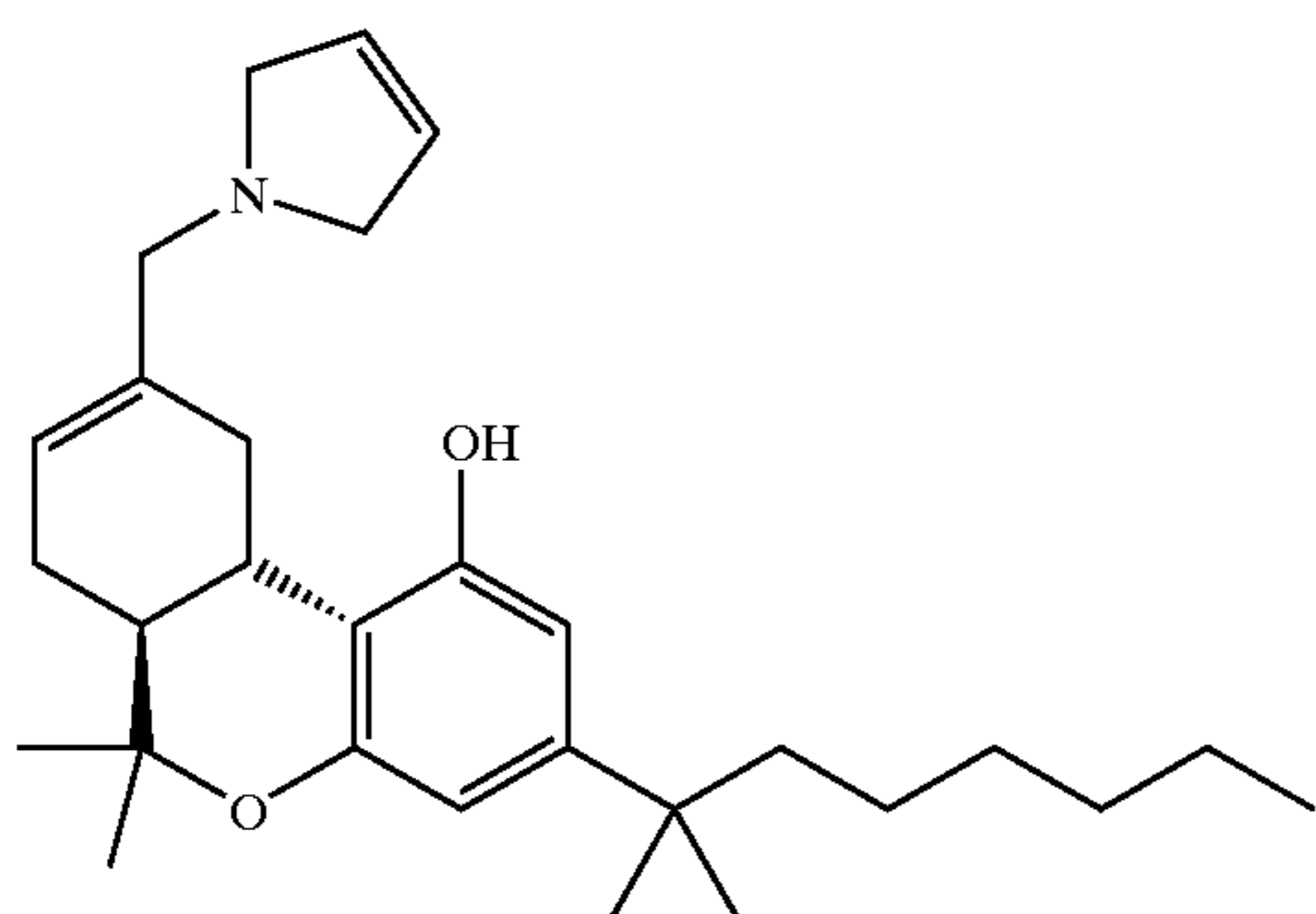
Compound 7
