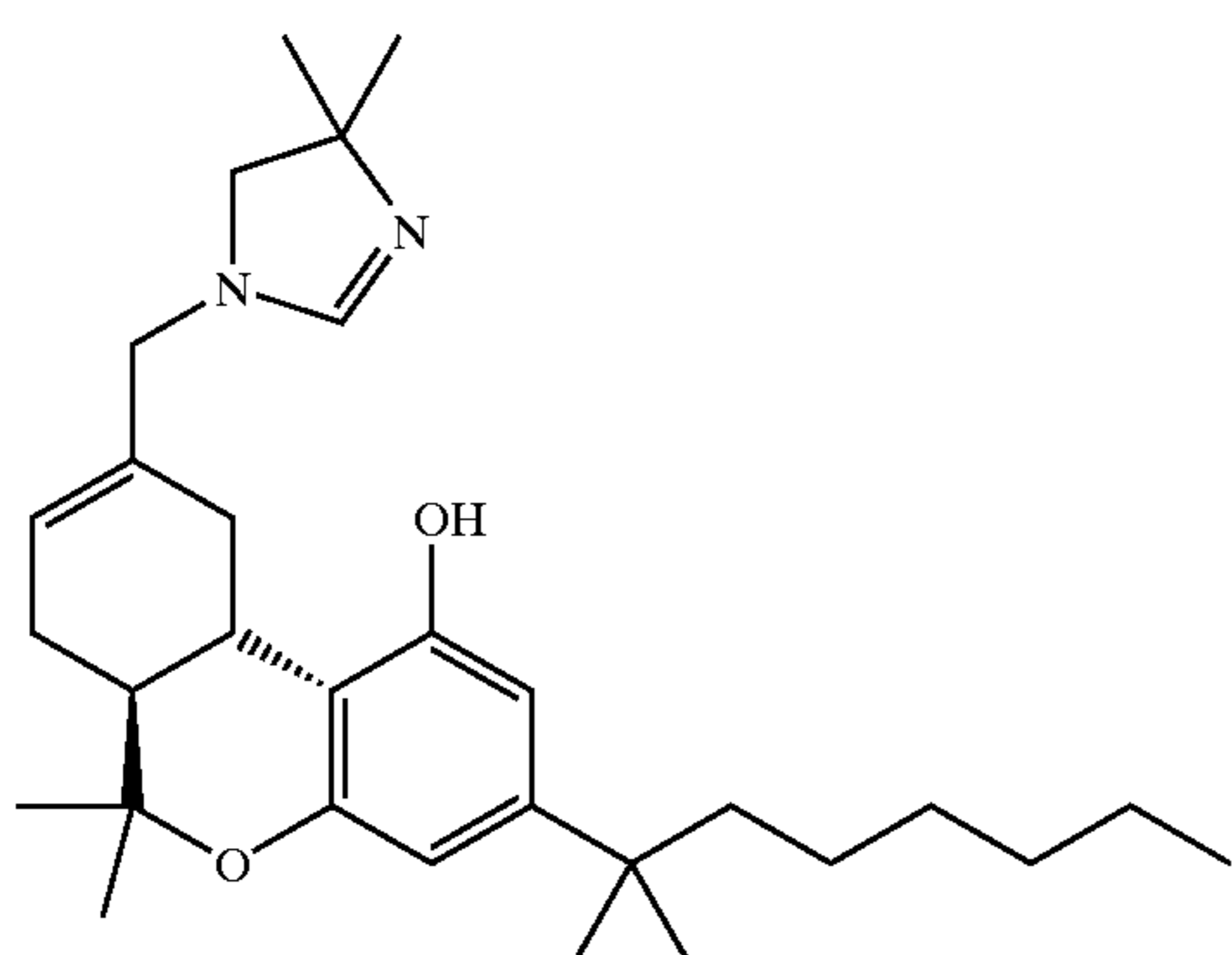
Compound 6
