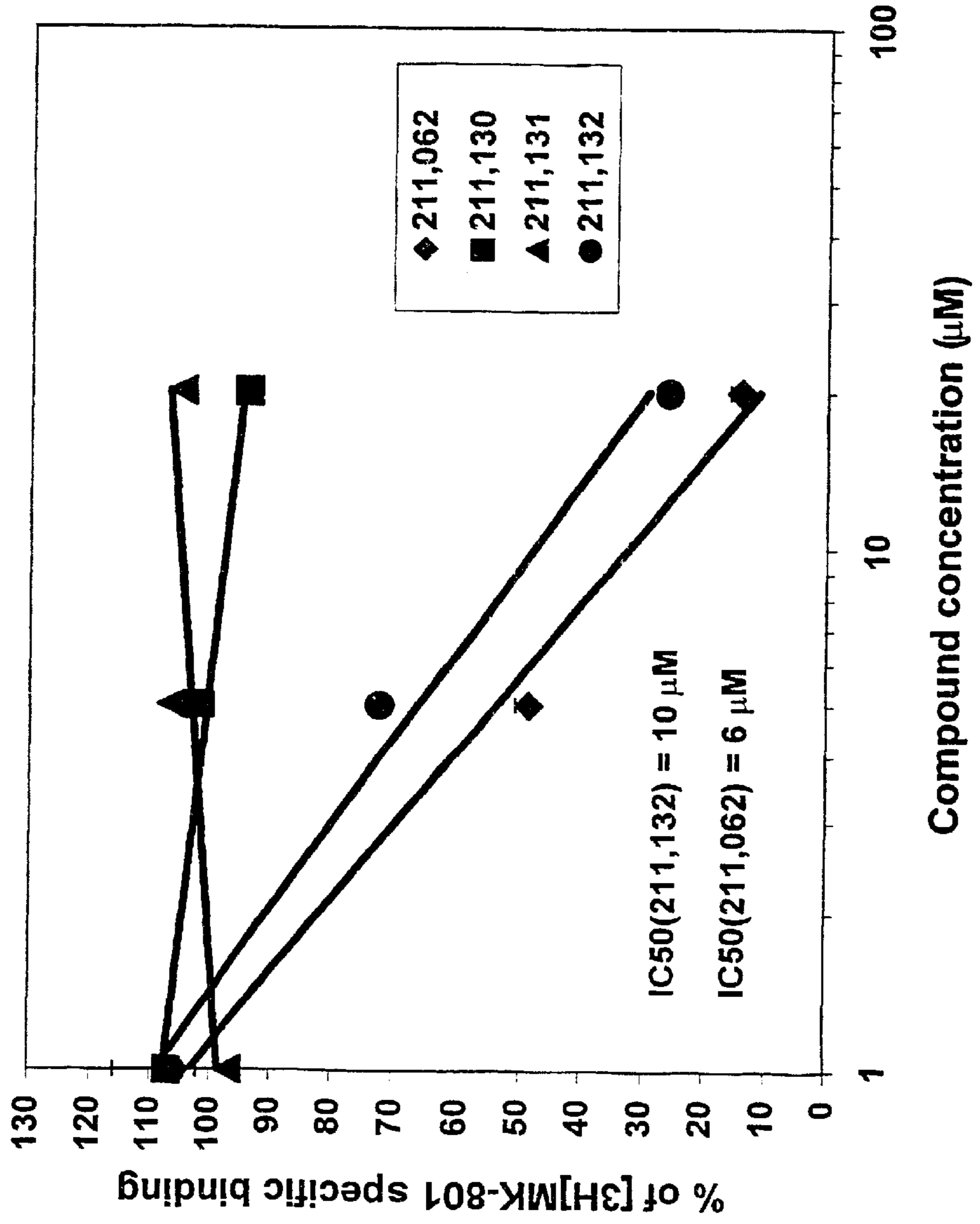
Figure 2 Displacement of [3H]MK-801 binding by Dexanabinol derivatives
