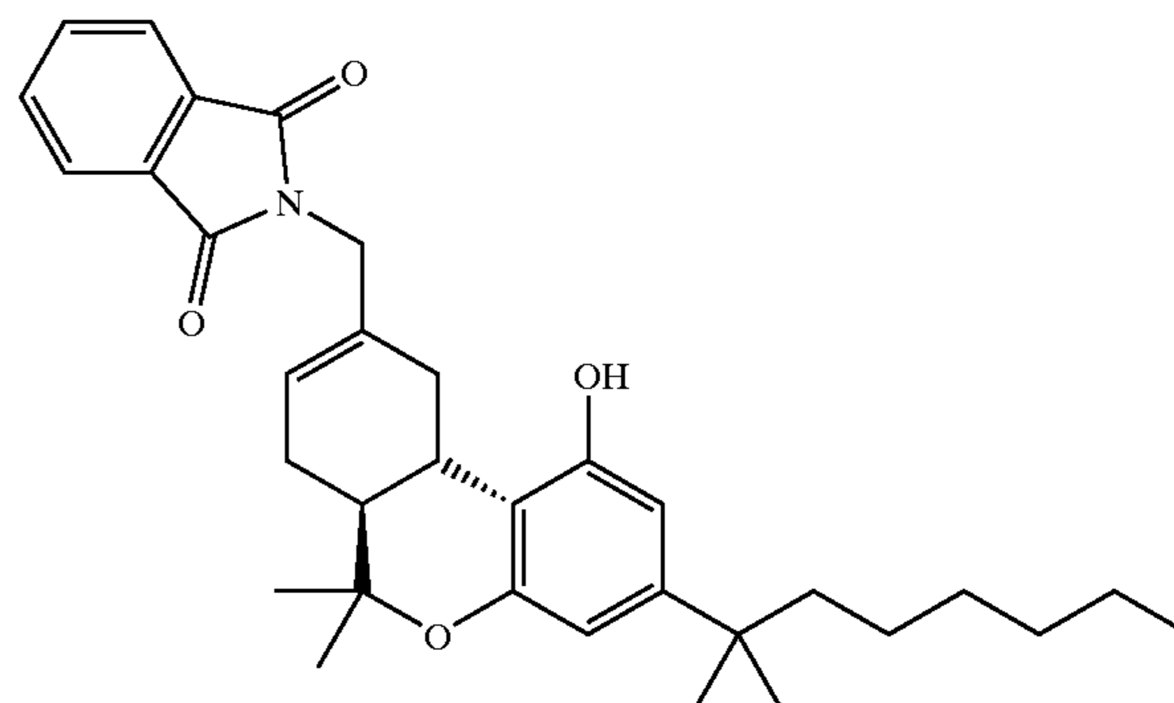
Compound 12
