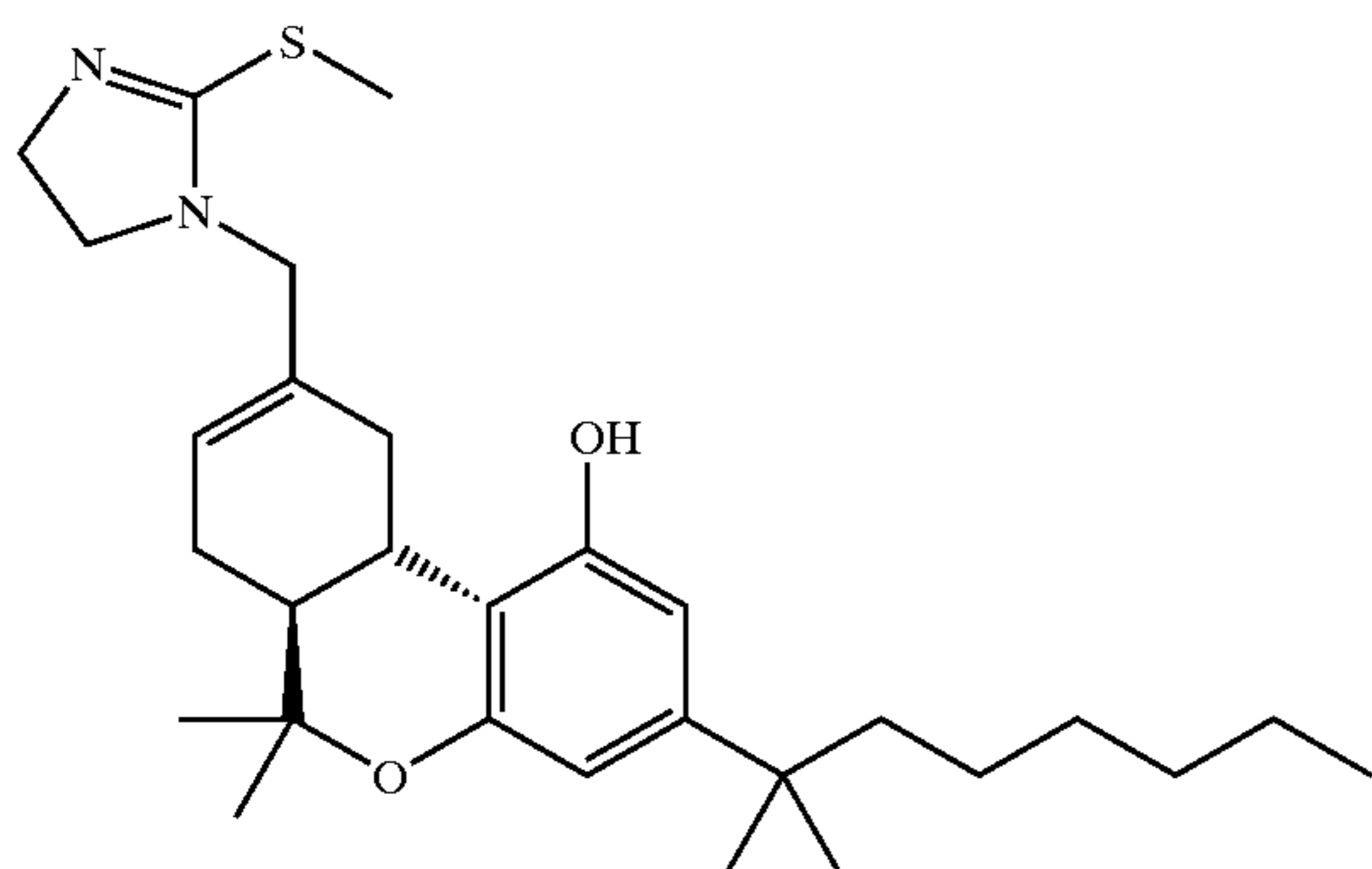
Compound 11
