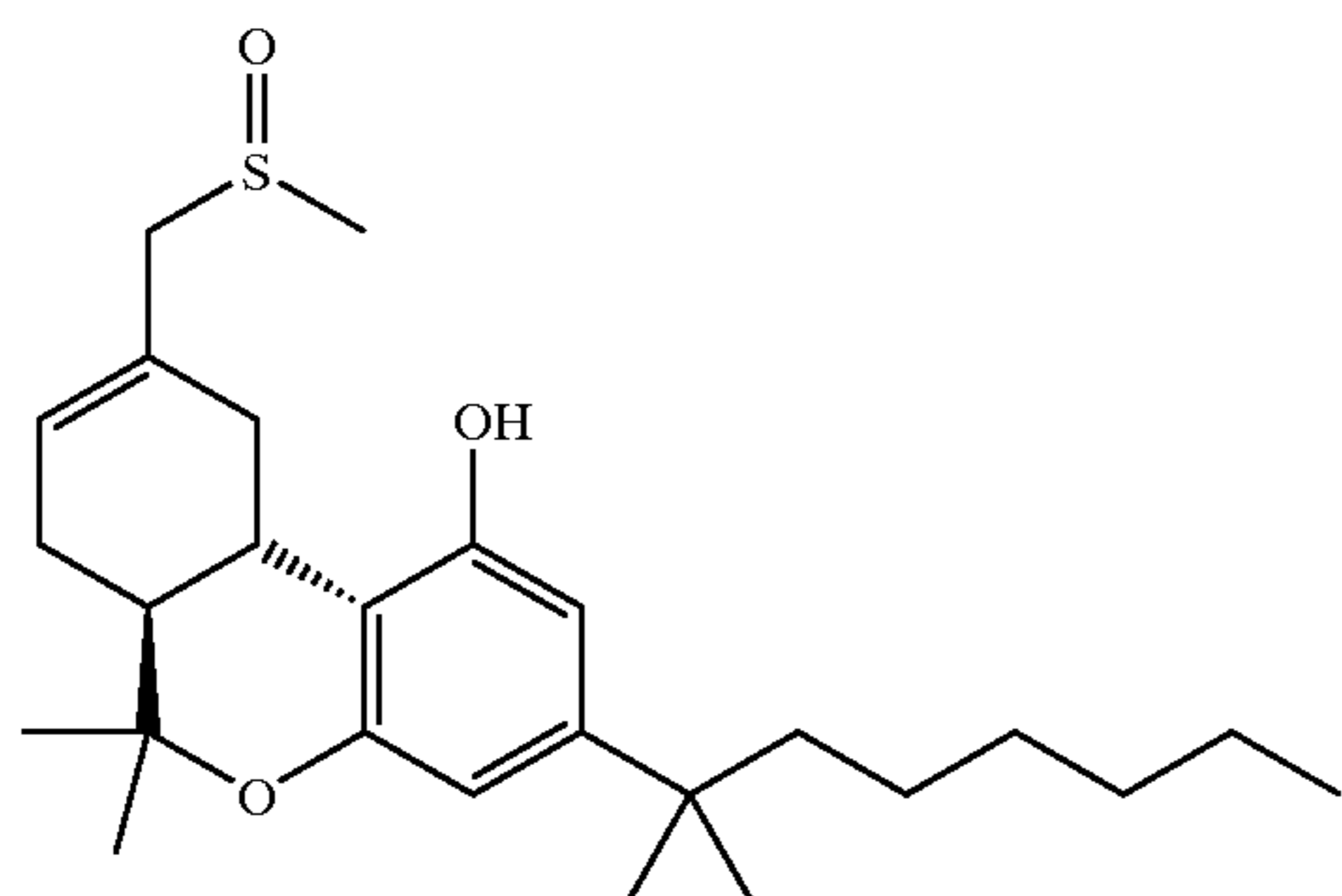
Compound 10
