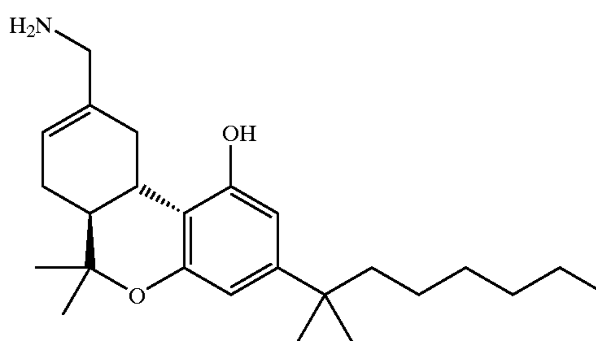
Compound 13
