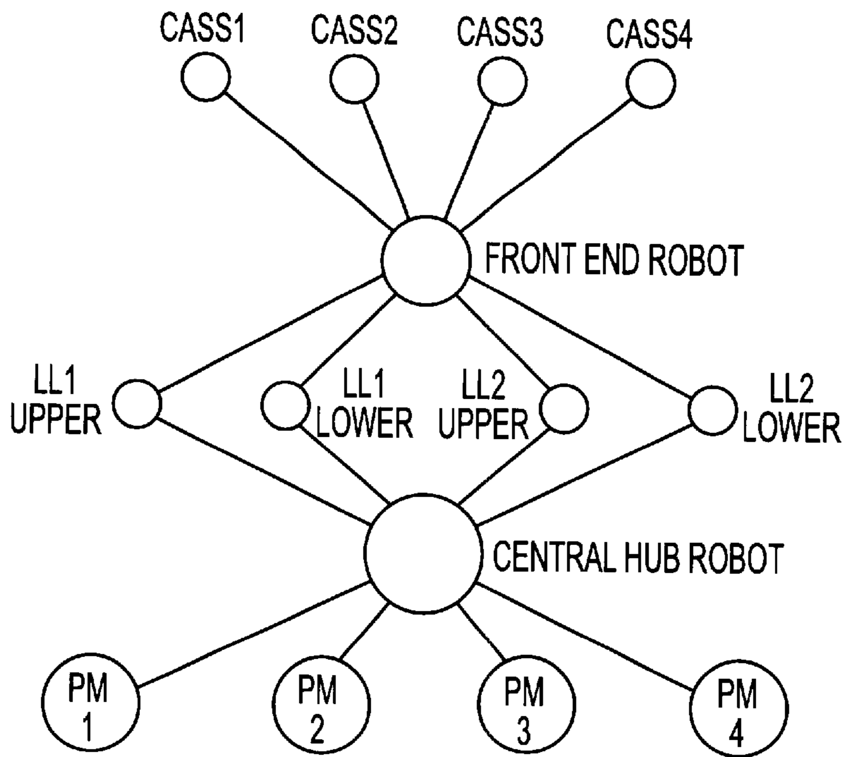
FIG. 4 (PRIOR ART)
