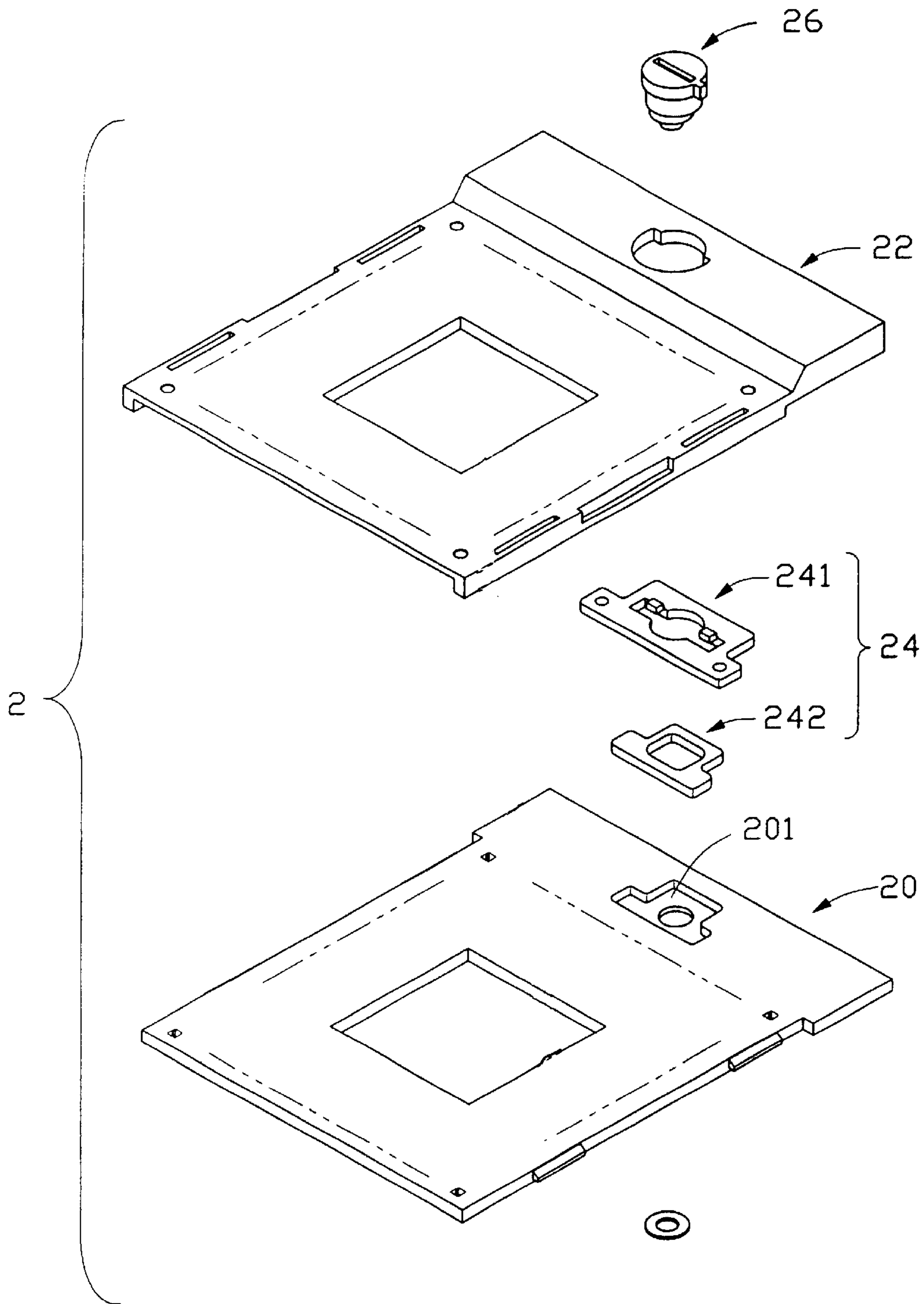
FIG. 5 (PRIOR ART)
