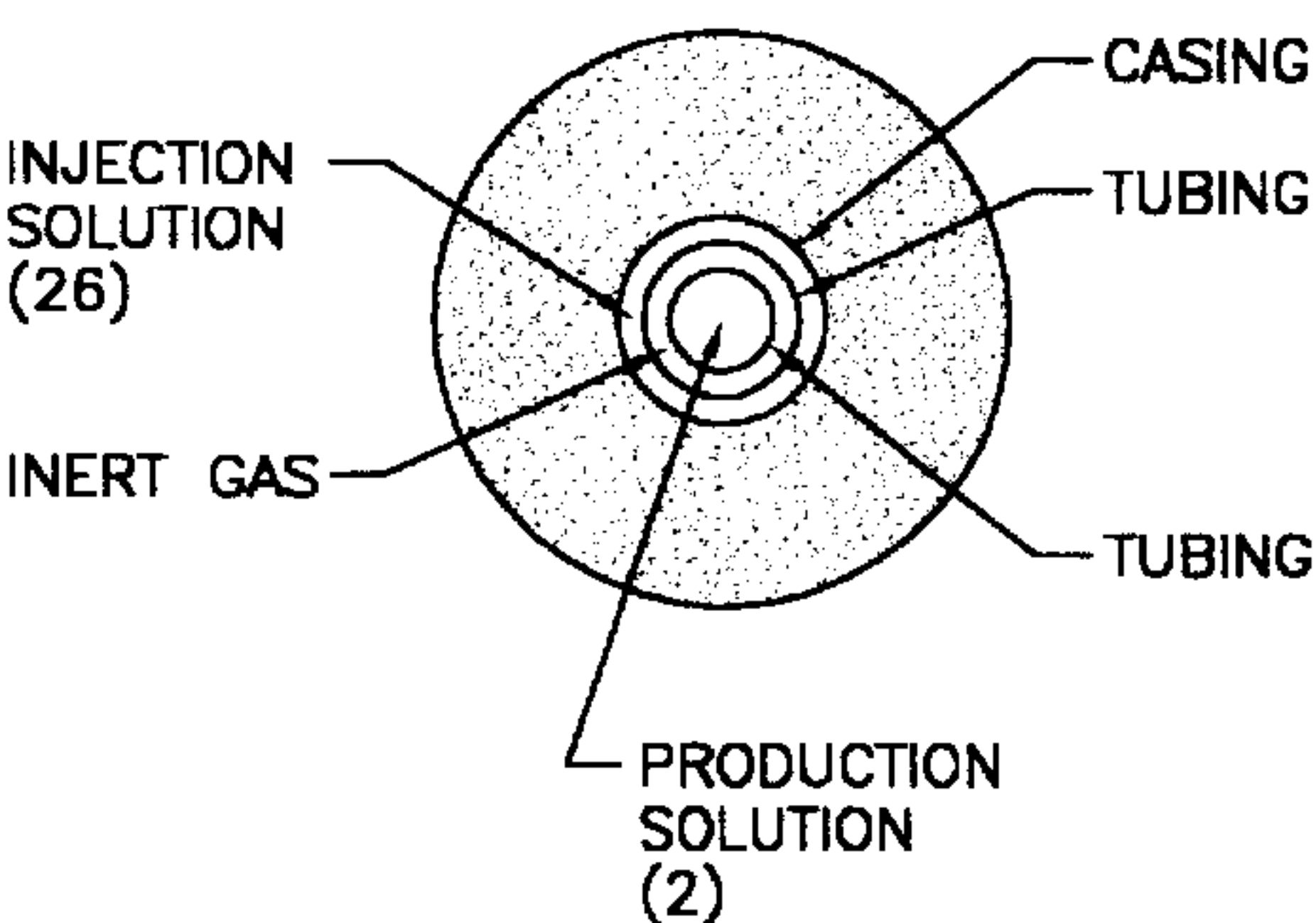
FIGURE 3B CROSS SECTION DETAIL A-A'
