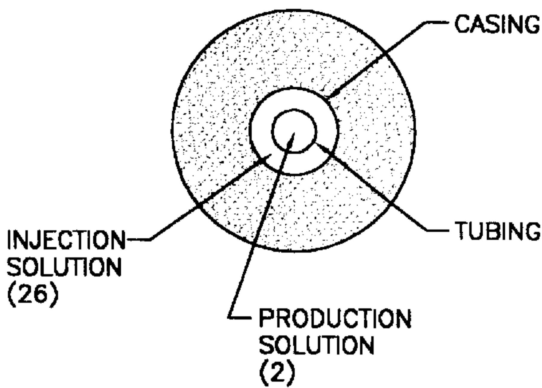
FIGURE 3A CROSS SECTION DETAIL A-A'
