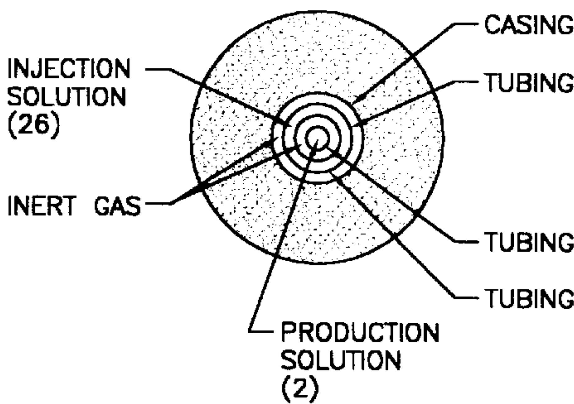
FIGURE 3C CROSS SECTION DETAIL A-A'
