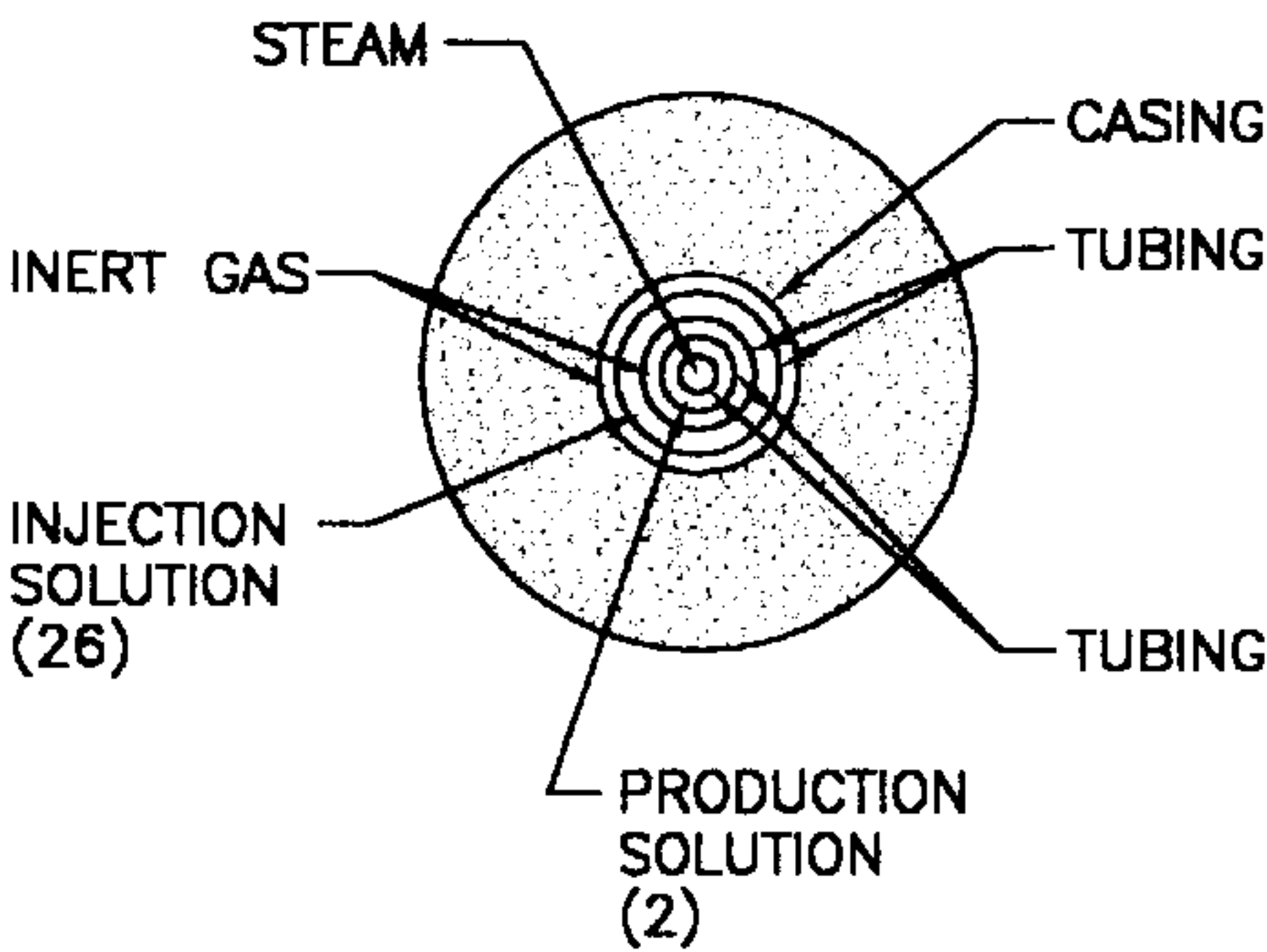
FIGURE 3D CROSS SECTION DETAIL A-A'
