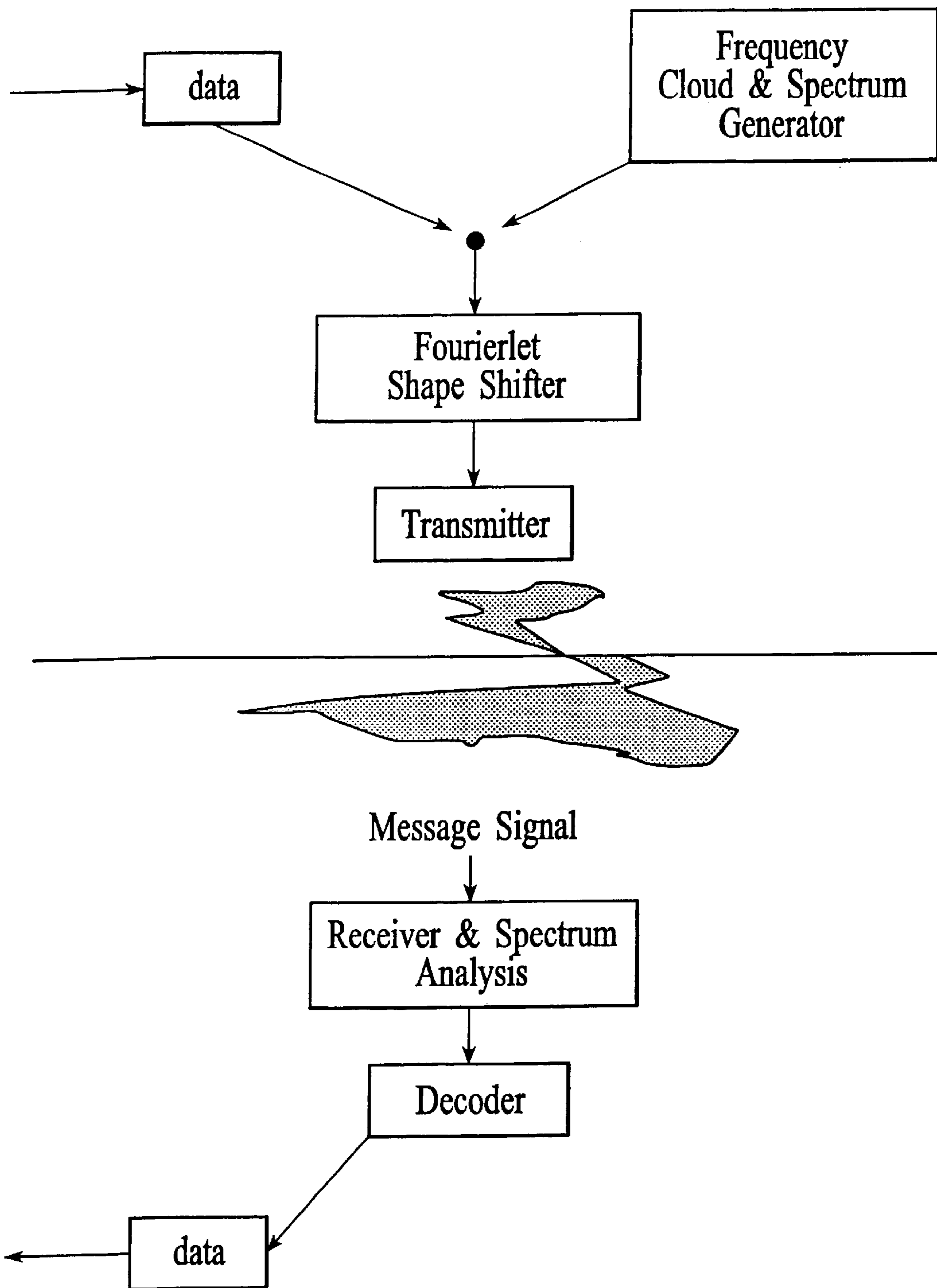
The Fourierlet Shape Shifter in System Context.
